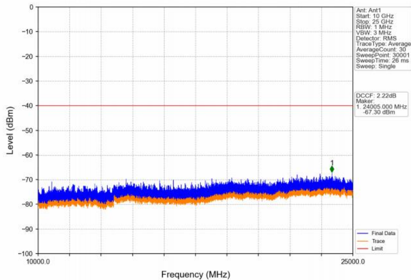
Band48_10MHz_64QAM_LCH_3555MHz_RB_1_0_NTNV
