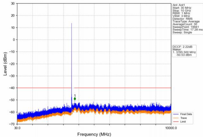
Band48_5MHz_16QAM_LCH_3552.5MHz_RB_1_0_NTNV
