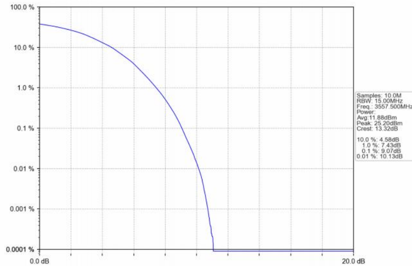
Band48_15MHz_64QAM_LCH_3557.5MHz_RB_75_0_NTNV
