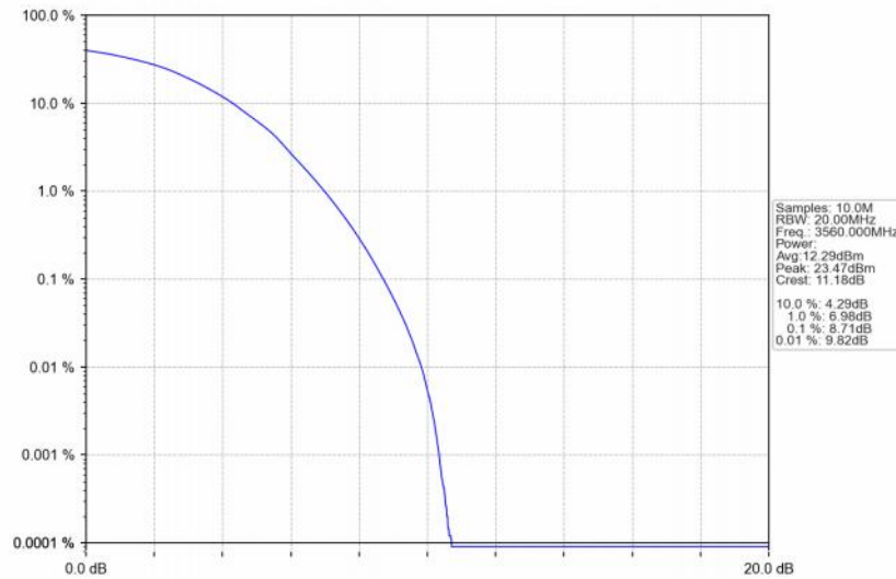
Band48_20MHz_64QAM_LCH_3560MHz_RB_100_0_NTNV
