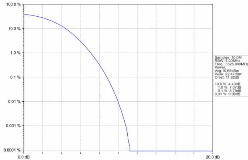
Band48_5MHz_256QAM_MCH_3625MHz_RB_25_0_NTNV
