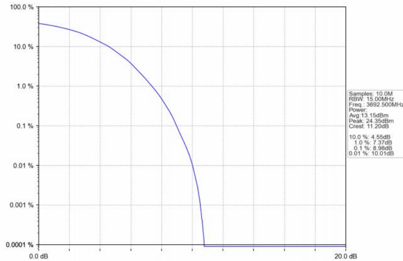
Band48_15MHz_64QAM_HCH_3692.5MHz_RB_75_0_NTNV
