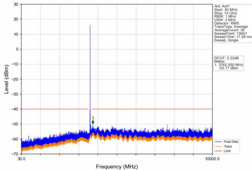
Band48_10MHz_16QAM_MCH_3625MHz_RB_1_0_NTNV
