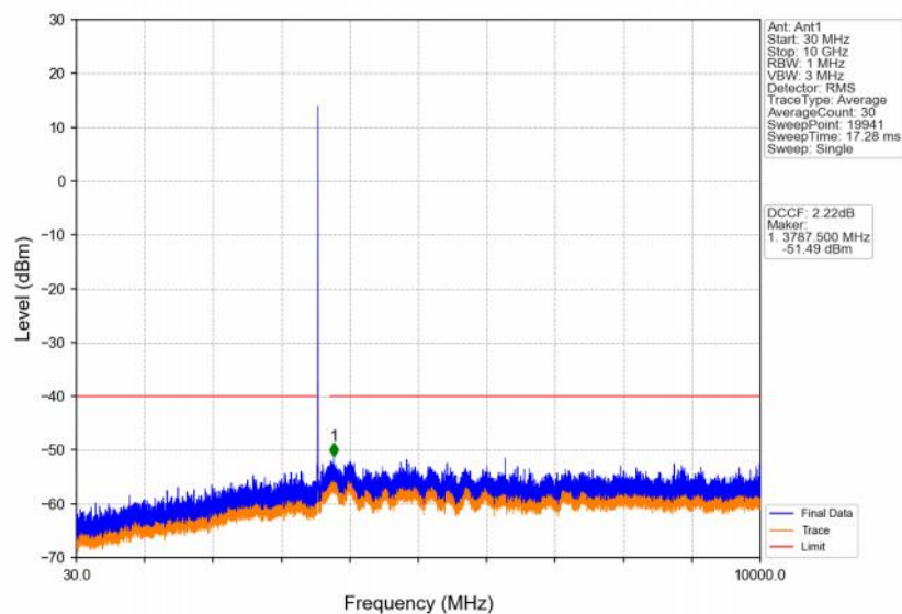
Band48_5MHz_64QAM_LCH_3552.5MHz_RB_1_0_NTNV
