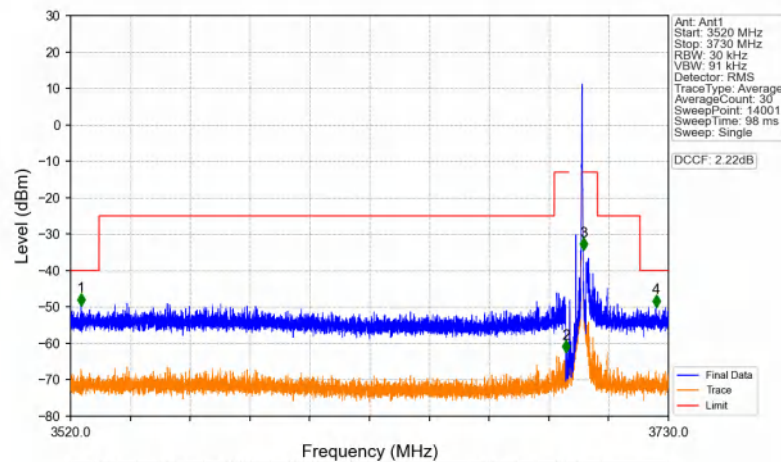
Band48_5MHz_64QAM_HCH_3697.5MHz_RB_1_24_NTNV
