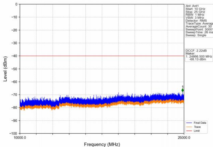
Band48_10MHz_16QAM_MCH_3625MHz_RB_1_0_NTNV
