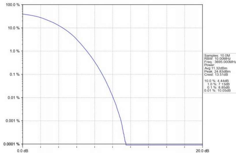
Band48_10MHz_256QAM_HCH_3695MHz_RB_50_0_NTNV
