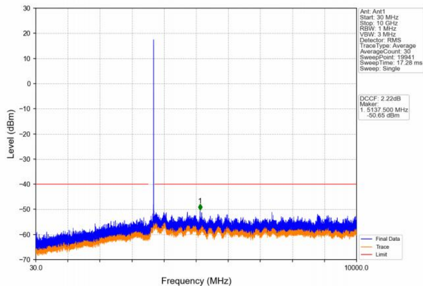
Band48_10MHz_16QAM_HCH_3695MHz_RB_1_0_NTNV
