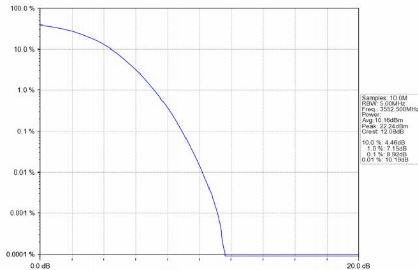
Band48_5MHz_256QAM_LCH_3552.5MHz_RB_25_0_NTNV
