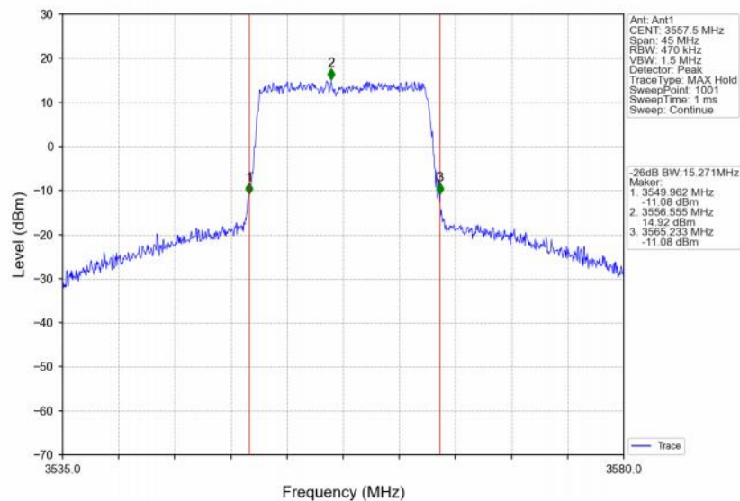
Band48_15MHz_16QAM_LCH_3557.5MHz_RB_75_0_NTNV
