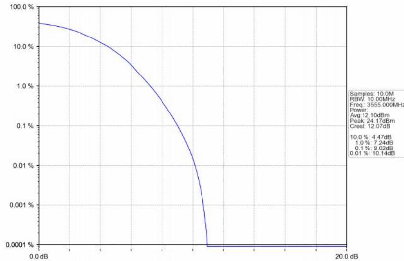
Band48_10MHz_64QAM_LCH_3555MHz_RB_50_0_NTNV
