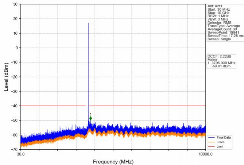
Band48_5MHz_QPSK_HCH_3697.5MHz_RB_1_0_NTNV
