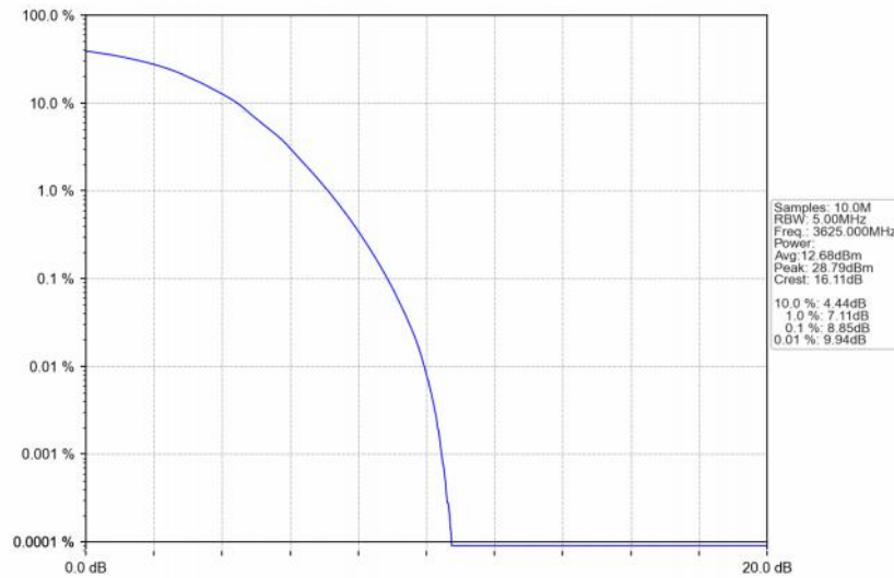
Band48_5MHz_16QAM_MCH_3625MHz_RB_25_0_NTNV
