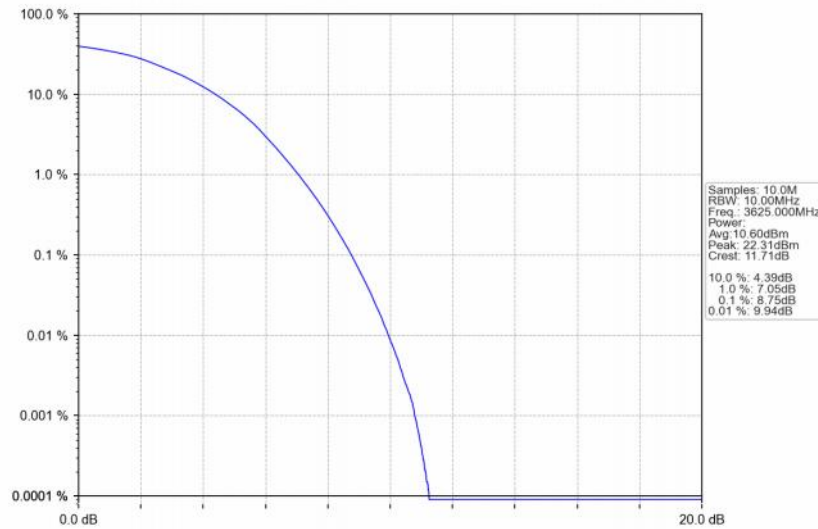
Band48_10MHz_256QAM_MCH_3625MHz_RB_50_0_NTNV
