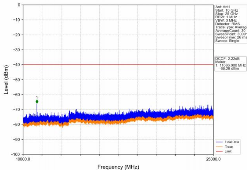
Band48_5MHz_64QAM_HCH_3697.5MHz_RB_1_0_NTNV
