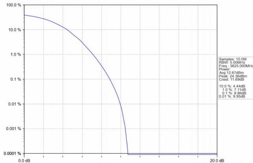
Band48_5MHz_64QAM_MCH_3625MHz_RB_25_0_NTNV
