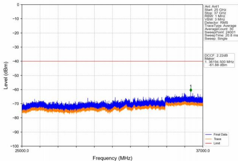
Band48_5MHz_QPSK_LCH_3552.5MHz_RB_1_0_NTNV
