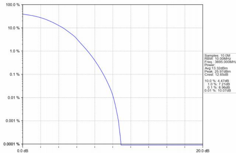
Band48_10MHz_16QAM_HCH_3695MHz_RB_50_0_NTNV
