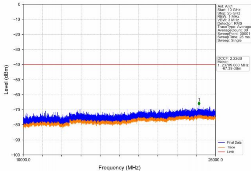
Band48_5MHz_64QAM_MCH_3625MHz_RB_1_0_NTNV
