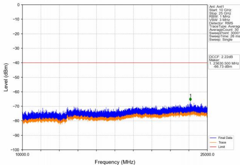
Band48_5MHz_16QAM_MCH_3625MHz_RB_1_0_NTNV
