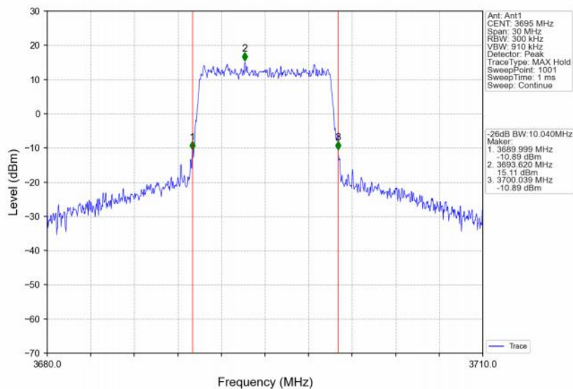
Band48_10MHz_16QAM_HCH_3695MHz_RB_50_0_NTNV
