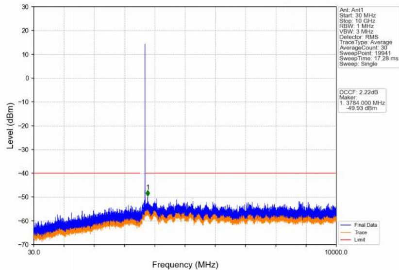
Band48_5MHz_64QAM_HCH_3697.5MHz_RB_1_0_NTNV
