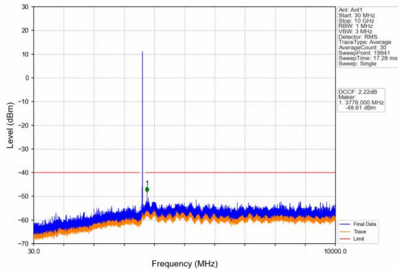
Band48_5MHz_256QAM_MCH_3625MHz_RB_1_0_NTNV
