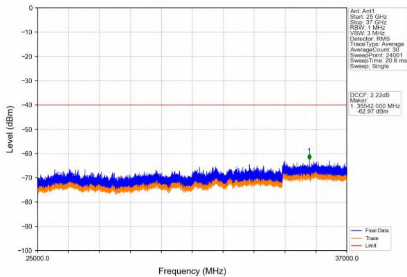
Band48_5MHz_16QAM_HCH_3697.5MHz_RB_1_0_NTNV
