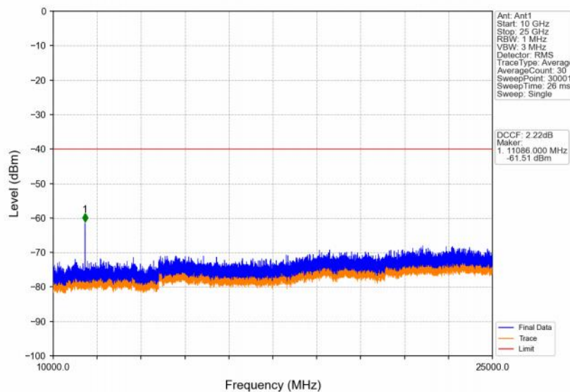
Band48_5MHz_QPSK_HCH_3697.5MHz_RB_1_0_NTNV
