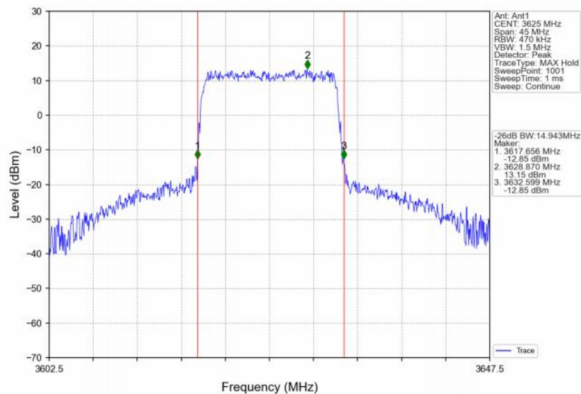
Band48_15MHz_64QAM_MCH_3625MHz_RB_75_0_NTNV
