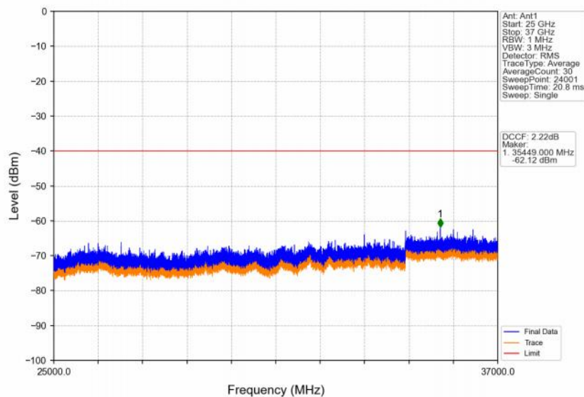
Band48_5MHz_64QAM_MCH_3625MHz_RB_1_0_NTNV
