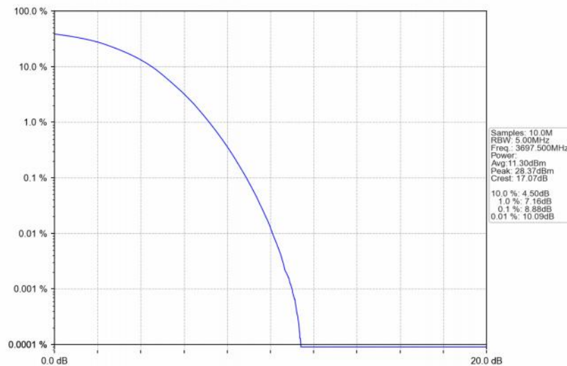
Band48_5MHz_256QAM_HCH_3697.5MHz_RB_25_0_NTNV
