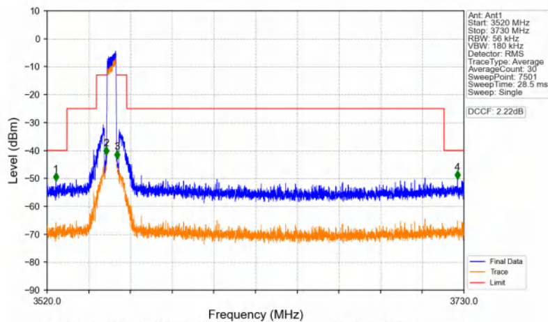
Band48_5MHz_256QAM_LCH_3552.5MHz_RB_25_0_NTNV
