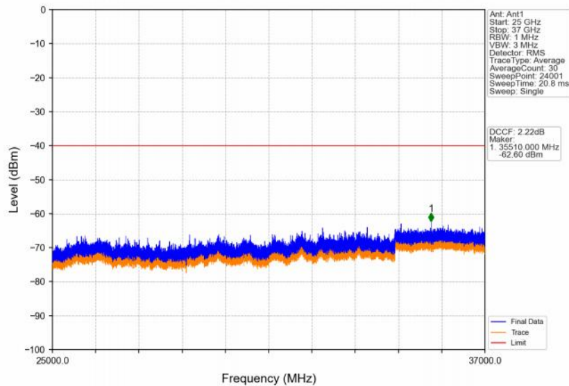
Band48_5MHz_64QAM_HCH_3697.5MHz_RB_1_24_NTNV
