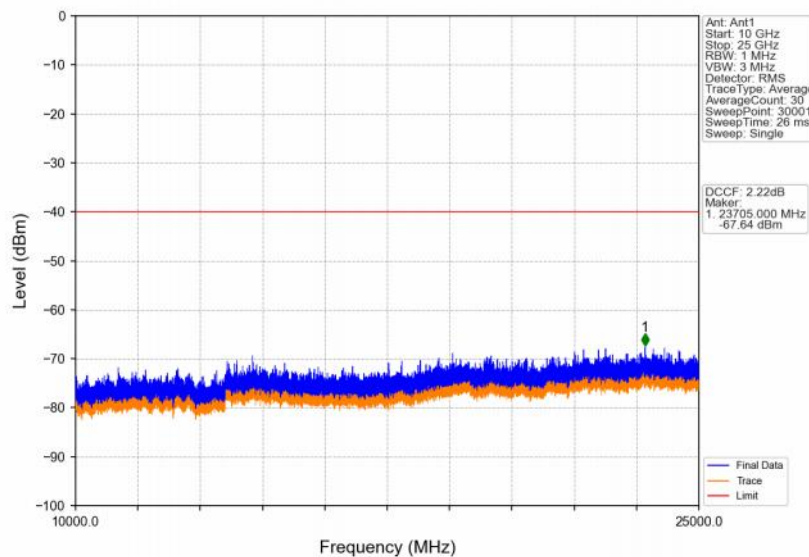
Band48_5MHz_256QAM_MCH_3625MHz_RB_1_0_NTNV
