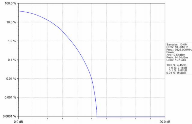
Band48_10MHz_16QAM_MCH_3625MHz_RB_50_0_NTNV
