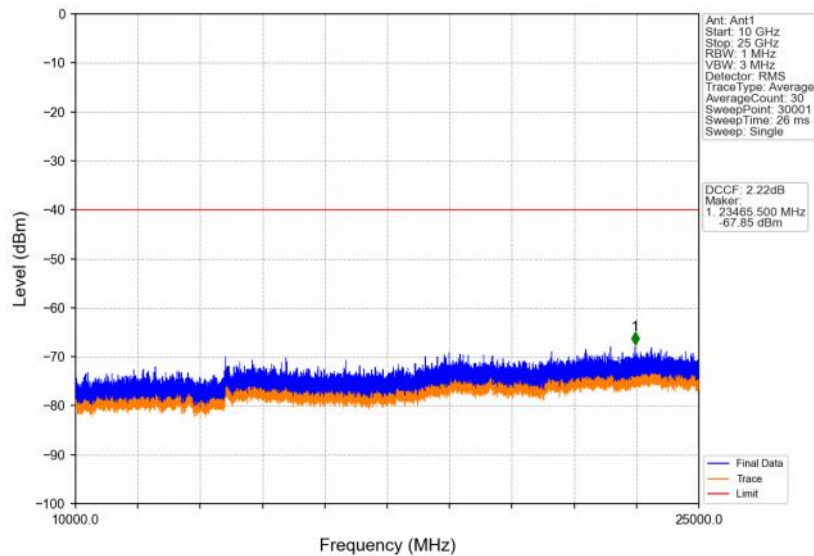
Band48_5MHz_QPSK_MCH_3625MHz_RB_1_0_NTNV
