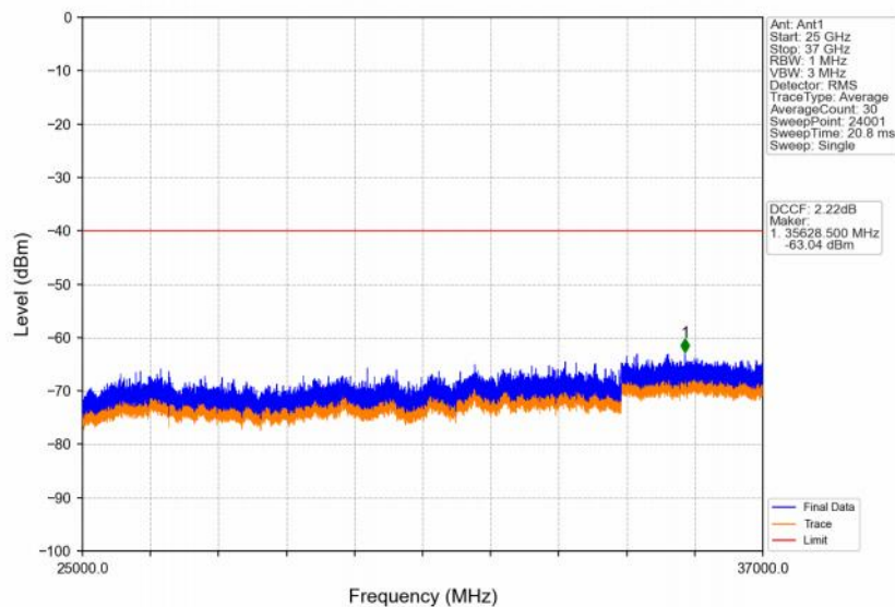
Band48_10MHz_16QAM_HCH_3695MHz_RB_1_0_NTNV
