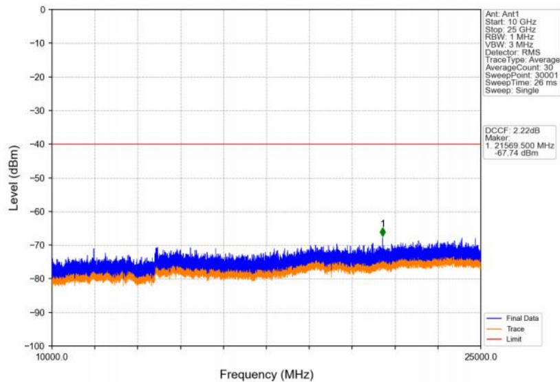
Band48_5MHz_QPSK_LCH_3552.5MHz_RB_1_0_NTNV
