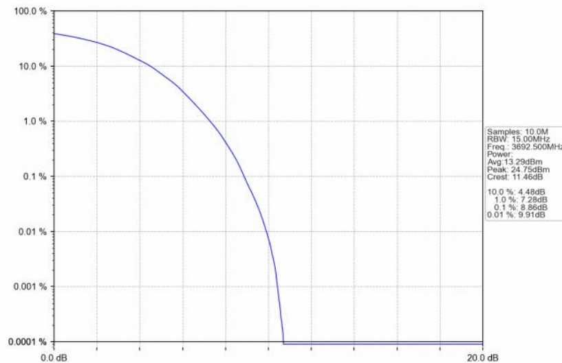
Band48_15MHz_16QAM_HCH_3692.5MHz_RB_75_0_NTNV
