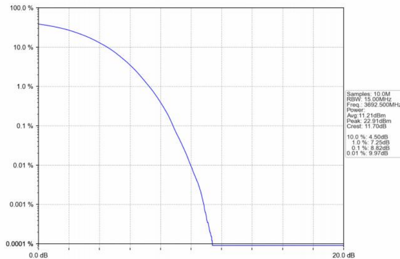
Band48_15MHz_256QAM_HCH_3692.5MHz_RB_75_0_NTNV
