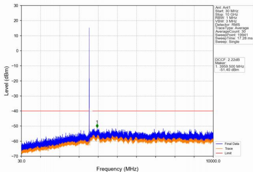
Band48_10MHz_64QAM_LCH_3555MHz_RB_1_0_NTNV
