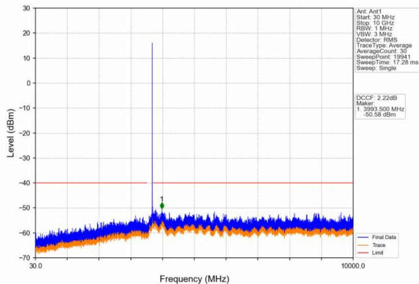
Band48_5MHz_16QAM_HCH_3697.5MHz_RB_1_0_NTNV
