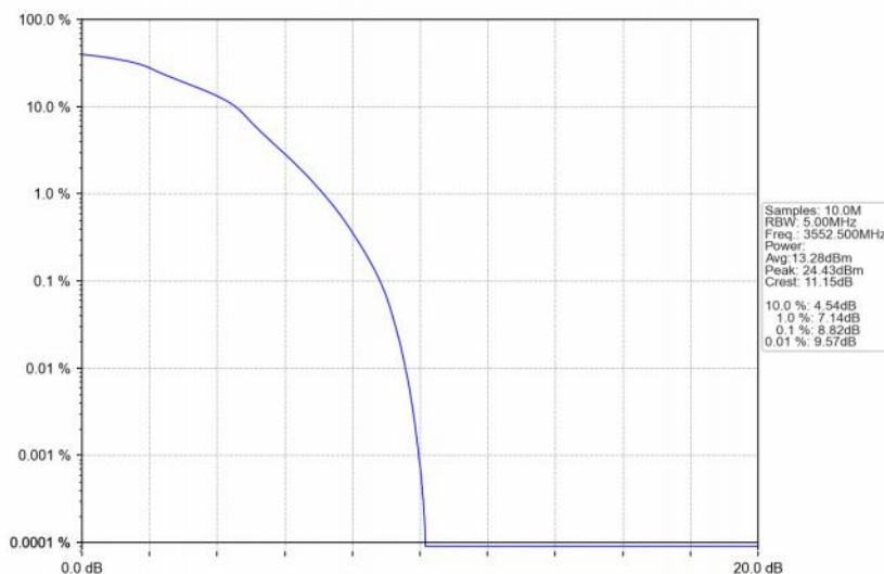
Band48_5MHz_16QAM_LCH_3552.5MHz_RB_25_0_NTNV
