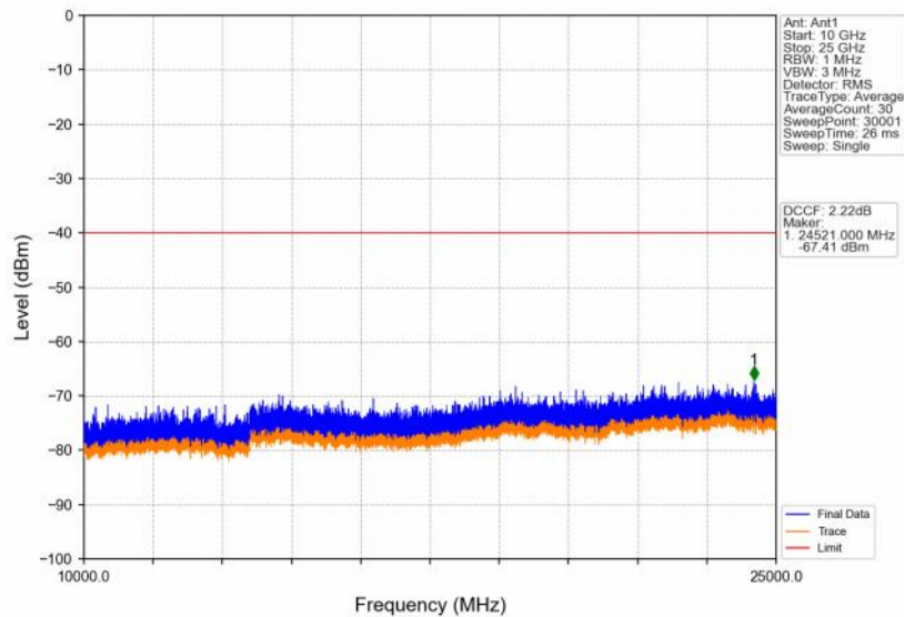
Band48_5MHz_256QAM_HCH_3697.5MHz_RB_1_0_NTNV
