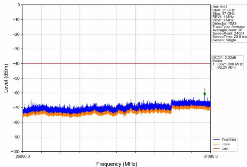
Band48_5MHz_QPSK_MCH_3625MHz_RB_1_0_NTNV
