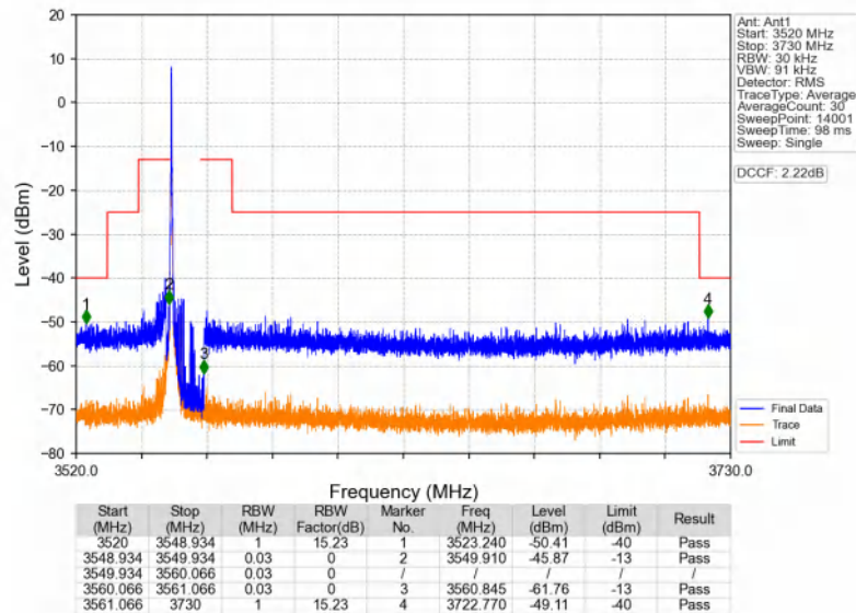
Band48_10MHz_64QAM_LCH_3555MHz_RB_1_0_NTNV
