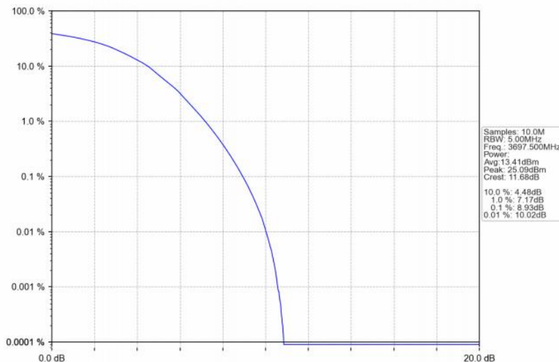
Band48_5MHz_QPSK_HCH_3697.5MHz_RB_25_0_NTNV
