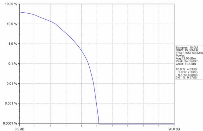
Band48_15MHz_16QAM_LCH_3557.5MHz_RB_75_0_NTNV
