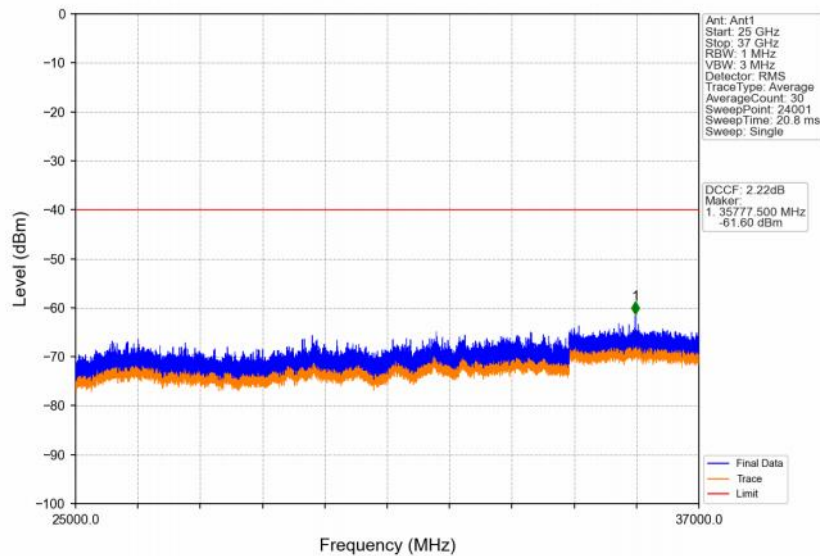
Band48_5MHz_256QAM_HCH_3697.5MHz_RB_1_0_NTNV
