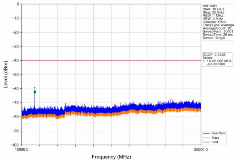
Band48_5MHz_16QAM_HCH_3697.5MHz_RB_1_0_NTNV
