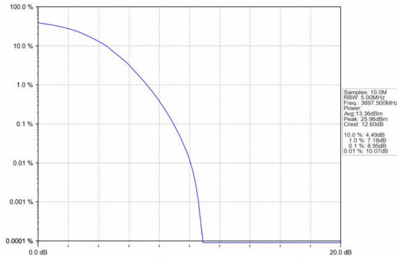
Band48_5MHz_64QAM_HCH_3697.5MHz_RB_25_0_NTNV
