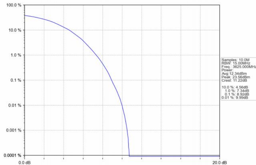
Band48_15MHz_64QAM_MCH_3625MHz_RB_75_0_NTNV
