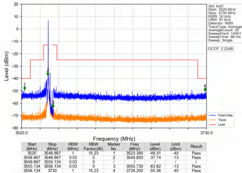
Band48_5MHz_64QAM_LCH_3552.5MHz_RB_1_0_NTNV
