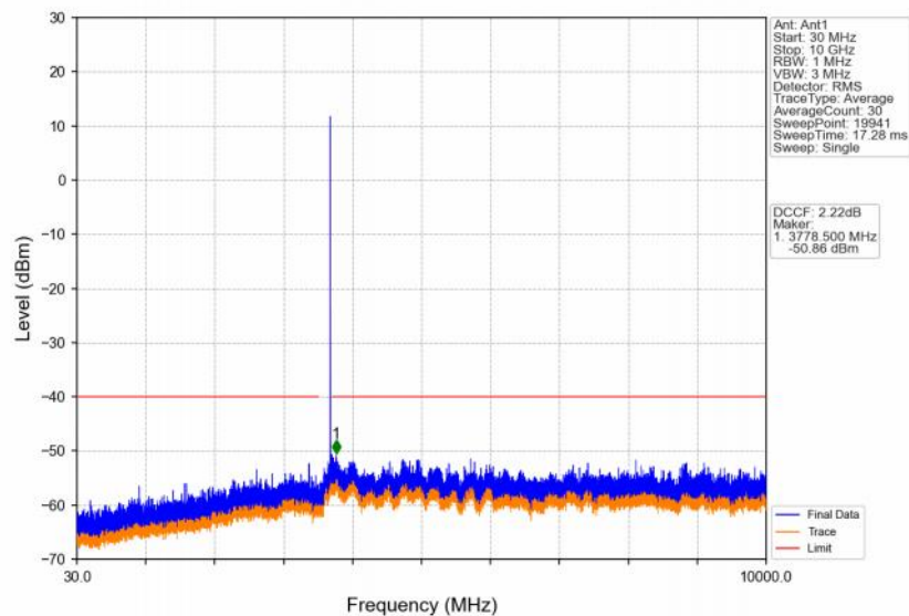
Band48_5MHz_256QAM_HCH_3697.5MHz_RB_1_0_NTNV
