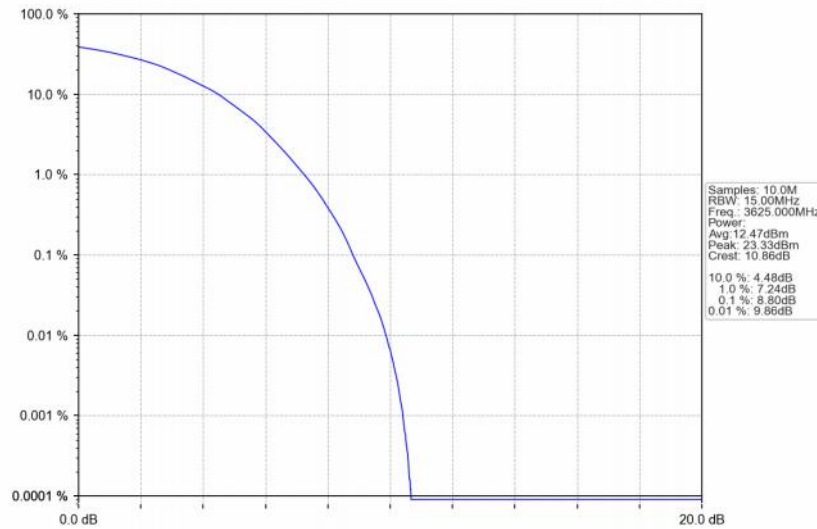
Band48_15MHz_16QAM_MCH_3625MHz_RB_75_0_NTNV
