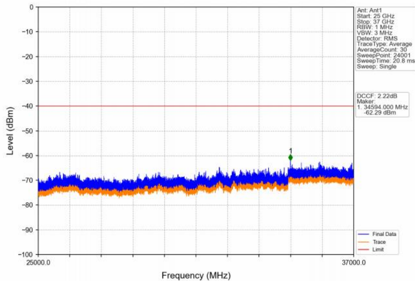
Band48_5MHz_16QAM_HCH_3697.5MHz_RB_1_0_NTNV
