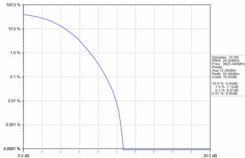
Band48_20MHz_64QAM_MCH_3625MHz_RB_100_0_NTNV
