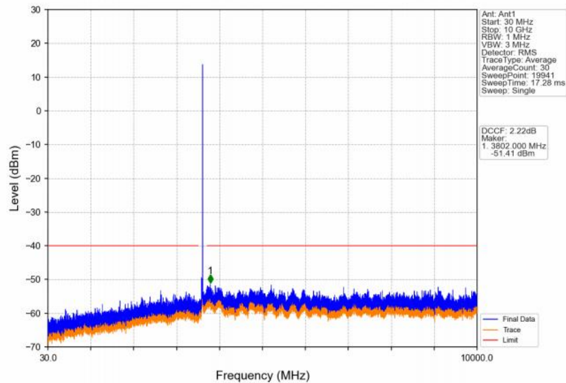
Band48_5MHz_16QAM_MCH_3625MHz_RB_1_0_NTNV
