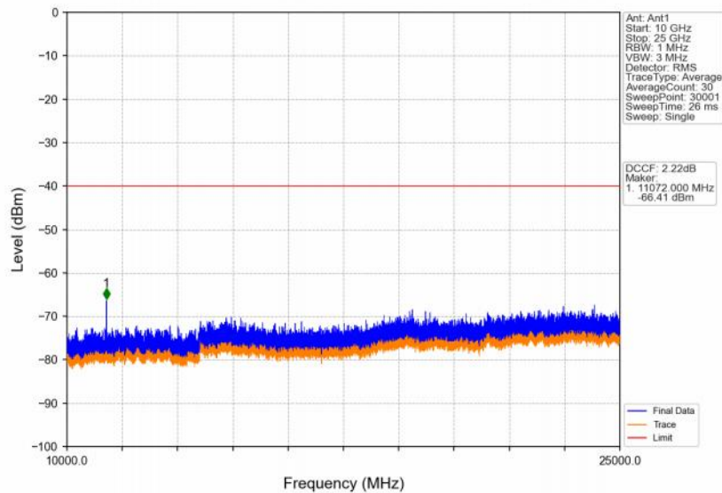
Band48_10MHz_16QAM_HCH_3695MHz_RB_1_0_NTNV
