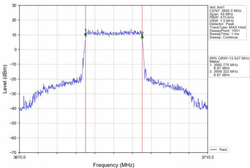
Band48_15MHz_256QAM_HCH_3692.5MHz_RB_75_0_NTNV
