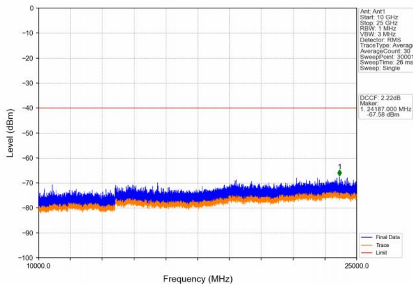
Band48_5MHz_16QAM_LCH_3552.5MHz_RB_1_0_NTNV
