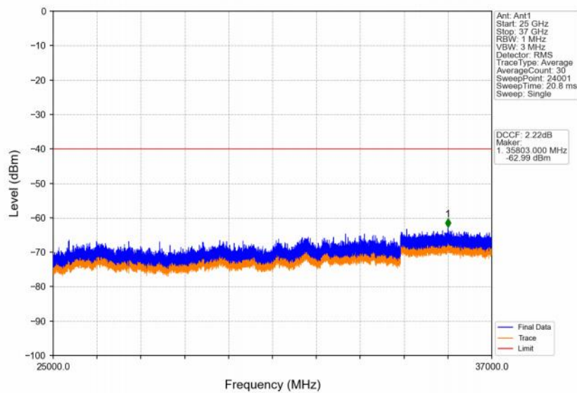
Band48_5MHz_256QAM_HCH_3697.5MHz_RB_1_0_NTNV
