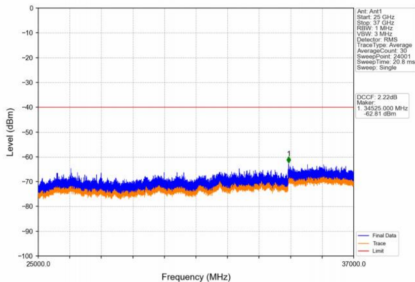
Band48_10MHz_64QAM_LCH_3555MHz_RB_1_0_NTNV
