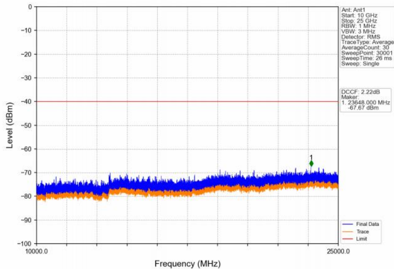
Band48_5MHz_64QAM_LCH_3552.5MHz_RB_1_0_NTNV
