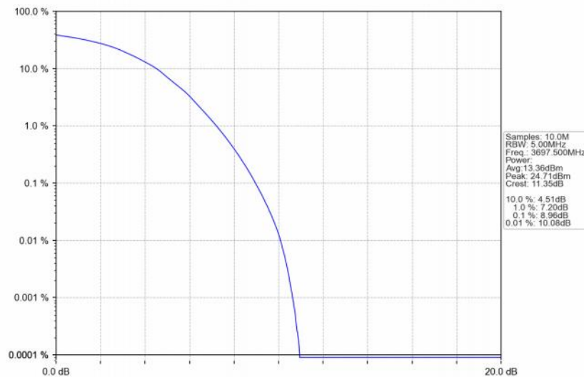
Band48_5MHz_16QAM_HCH_3697.5MHz_RB_25_0_NTNV
