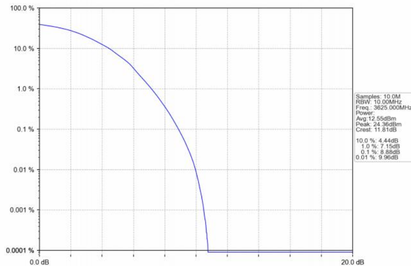
Band48_10MHz_64QAM_MCH_3625MHz_RB_50_0_NTNV
