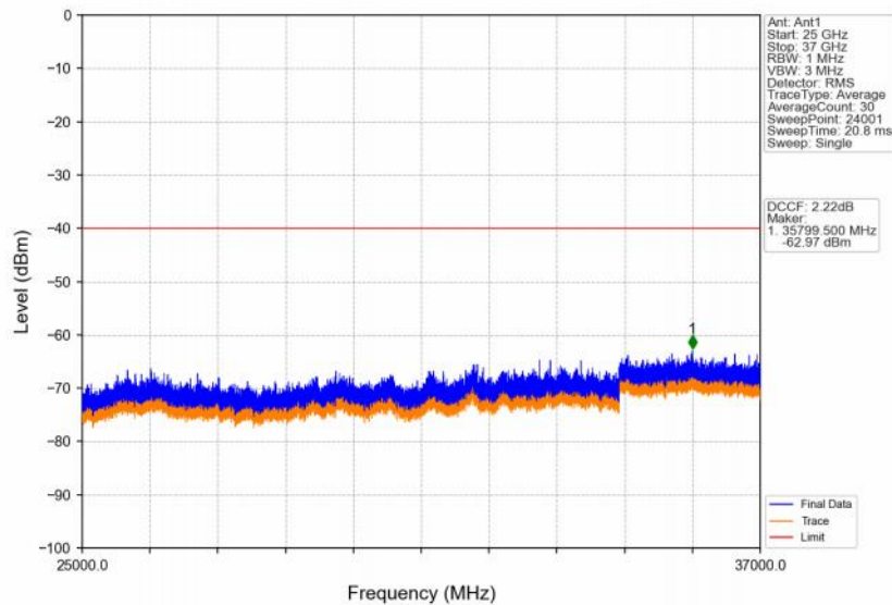
Band48_5MHz_256QAM_LCH_3552.5MHz_RB_25_0_NTNV
