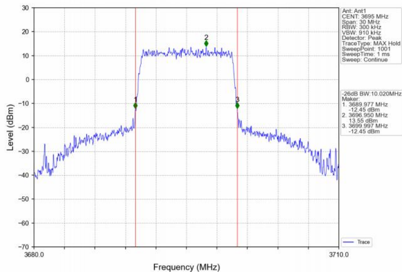
Band48_10MHz_256QAM_HCH_3695MHz_RB_50_0_NTNV
