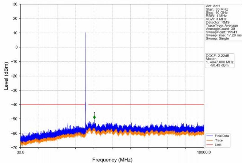
Band48_5MHz_256QAM_LCH_3552.5MHz_RB_1_0_NTNV
