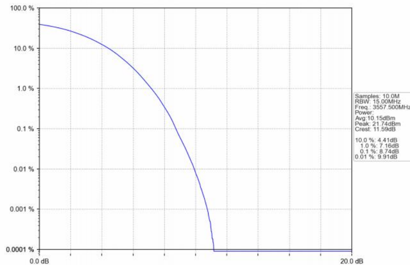
Band48_15MHz_256QAM_LCH_3557.5MHz_RB_75_0_NTNV
