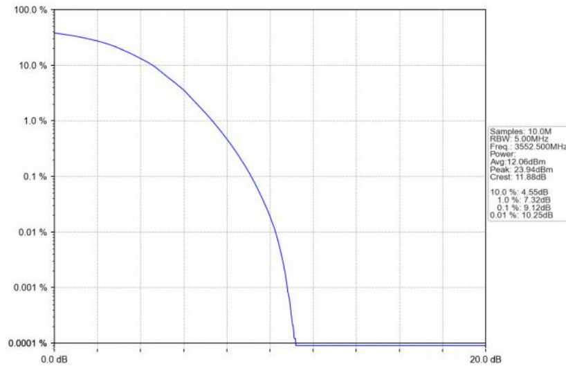
Band48_5MHz_64QAM_LCH_3552.5MHz_RB_25_0_NTNV
