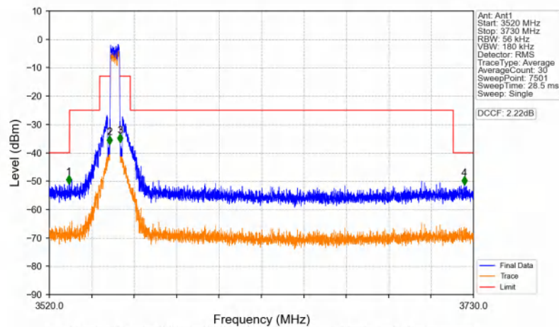
Band48_5MHz_16QAM_LCH_3552.5MHz_RB_25_0_NTNV
