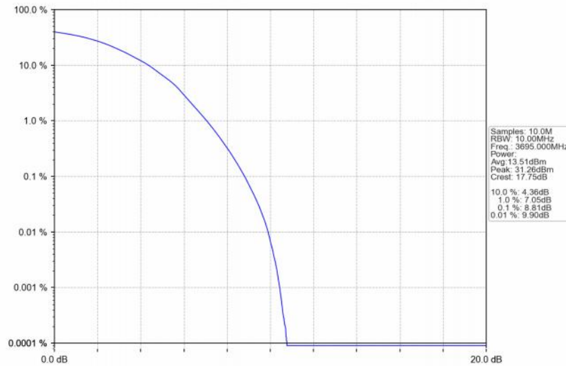
Band48_10MHz_64QAM_HCH_3695MHz_RB_50_0_NTNV
