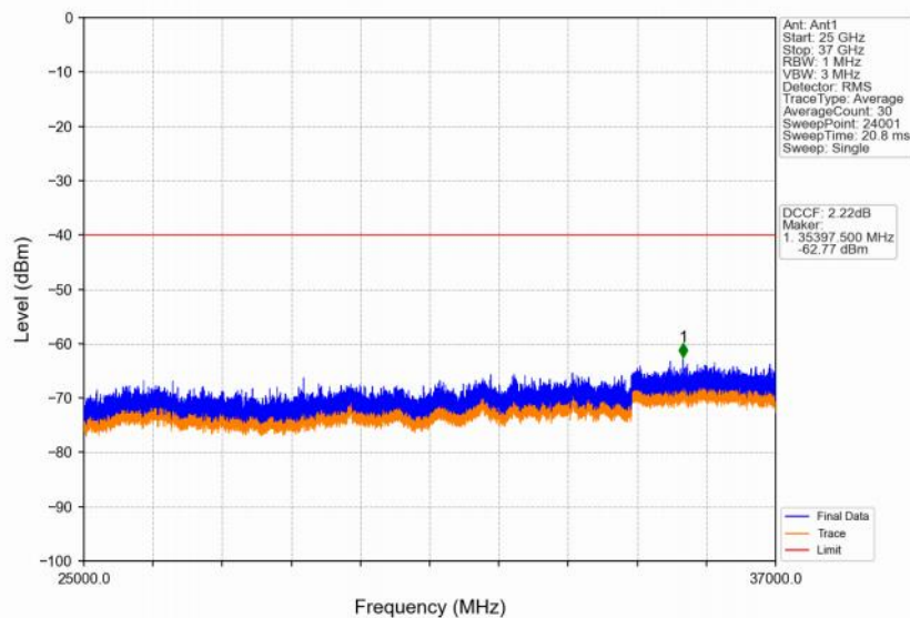
Band48_5MHz_64QAM_LCH_3552.5MHz_RB_1_0_NTNV
