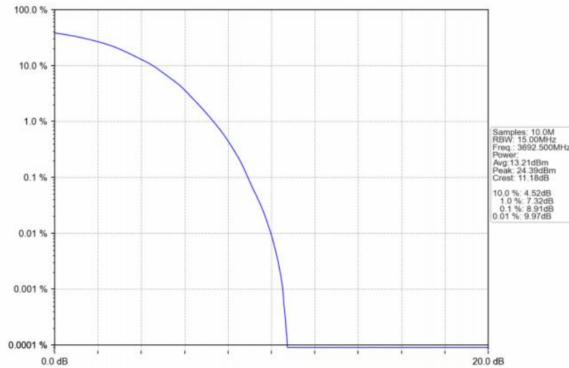
Band48_15MHz_QPSK_HCH_3692.5MHz_RB_75_0_NTNV
