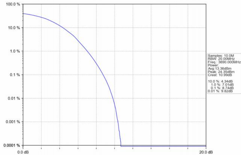
Band48_20MHz_64QAM_HCH_3690MHz_RB_100_0_NTNV
