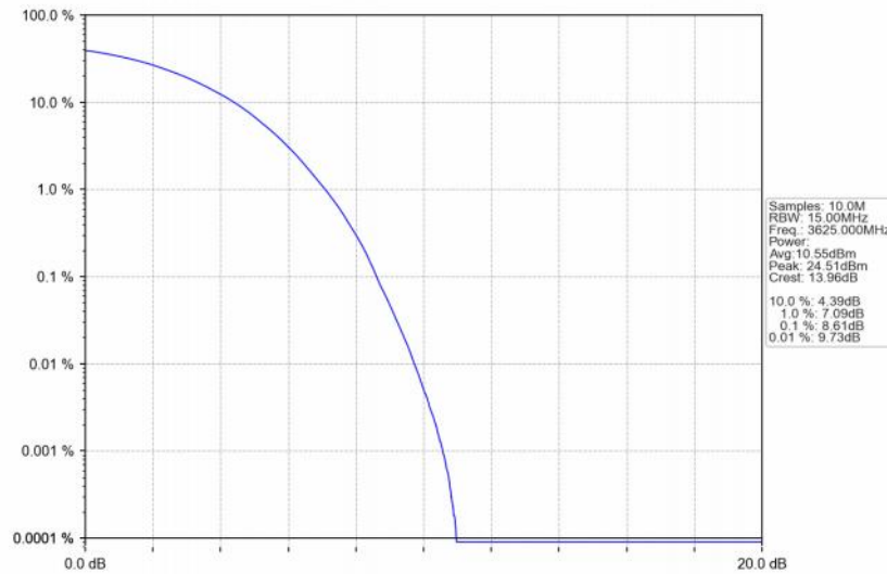
Band48_15MHz_256QAM_MCH_3625MHz_RB_75_0_NTNV
