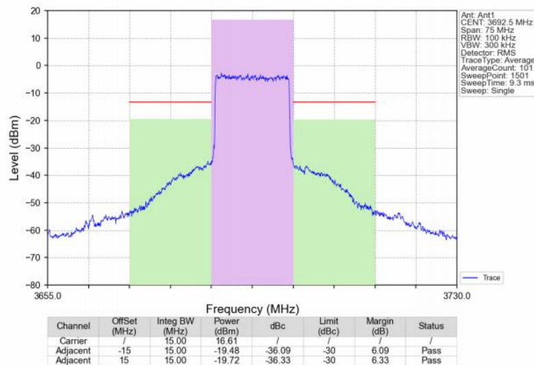
Band48_15MHz_16QAM_HCH_3692.5MHz_RB_75_0_NTNV
