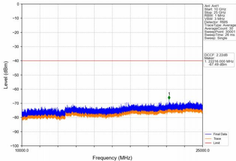
Band48_20MHz_64QAM_MCH_3625MHz_RB_1_0_NTNV
