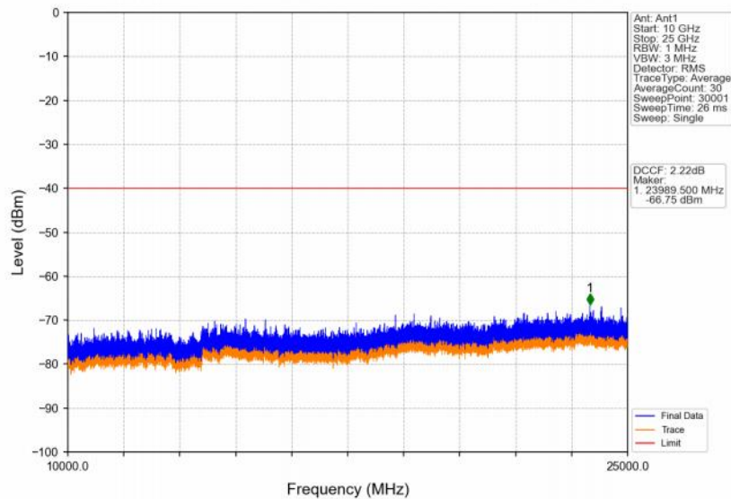
Band48_10MHz_256QAM_HCH_3695MHz_RB_1_0_NTNV
