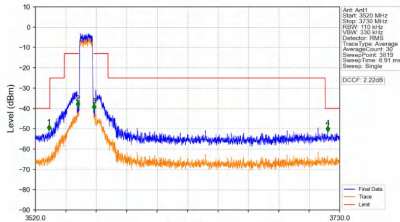
Band48_10MHz_64QAM_LCH_3555MHz_RB_50_0_NTNV
