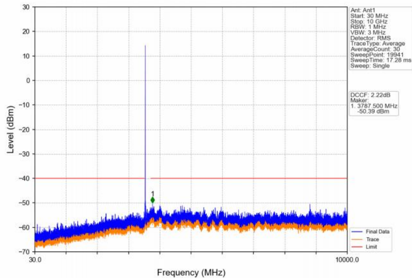
Band48_15MHz_16QAM_LCH_3557.5MHz_RB_1_0_NTNV
