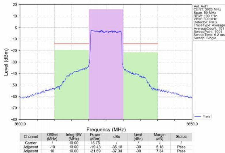
Band48_10MHz_64QAM_MCH_3625MHz_RB_50_0_NTNV
