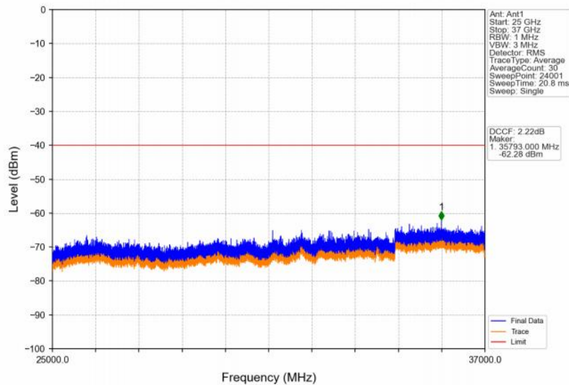
Band48_15MHz_64QAM_HCH_3692.5MHz_RB_1_74_NTNV
