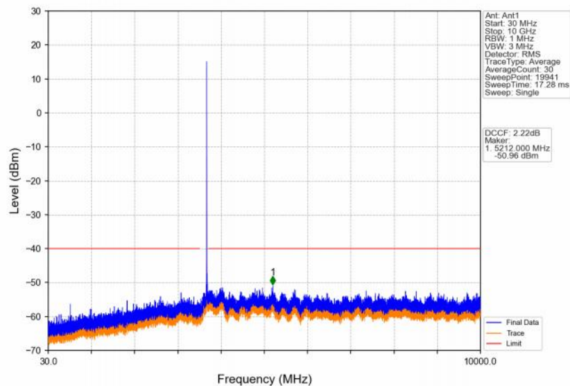
Band48_15MHz_16QAM_HCH_3692.5MHz_RB_1_0_NTNV
