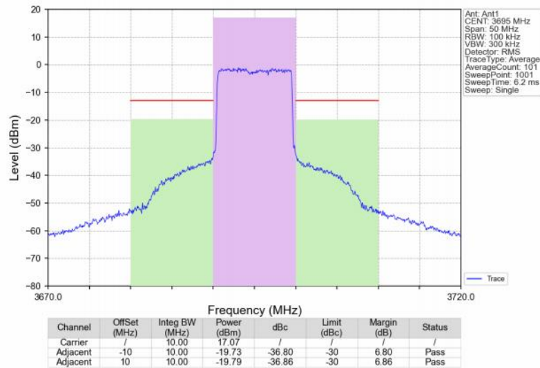
Band48 10MHz 64QAM HCH 3695MHz RB 50 0 NTN
