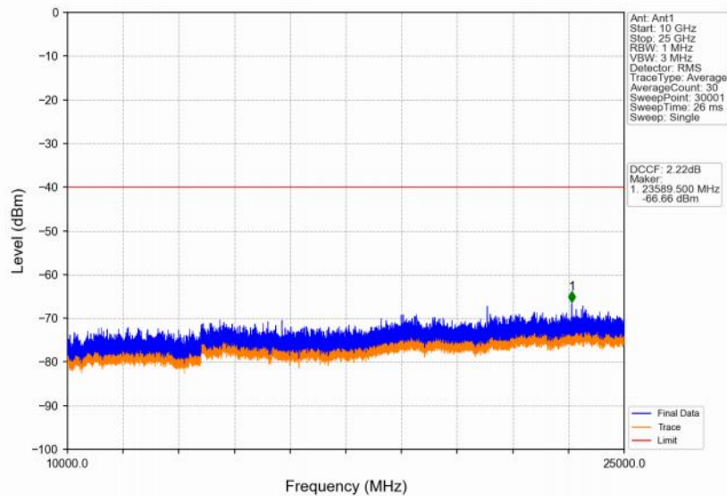
Band48_10MHz_64QAM_MCH_3625MHz_RB_1_0_NTNV
