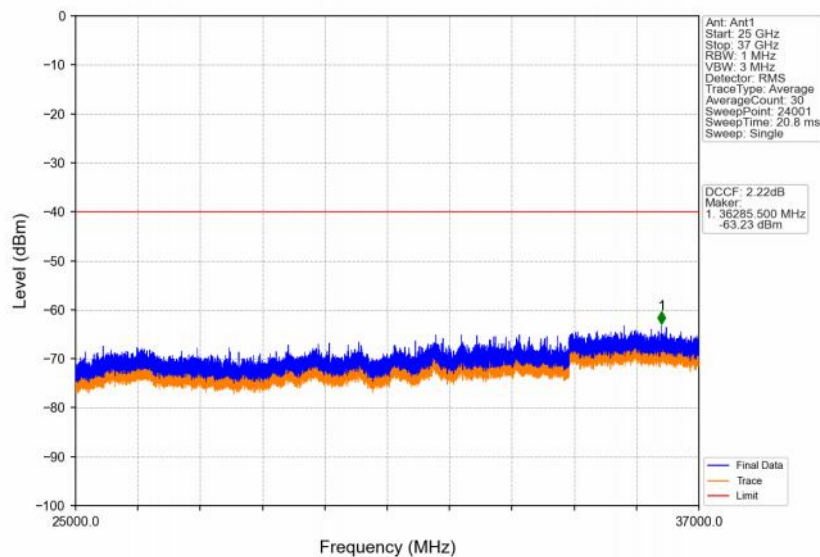
Band48_20MHz_64QAM_LCH_3560MHz_RB_1_0_NTNV
