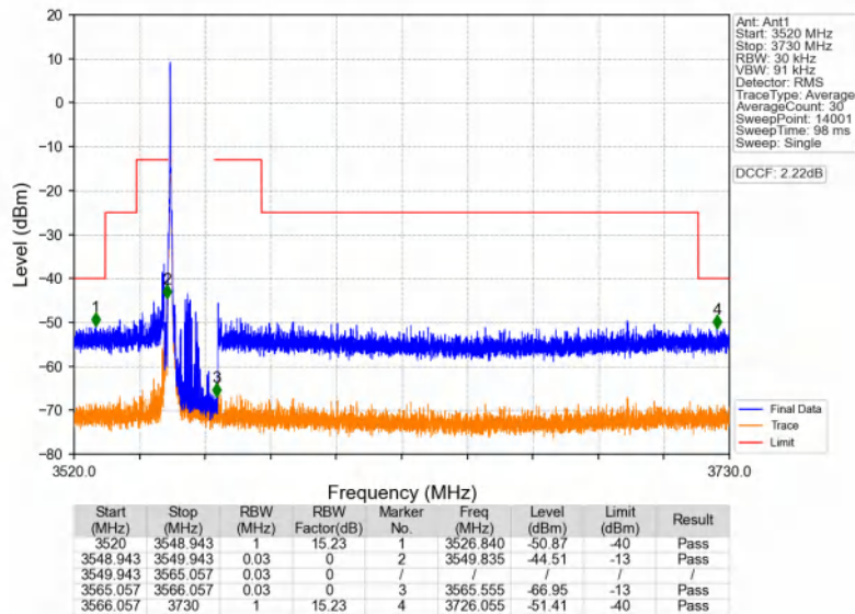
Band48_15MHz_64QAM_LCH_3557.5MHz_RB_1_0_NTNV
