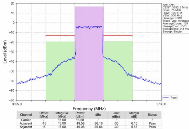
Band48_15MHz_64QAM_HCH_3692.5MHz_RB_75_0_NTNV
