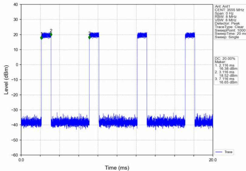
n48_30kHz_SISO_NTNV_10MHz_DFT-s-OFDM PI/2 BPSK_3555MHz_Inner_Full
