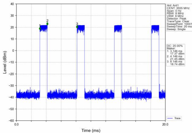
n48_30kHz_SISO_NTNV_10MHz_CP-OFDM QPSK_3555MHz_Inner_Full
