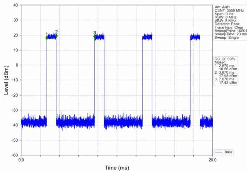
n48_30kHz_SISO_NTNV_10MHz_DFT-s-OFDM QPSK_3555MHz_Inner_Full
