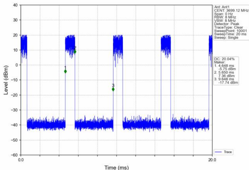
n48_30kHz_SISO_NTNV_10MHz_CP-OFDM QPSK_3694.98MHz_Edge_1RB_Right
