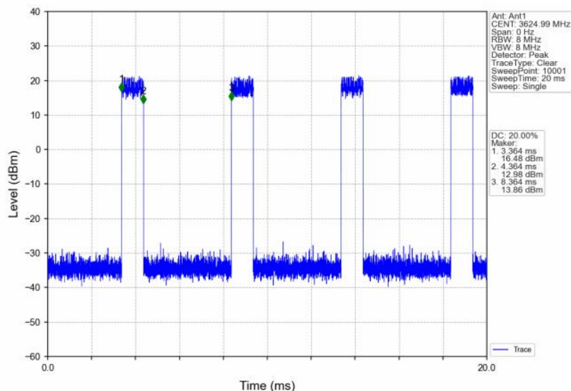
n48_30kHz_SISO_NTNV_10MHz_DFT-s-OFDM 64 QAM_3624.99MHz_Inner_Full
