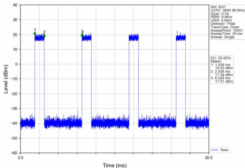
n48_30kHz_SISO_NTNV_10MHz_DFT-s-OFDM_16_QAM_3694.98MHz_Inner_Full
