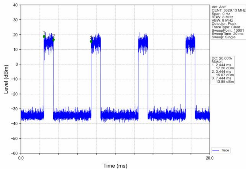
n48_30kHz_SISO_NTNV_10MHz_DFT-s-OFDM 64 QAM_3624.99MHz_Edge_1RB_Right
