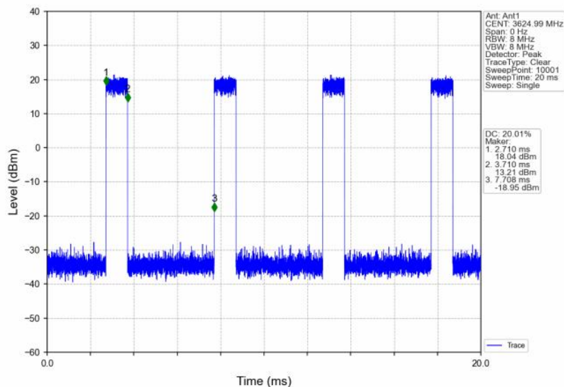
n48_30kHz_SISO_NTNV_10MHz_CP-OFDM 64 QAM_3624.99MHz_Inner_Full
