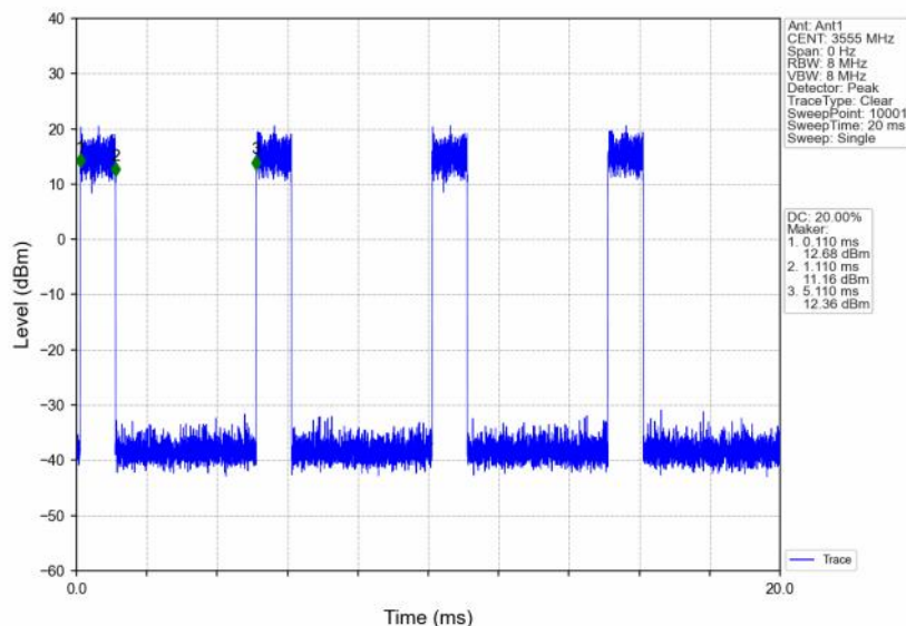
n48_30kHz_SISO_NTNV_10MHz_CP-OFDM 256 QAM_3555MHz_Inner_Full
