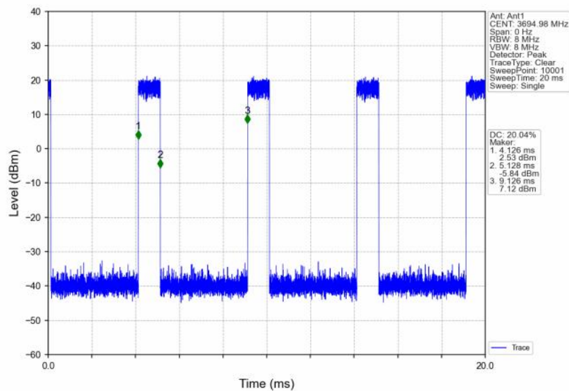
n48_30kHz_SISO_NTNV_10MHz_CP-OFDM 64 QAM_3694.98MHz_Inner_Full
