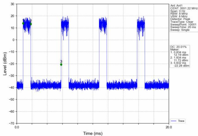
n48_30kHz_SISO_NTNV_10MHz_DFT-s-OFDM_256_QAM_3555MHz_Inner_1RB_Right
