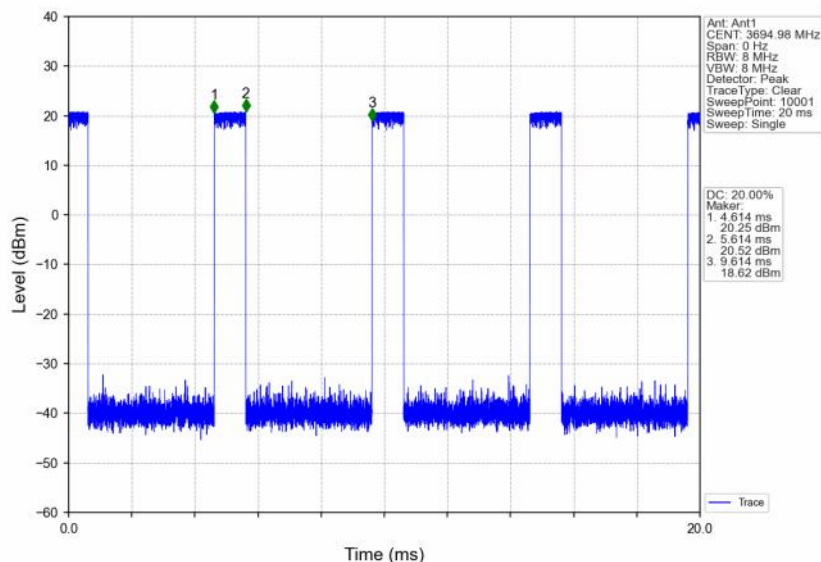
n48_30kHz_SISO_NTNV_10MHz_DFT-s-OFDM QPSK_3694.98MHz_Inner_Full
