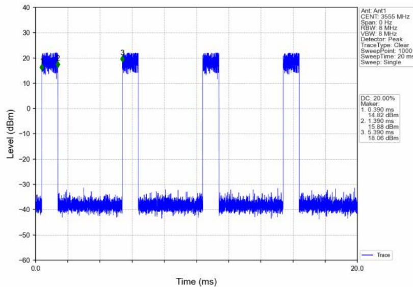
n48_30kHz_SISO_NTNV_10MHz_CP-OFDM 64 QAM_3555MHz_Inner_Full
