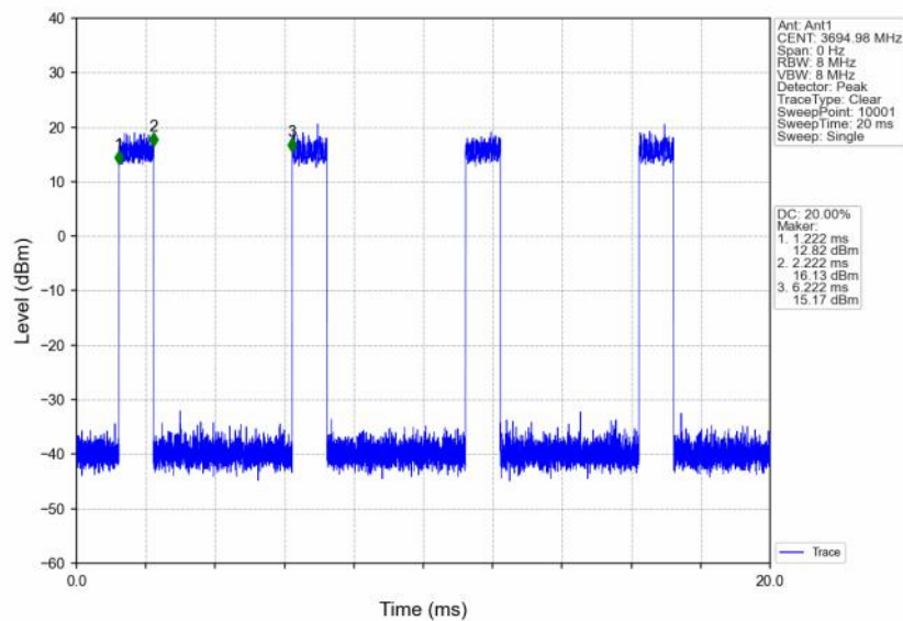
n48_30kHz_SISO_NTNV_10MHz_DFT-s-OFDM 256 QAM_3694.98MHz_Inner_Full
