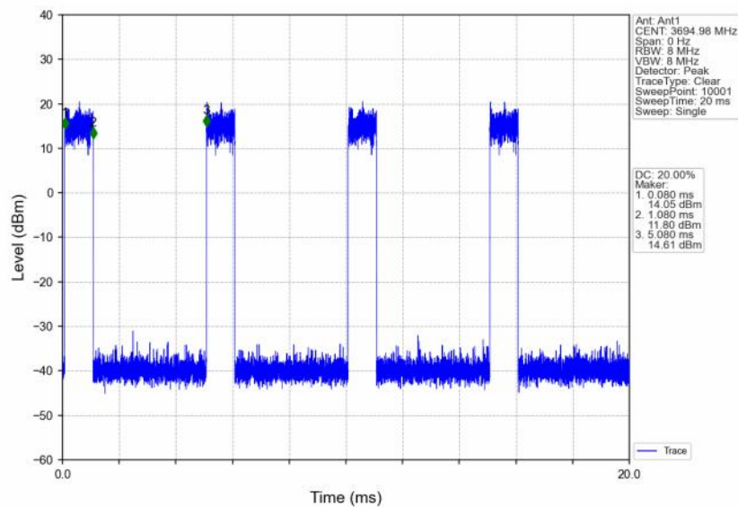
n48_30kHz_SISO_NTNV_10MHz_CP-OFDM 256 QAM_3694.98MHz_Inner_Full
