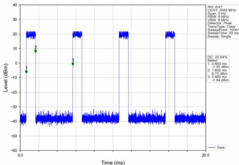
n48_30kHz_SISO_NTNV_10MHz_DFT-s-OFDM_16_QAM_3555MHz_Inner_Full
