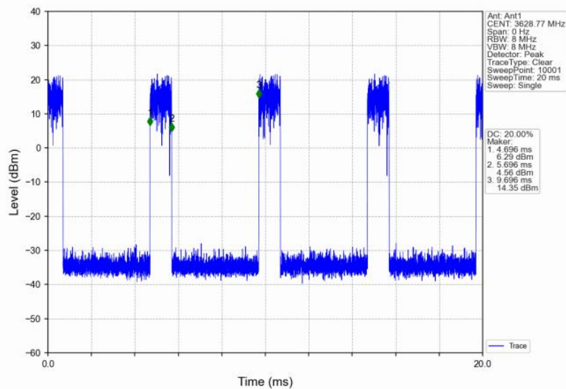
n48_30kHz_SISO_NTNV_10MHz_CP-OFDM 64 QAM 3624.99MHz_Inner_1RB_Right
