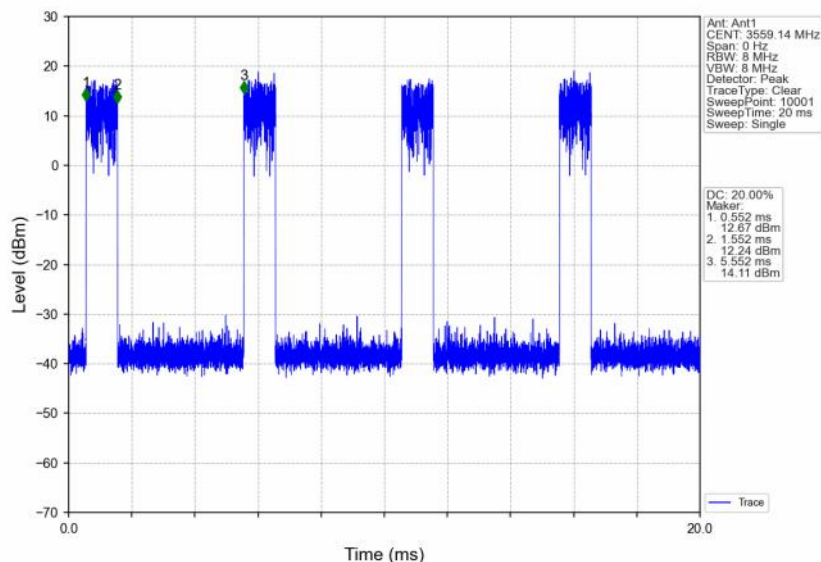
n48_30kHz_SISO_NTNV_10MHz_CP-OFDM 256 QAM 3555MHz_Edge_1RB_Right
