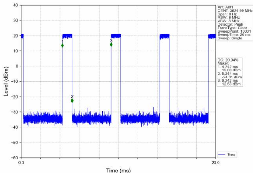
n48_30kHz_SISO_NTNV_10MHz_DFT-s-OFDM QPSK_3624.99MHz_Inner_Full
