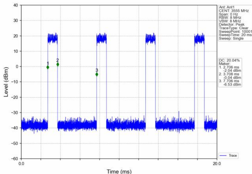
n48_30kHz_SISO_NTNV_10MHz_DFT-s-OFDM_64_QAM_3555MHz_Inner_Full
