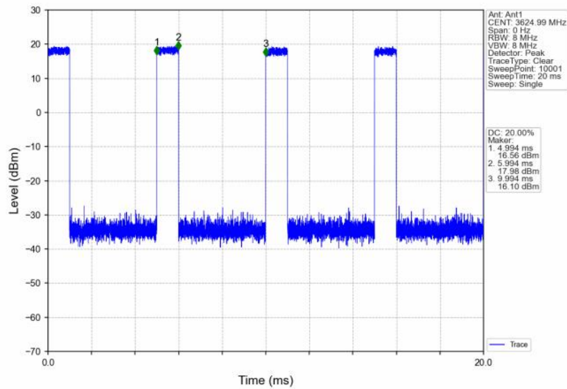
n48_30kHz_SISO_NTNV_10MHz_DFT-s-OFDM PI/2 BPSK_3624.99MHz_Inner_Full
