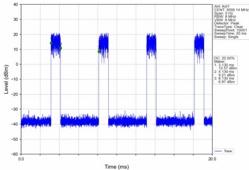
n48_30kHz_SISO_NTNV_10MHz_CP-OFDM 64 QAM 3555MHz_Edge_1RB_Right
