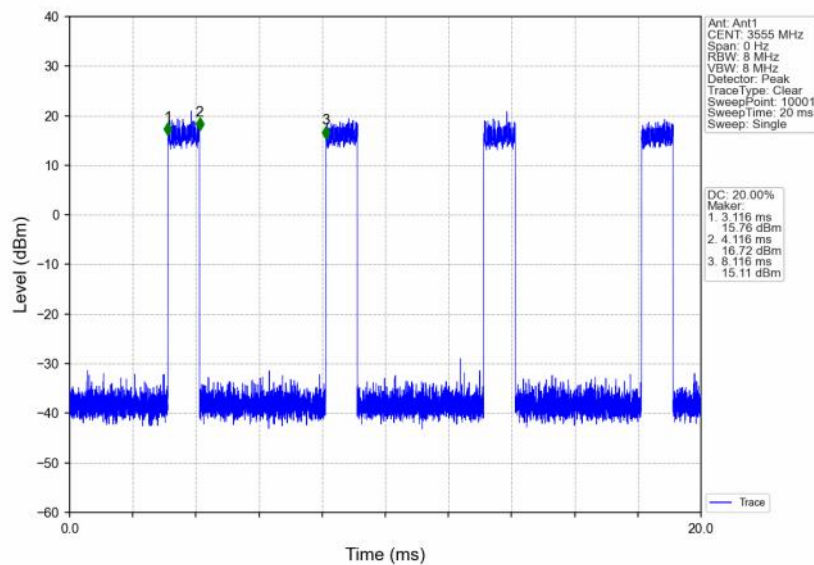
n48_30kHz_SISO_NTNV_10MHz_DFT-s-OFDM 256 QAM_3555MHz_Inner_Full
