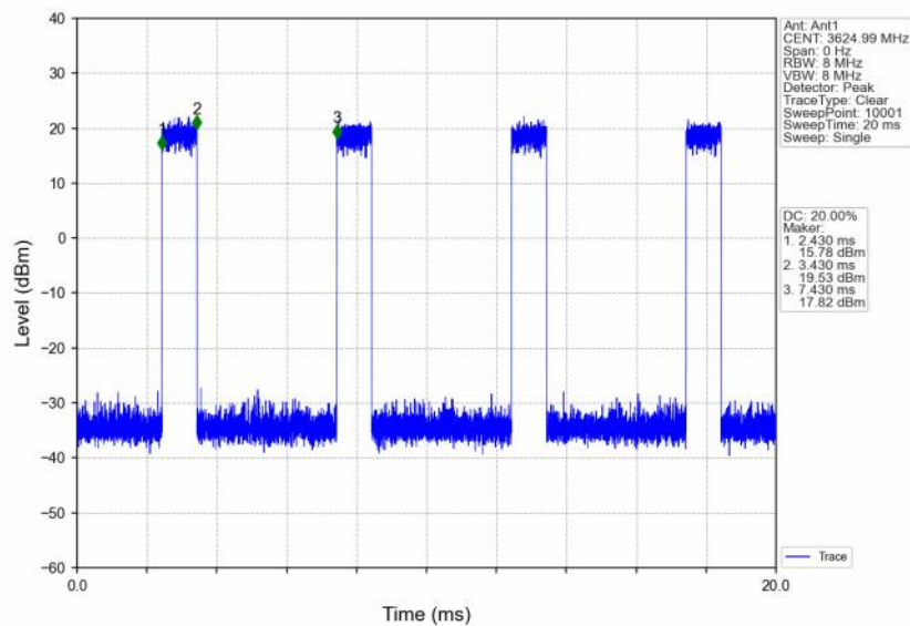
n48_30kHz_SISO_NTNV_10MHz_CP-OFDM QPSK_3624.99MHz_Inner_Full
