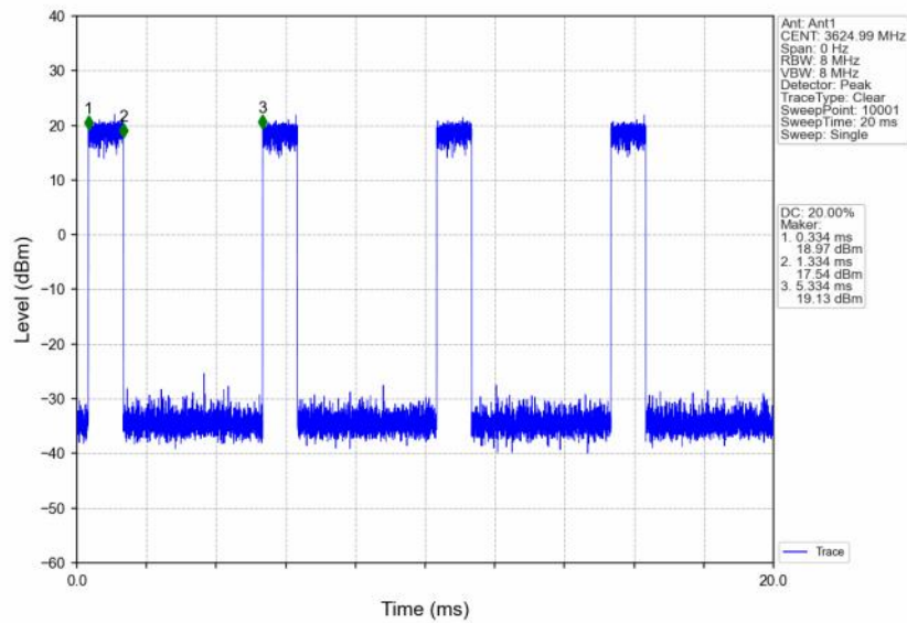
n48_30kHz_SISO_NTNV_10MHz_CP-OFDM_16_QAM_3624.99MHz_Inner_Full
