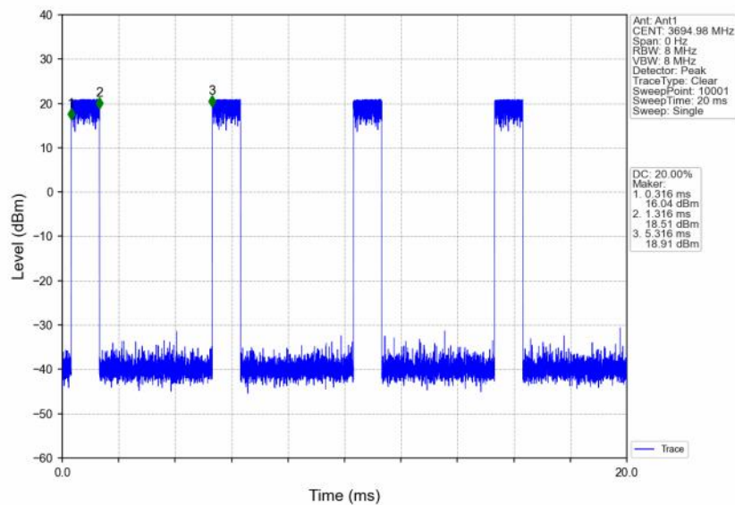
n48_30kHz_SISO_NTNV_10MHz_CP-OFDM_16_QAM_3694.98MHz_Inner_Full
