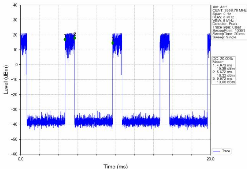
n48_30kHz_SISO_NTNV_10MHz_CP-OFDM 16 QAM 3555MHz_Inner_1RB_Right
