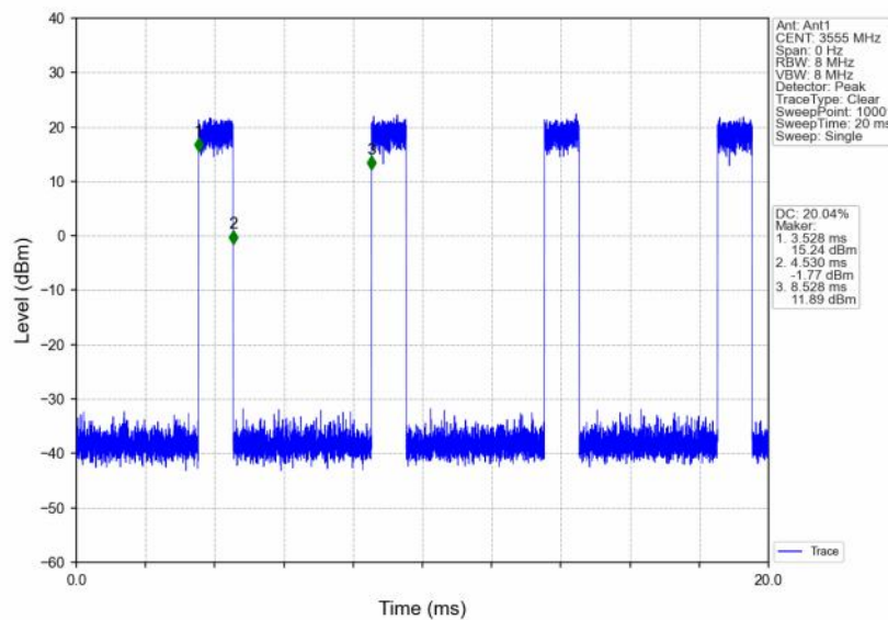
n48_30kHz_SISO_NTNV_10MHz_CP-OFDM_16 QAM_3555MHz_Inner_Full
