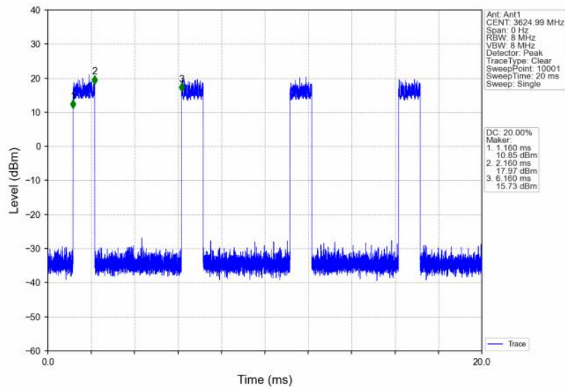
n48_30kHz_SISO_NTNV_10MHz_DFT-s-OFDM 256 QAM_3624.99MHz_Inner_Full
