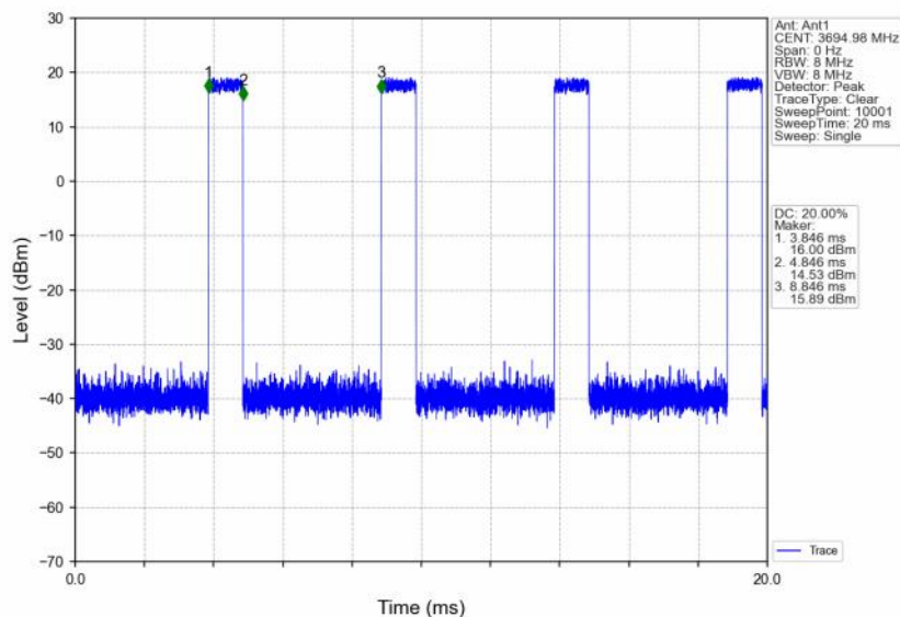
n48_30kHz_SISO_NTNV_10MHz_DFT-s-OFDM PI/2 BPSK_3694.98MHz_Inner_Full
