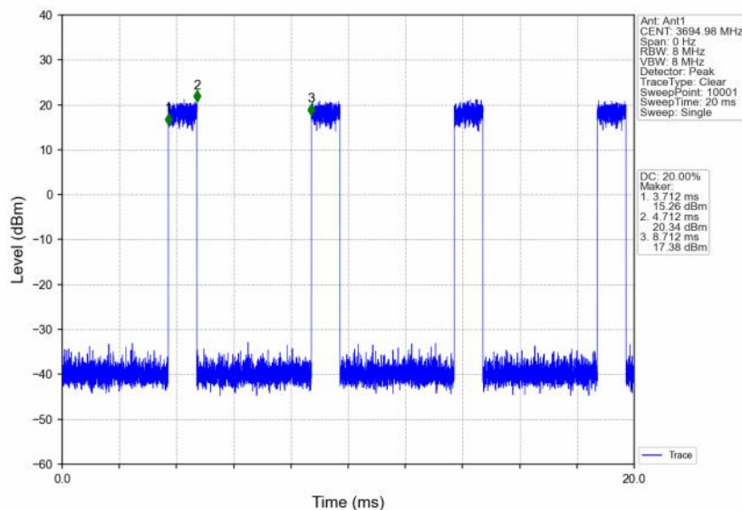
n48_30kHz_SISO_NTNV_10MHz_CP-OFDM QPSK_3694.98MHz_Inner_Full
