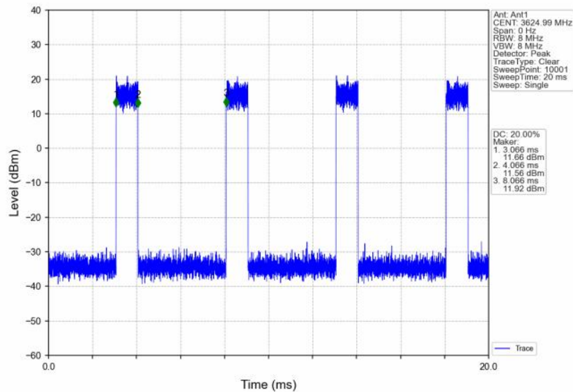
n48_30kHz_SISO_NTNV_10MHz_CP-OFDM 256 QAM_3624.99MHz_Inner_Full
