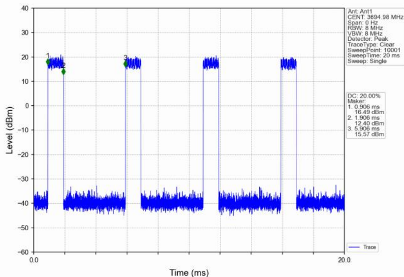
n48_30kHz_SISO_NTNV_10MHz_DFT-s-OFDM 64 QAM_3694.98MHz_Inner_Full
