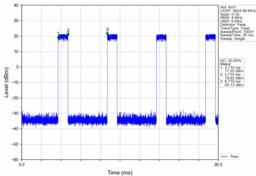
n48_30kHz_SISO_NTNV_10MHz_DFT-s-OFDM_16_QAM_3624.99MHz_Inner_Full
