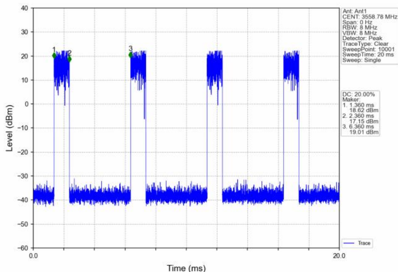
n48_30kHz_SISO_NTNV_10MHz_CP-OFDM_QPSK_3555MHz_Inner_1RB_Right
