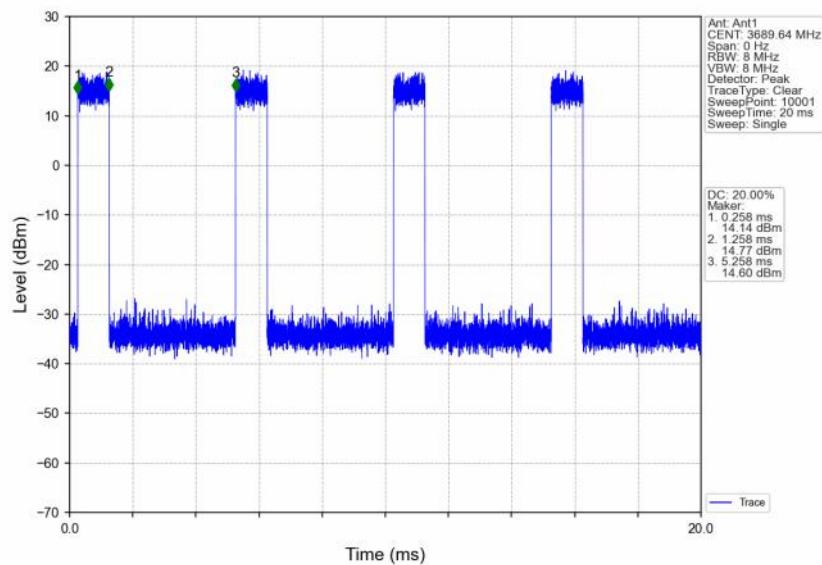
n48_30kHz_SISO_NTNV_20MHz_CP-OFDM 256 QAM_3690MHz_Inner_Full
