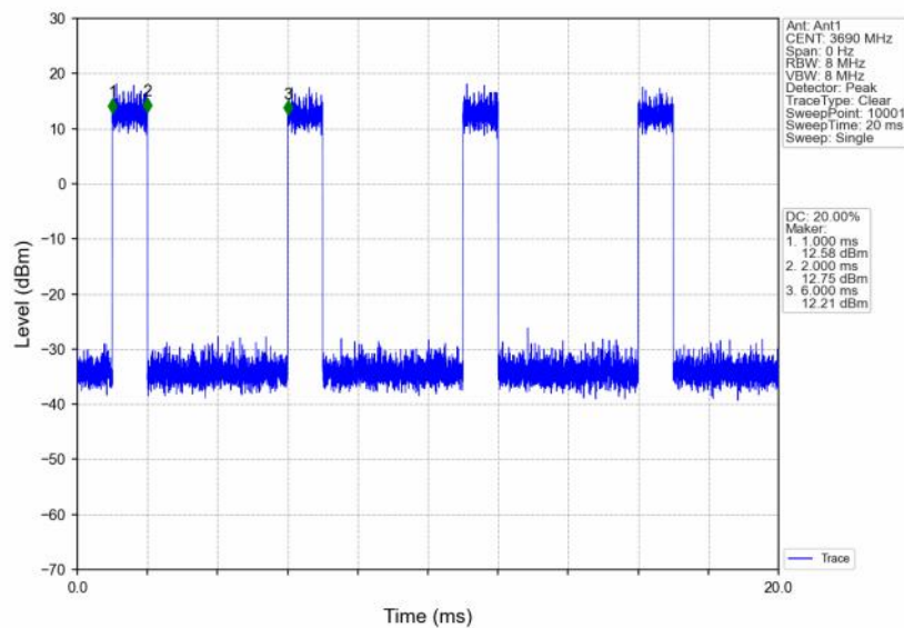
n48_30kHz_SISO_NTNV_20MHz_CP-OFDM 256 QAM_3690MHz_Inner_Full
