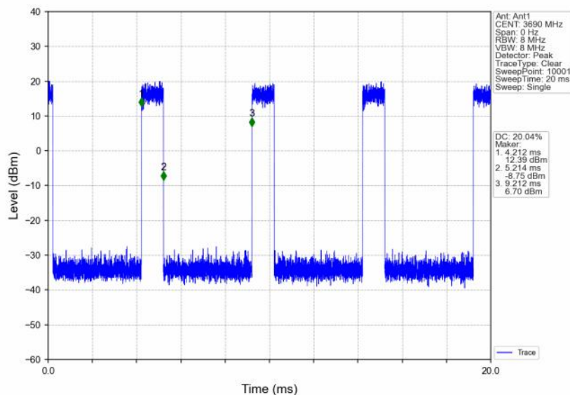
n48_30kHz_SISO_NTNV_20MHz_CP-OFDM_16 QAM_3690MHz_Inner_Full
