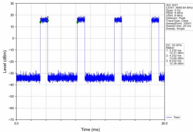
n48_30kHz_SISO_NTNV_20MHz_DFT-s-OFDM 256 QAM_3690MHz_Inner_Full
