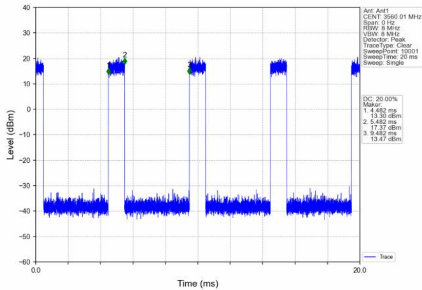
n48_30kHz_SISO_NTNV_20MHz_CP-OFDM QPSK_3560.01MHz_Inner_Full
