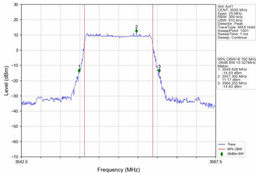
n48_30kHz_SISO_NTNV_10MHz_DFT-s-OFDM QPSK_3555MHz_Outer_Full
