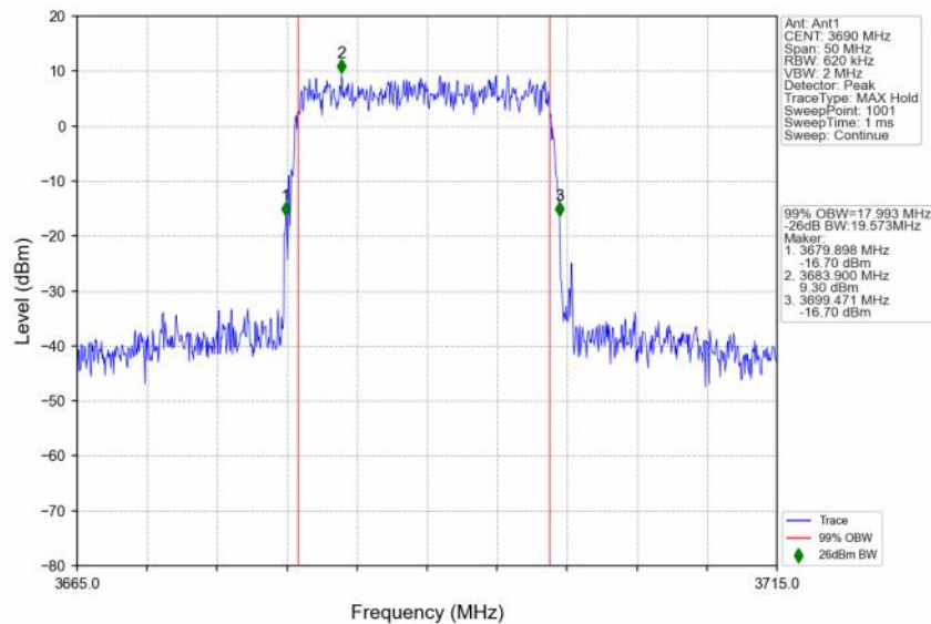
n48_30kHz_SISO_NTNV_20MHz_DFT-s-OFDM_64_QAM_3690MHz_Outer_Full
