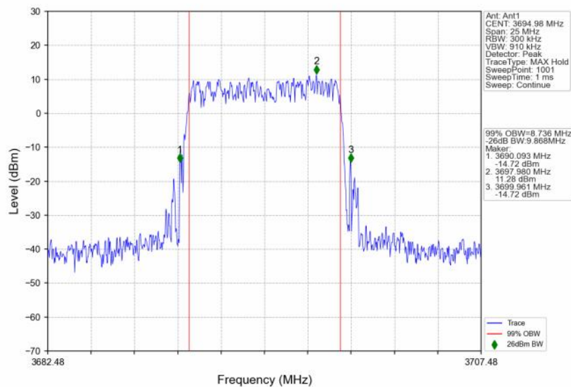
n48_30kHz_SISO_NTNV_10MHz_DFT-s-OFDM QPSK_3694.98MHz_Outer_Full
