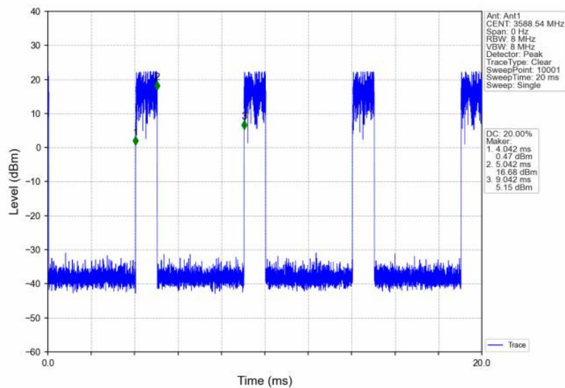
n48_30kHz_SISO_NTNV_40MHz_CP-OFDM 16 QAM 3570MHz_Inner_1RB_Right
