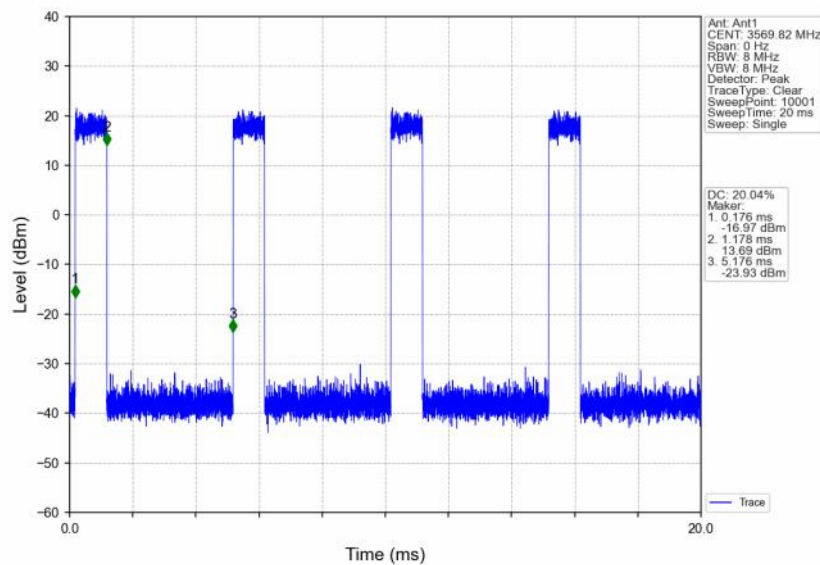
n48_30kHz_SISO_NTNV_40MHz_CP-OFDM_QPSK_3570MHz_Inner_Full
