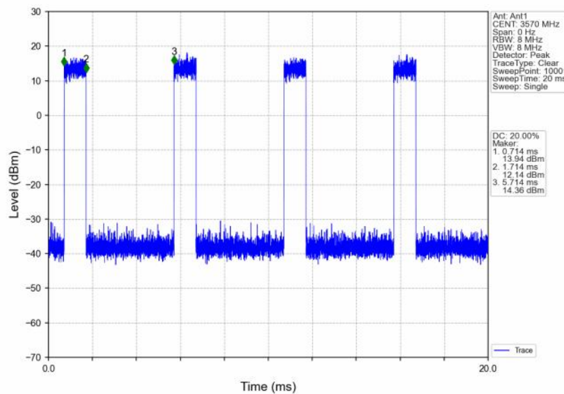
n48_30kHz_SISO_NTNV_40MHz_CP-OFDM_16_QAM_3570MHz_Inner_Full
