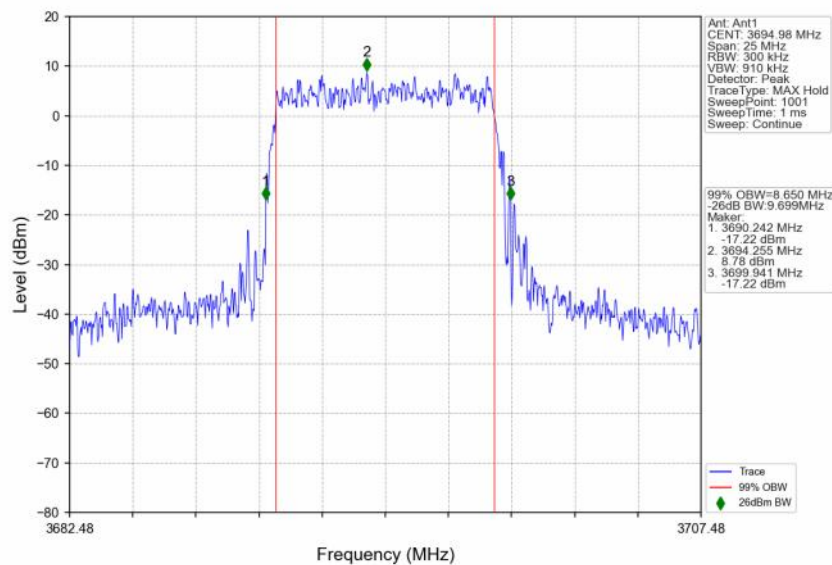
n48_30kHz_SISO_NTNV_10MHz_CP-OFDM QPSK_3694.98MHz_Outer_Full
