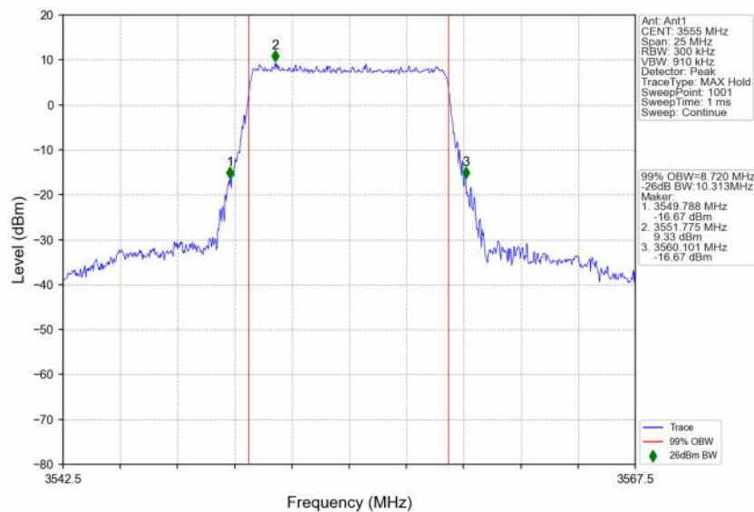
n48_30kHz_SISO_NTNV_10MHz_DFT-s-OFDM 64 QAM_3555MHz_Outer_Full
