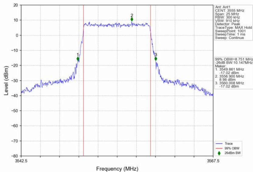
n48_30kHz_SISO_NTNV_10MHz_CP-OFDM 64 QAM_3555MHz_Outer_Full
