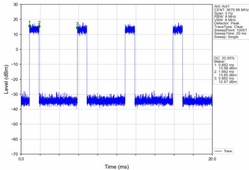
n48_30kHz_SISO_NTNV_40MHz_CP-OFDM_16_QAM_3679.98MHz_Inner_Full
