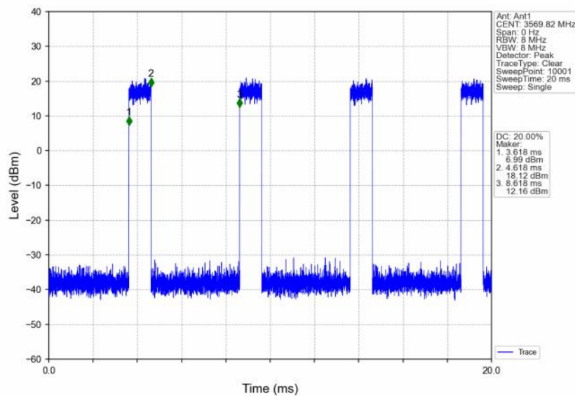
n48_30kHz_SISO_NTNV_40MHz_CP-OFDM_16_QAM_3570MHz_Inner_Full
