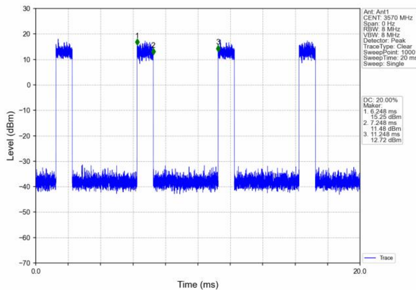
n48_30kHz_SISO_NTNV_40MHz_CP-OFDM 64 QAM_3570MHz_Inner_Full
