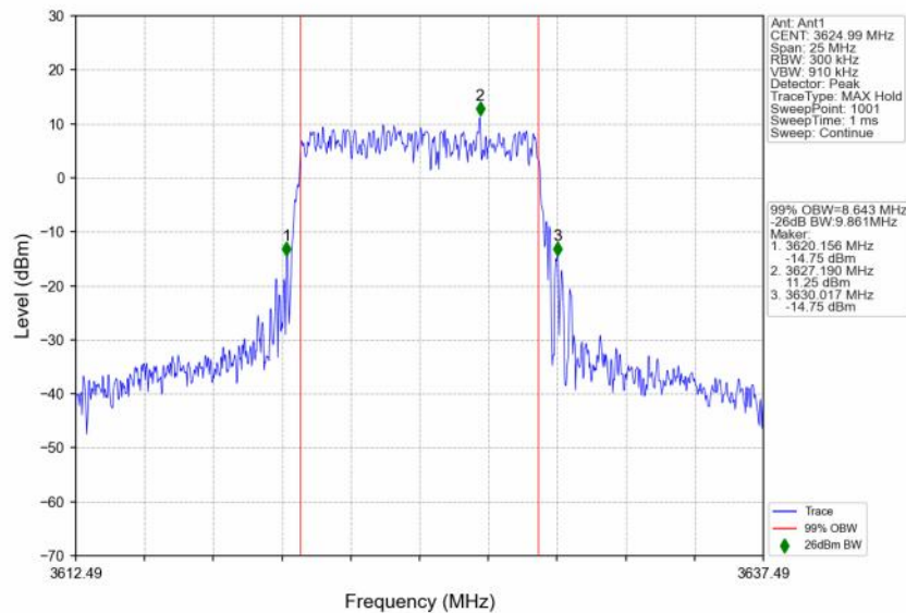
n48_30kHz_SISO_NTNV_10MHz_DFT-s-OFDM_16_QAM_3624.99MHz_Outer_Full
