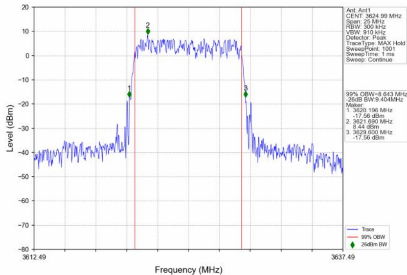
n48_30kHz_SISO_NTNV_10MHz_DFT-s-OFDM_256_QAM_3624.99MHz_Outer_Full
