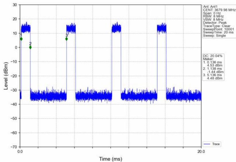
n48_30kHz_SISO_NTNV_40MHz_CP-OFDM QPSK_3679.98MHz_Inner_Full
