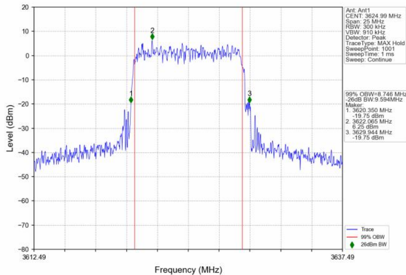
n48_30kHz_SISO_NTNV_10MHz_CP-OFDM 256 QAM_3624.99MHz_Outer_Full
