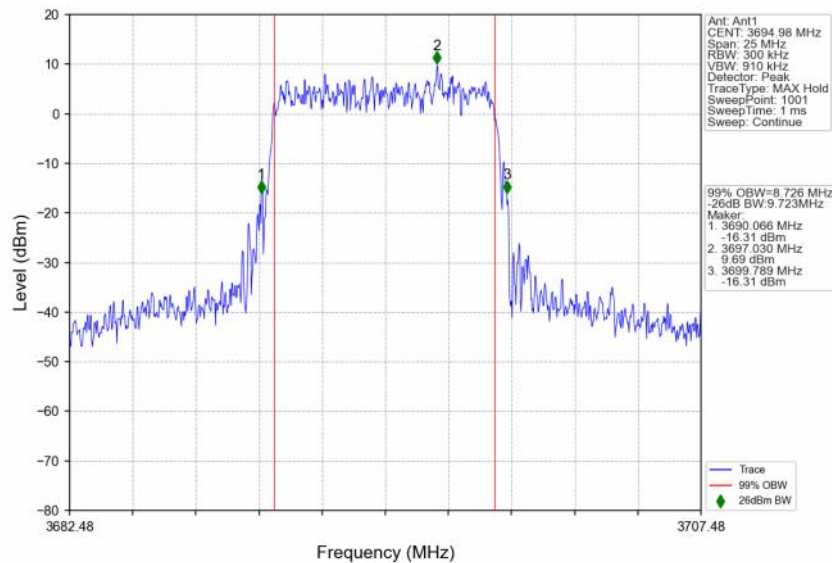
n48_30kHz_SISO_NTNV_10MHz_CP-OFDM_64_QAM_3694.98MHz_Outer_Full
