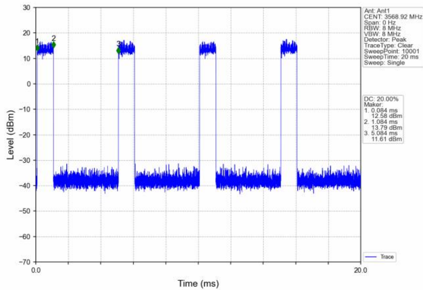
n48_30kHz_SISO_NTNV_40MHz_DFT-s-OFDM_64_QAM_3570MHz_Inner_Full
