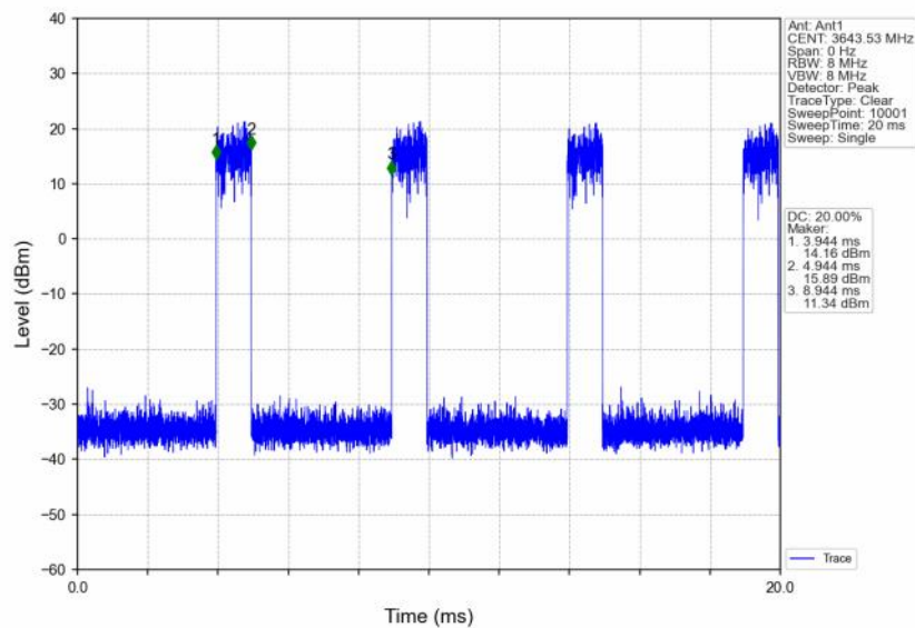
n48_30kHz_SISO_NTNV_40MHz_DFT-s-OFDM 64 QAM 3624.99MHz_Inner_1RB_Right
