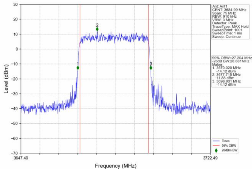
n48_30kHz_SISO_NTNV_30MHz_DFT-s-OFDM QPSK_3684.99MHz_Outer_Full
