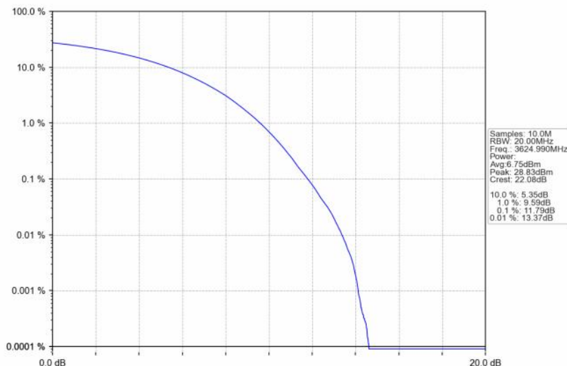
n48_30kHz_SISO_NTNV_20MHz_CP-OFDM_256_QAM_3624.99MHz_Outer_Full
