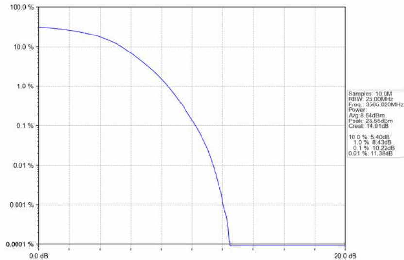
n48_30kHz_SISO_NTNV_30MHz_DFT-s-OFDM_256_QAM_3565.02MHz_Outer_Full
