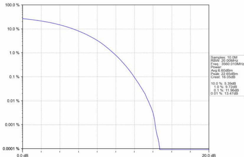
n48_30kHz_SISO_NTNV_20MHz_CP-OFDM_256_QAM_3560.01MHz_Outer_Full
