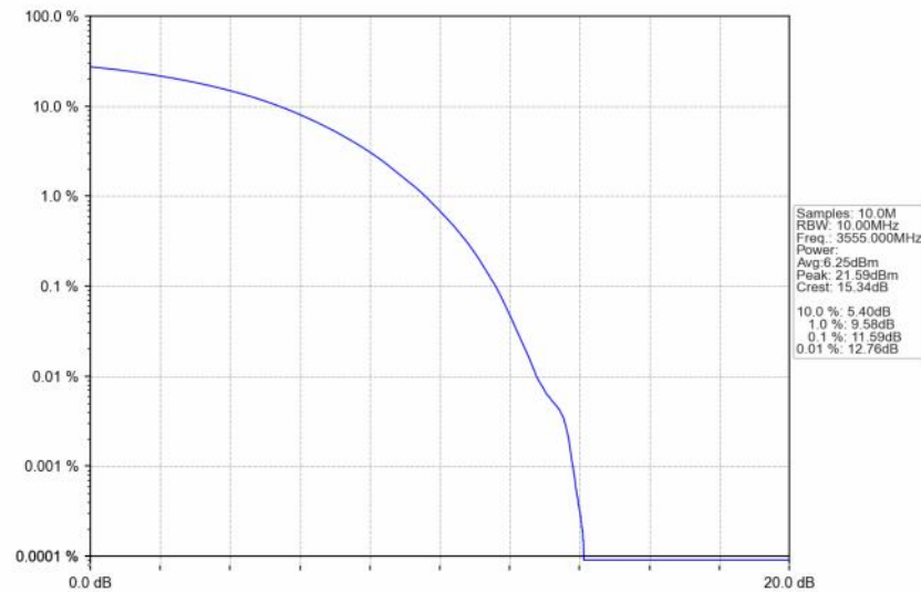
n48_30kHz_SISO_NTNV_10MHz_CP-OFDM 256 QAM_3555MHz_Outer_Full
