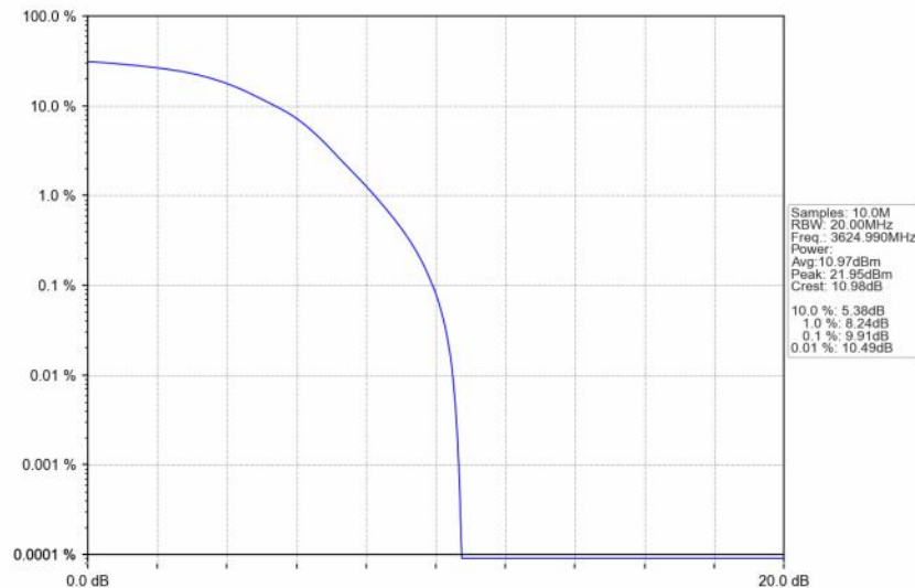
n48_30kHz_SISO_NTNV_20MHz_DFT-s-OFDM_16_QAM_3624.99MHz_Outer_Full
