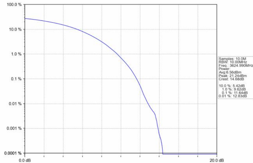
n48_30kHz_SISO_NTNV_10MHz_CP-OFDM 256 QAM_3624.99MHz_Outer_Full
