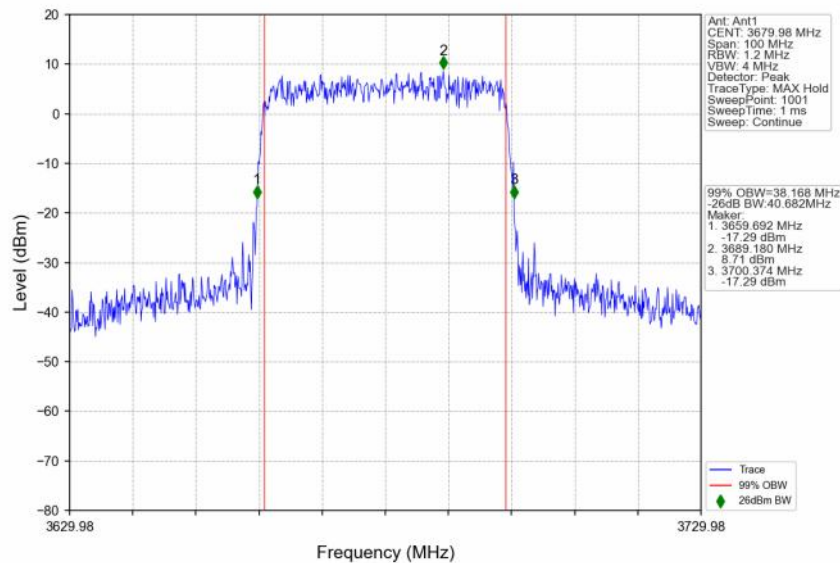
n48_30kHz_SISO_NTNV_40MHz_CP-OFDM_64_QAM_3679.98MHz_Outer_Full
