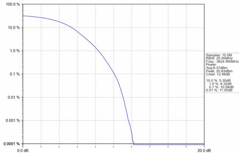
n48_30kHz_SISO_NTNV_30MHz_DFT-s-OFDM_256_QAM_3624.99MHz_Outer_Full
