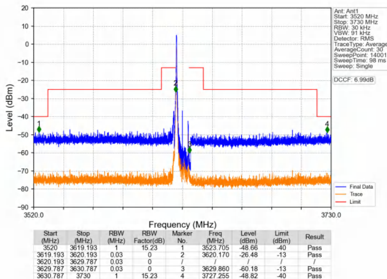
n48_30kHz_SISO_NTNV_10MHz_CP-OFDM QPSK_3624.99MHz_Edge_1RB_Left
