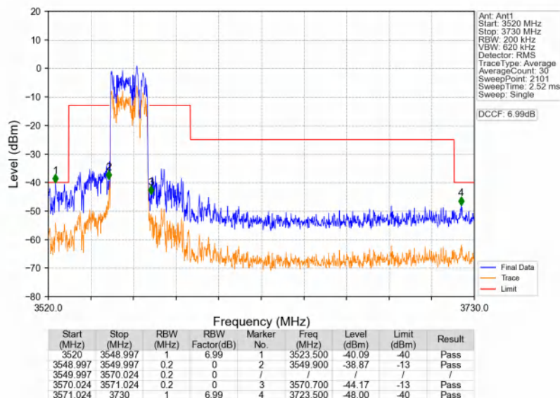
n48_30kHz_SISO_NTNV_20MHz_DFT-s-OFDM QPSK_3560.01MHz_Outer_Full
