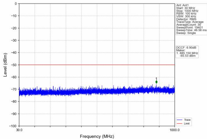
n48_30kHz_SISO_NTNV_20MHz_DFT-s-OFDM_PI/2_BPSK_3560.01MHz_Outer_Full
