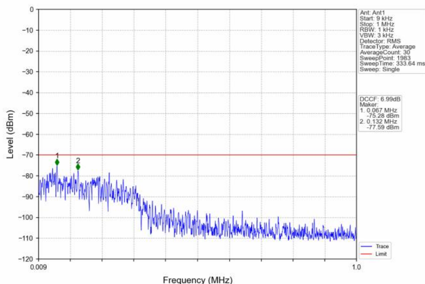
n48_30kHz_SISO_NTNV_20MHz_CP-OFDM QPSK_3560.01MHz_Edge_1RB_Left
