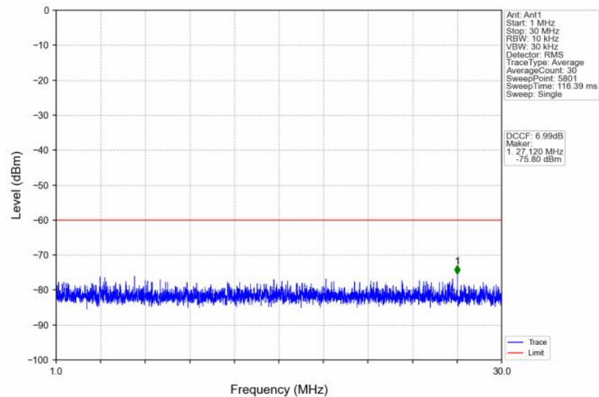
n48_30kHz_SISO_NTNV_10MHz_DFT-s-OFDM QPSK_3694.98MHz_Inner_1RB_Right
