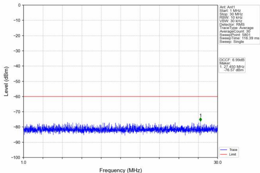
n48_30kHz_SISO_NTNV_10MHz_CP-OFDM QPSK_3694.98MHz_Inner_1RB_Right
