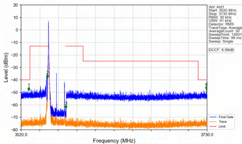
n48_30kHz_SISO_NTNV_20MHz_DFT-s-OFDM QPSK_3560.01MHz_Edge_1RB_Left
