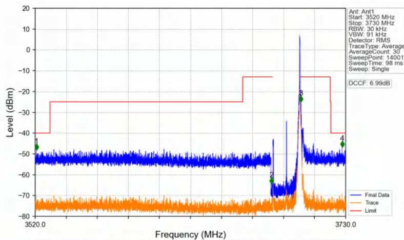
n48_30kHz_SISO_NTNV_20MHz_DFT-s-OFDM QPSK_3690MHz_Edge_1RB_Right
