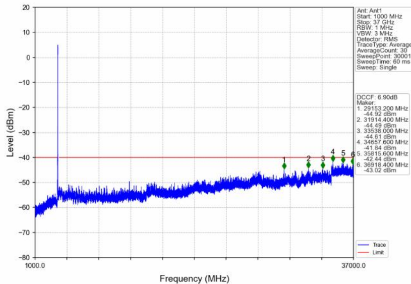
n48_30kHz_SISO_NTNV_20MHz_DFT-s-OFDM_PI/2_BPSK_3560.01MHz_Outer_Full
