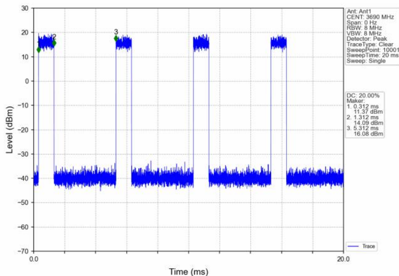
n48_30kHz_SISO_NTNV_20MHz_CP-OFDM_64_QAM_3690MHz_Inner_Full
