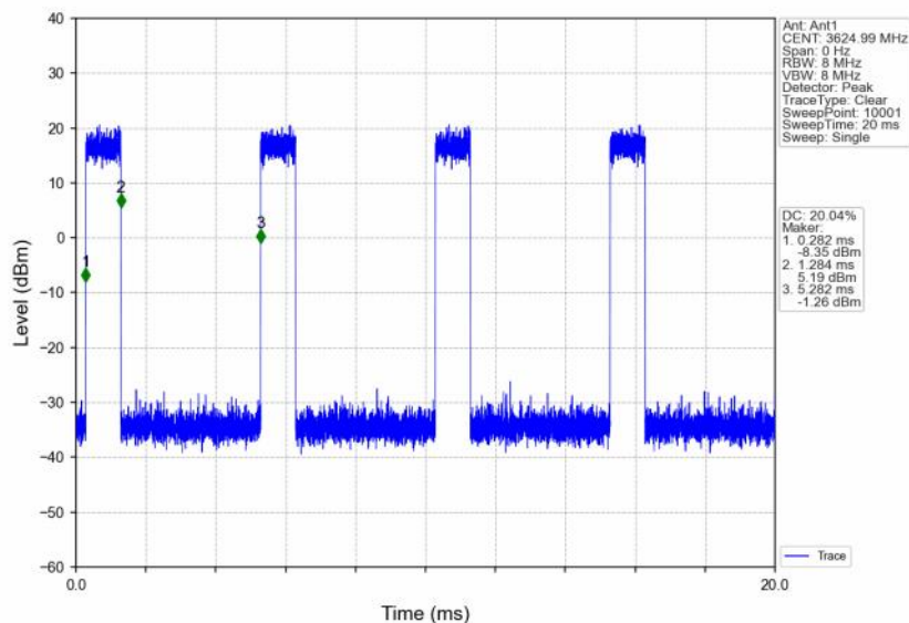
n48_30kHz_SISO_NTNV_20MHz_CP-OFDM_16_QAM_3624.99MHz_Inner_Full
