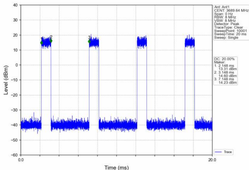
n48_30kHz_SISO_NTNV_20MHz_CP-OFDM 256 QAM_3690MHz_Inner_Full
