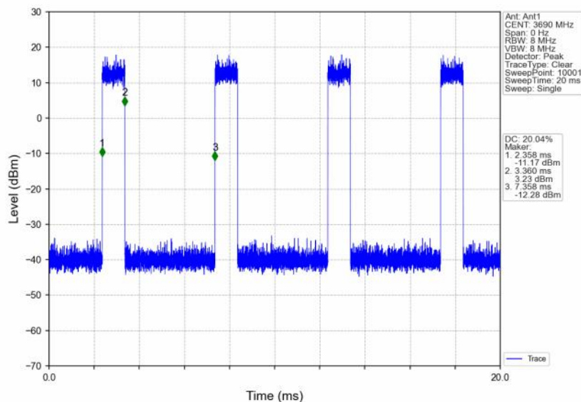
n48_30kHz_SISO_NTNV_20MHz_CP-OFDM 256 QAM_3690MHz_Inner_Full
