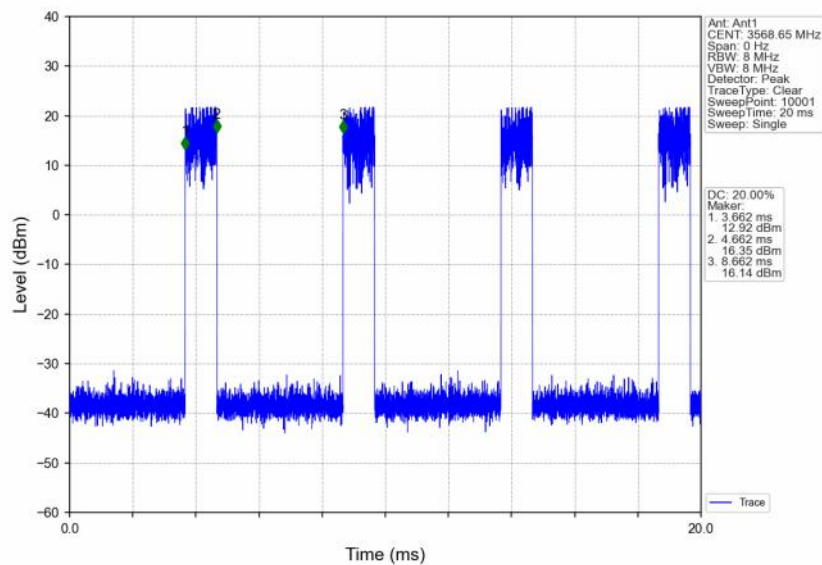
n48_30kHz_SISO_NTNV_20MHz_CP-OFDM_16_QAM_3560.01MHz_Inner_1RB_Right
