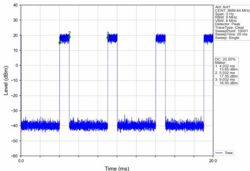
n48_30kHz_SISO_NTNV_20MHz_CP-OFDM_64_QAM_3690MHz_Inner_Full
