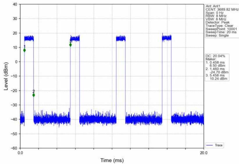
n48_30kHz_SISO_NTNV_20MHz_DFT-s-OFDM_16_QAM_3690MHz_Inner_Full
