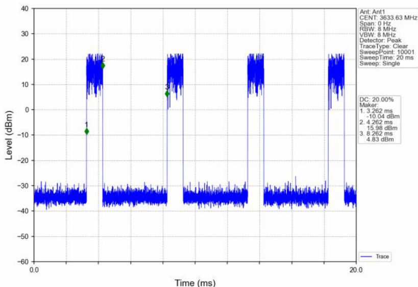
n48_30kHz_SISO_NTNV_20MHz_CP-OFDM_16_QAM_3624.99MHz_Inner_1RB_Right
