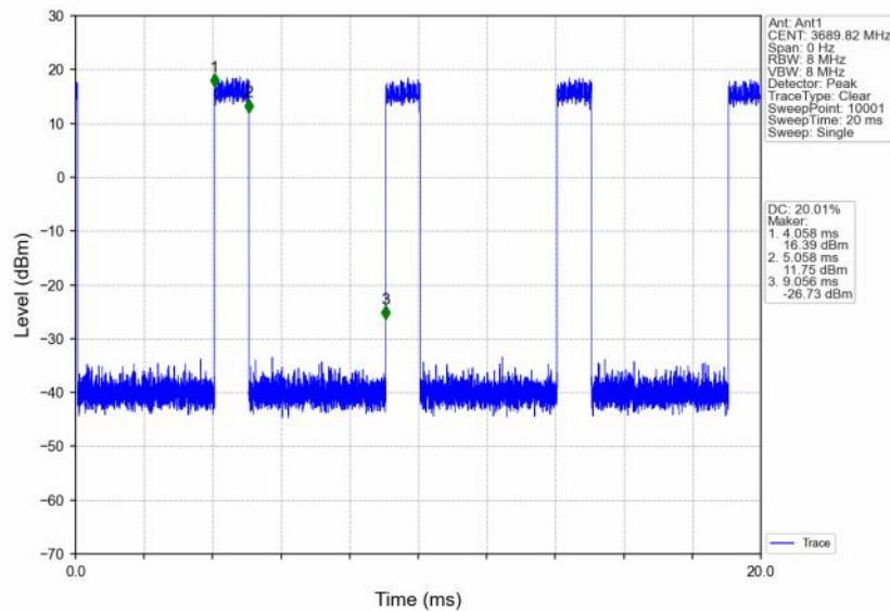
n48_30kHz_SISO_NTNV_20MHz_DFT-s-OFDM_64_QAM_3690MHz_Inner_Full
