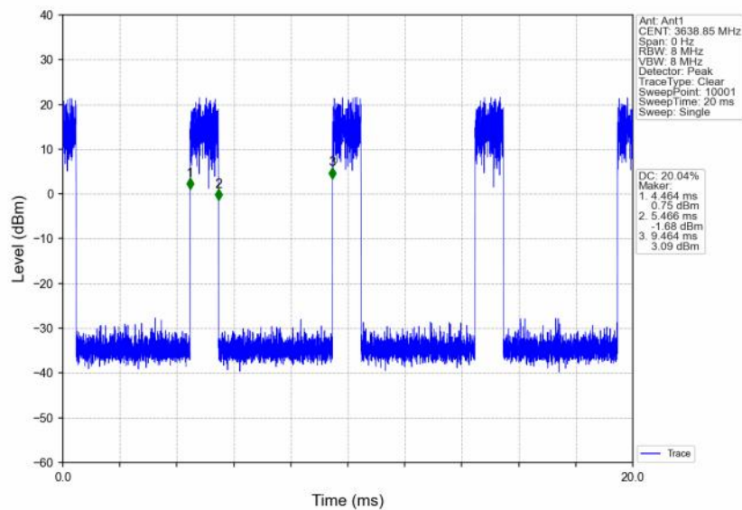
n48_30kHz_SISO_NTNV_30MHz_CP-OFDM 64 QAM 3624.99MHz_Edge_1RB_Right
