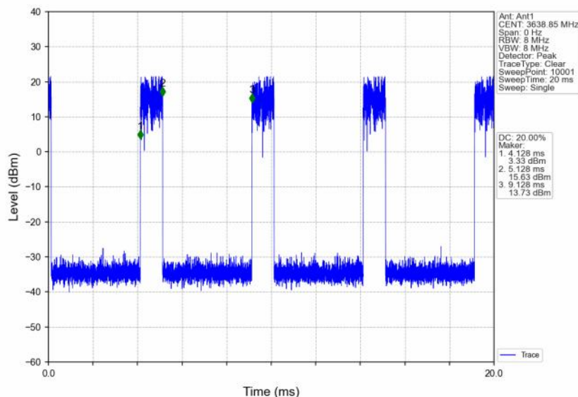
n48_30kHz_SISO_NTNV_30MHz_CP-OFDM_16_QAM_3624.99MHz_Edge_1RB_Right
