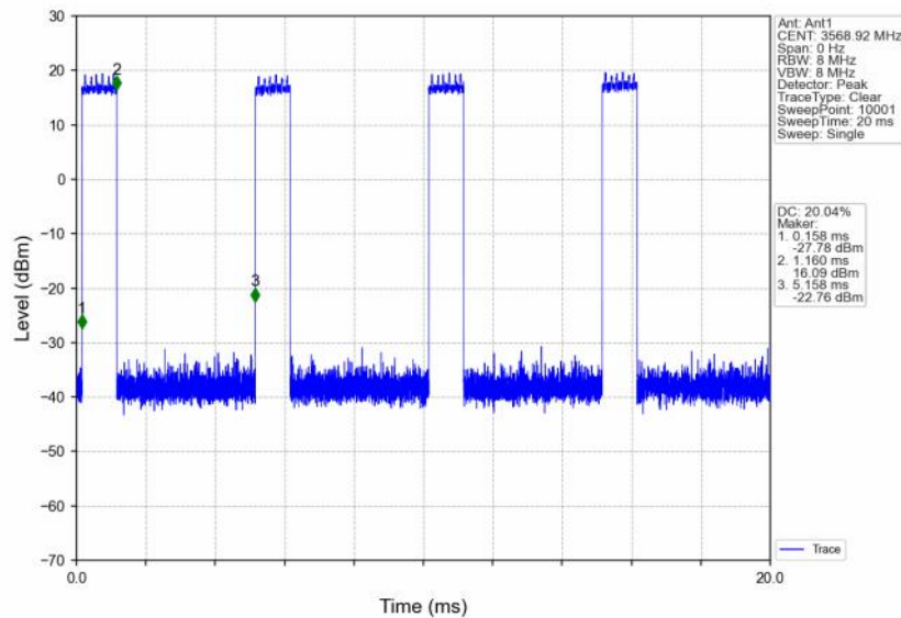
n48_30kHz_SISO_NTNV_40MHz_DFT-s-OFDM_PI/2_BPSK_3570MHz_Inner_Full
