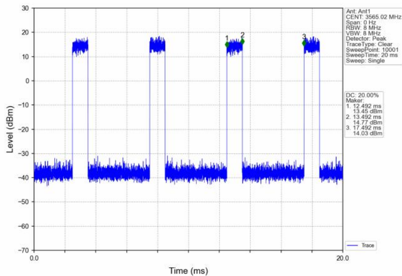
n48_30kHz_SISO_NTNV_30MHz_CP-OFDM 64 QAM_3565.02MHz_Inner_Full
