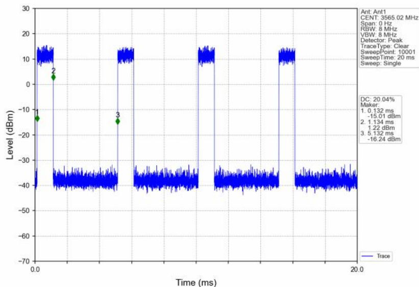
n48_30kHz_SISO_NTNV_30MHz_CP-OFDM 256 QAM_3565.02MHz_Inner_Full
