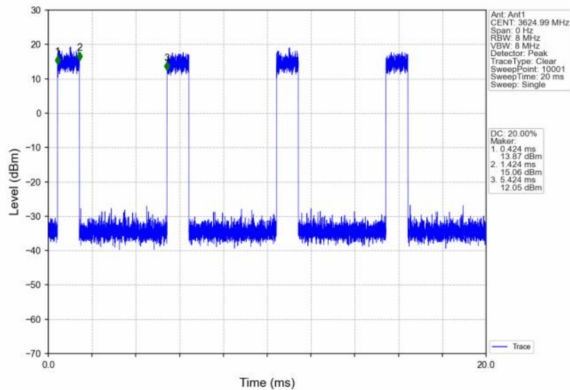
n48_30kHz_SISO_NTNV_30MHz_CP-OFDM 64 QAM_3624.99MHz_Inner_Full
