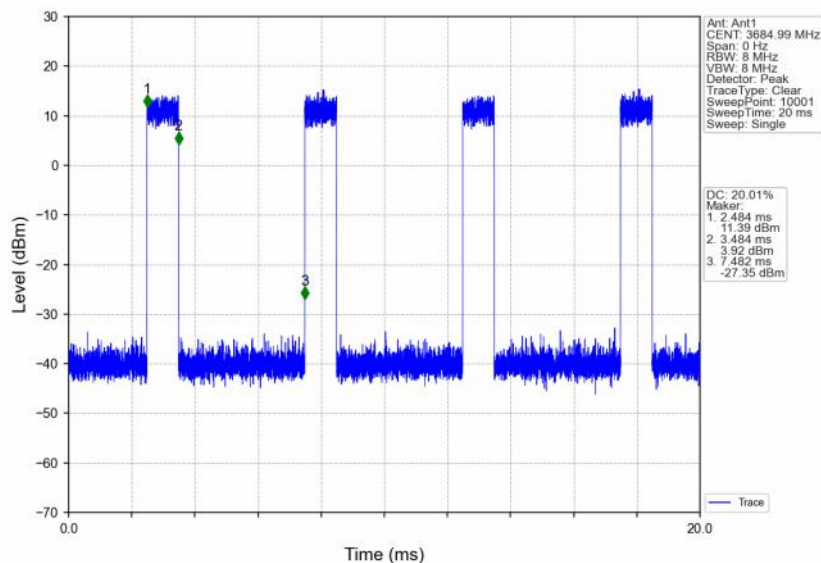
n48_30kHz_SISO_NTNV_30MHz_CP-OFDM 256 QAM_3684.99MHz_Inner_Full
