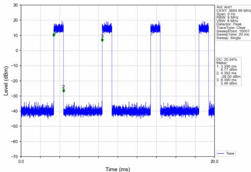
n48_30kHz_SISO_NTNV_30MHz_CP-OFDM_16_QAM_3684.99MHz_Inner_Full
