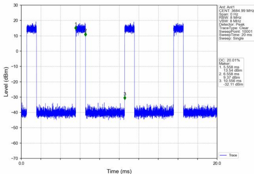
n48_30kHz_SISO_NTNV_30MHz_CP-OFDM QPSK_3684.99MHz_Inner_Full
