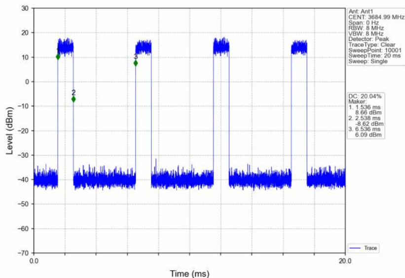
n48_30kHz_SISO_NTNV_30MHz_CP-OFDM 64 QAM_3684.99MHz_Inner_Full
