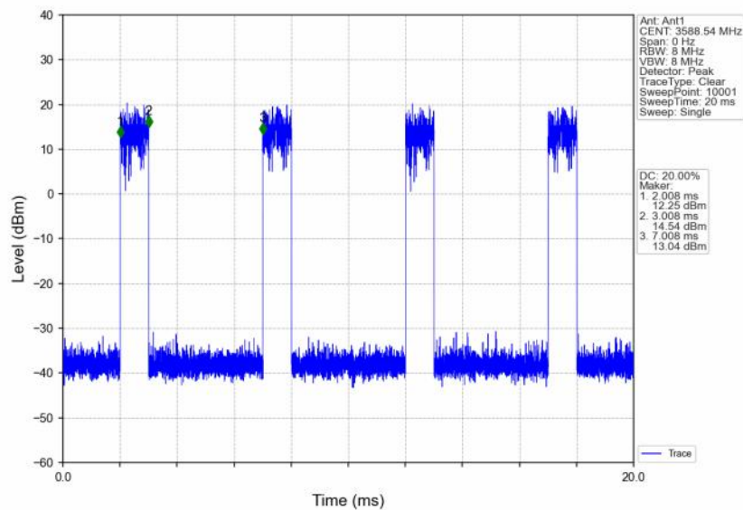
n48_30kHz_SISO_NTNV_40MHz_DFT-s-OFDM_256_QAM_3570MHz_Inner_1RB_Right
