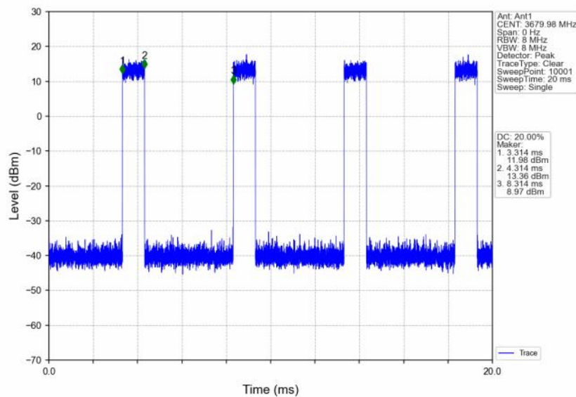
n48_30kHz_SISO_NTNV_40MHz_CP-OFDM_16_QAM_3679.98MHz_Inner_Full
