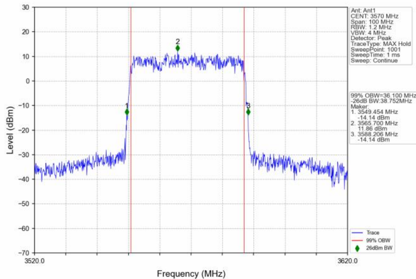
n48_30kHz_SISO_NTNV_40MHz_DFT-s-OFDM QPSK_3570MHz_Outer_Full
