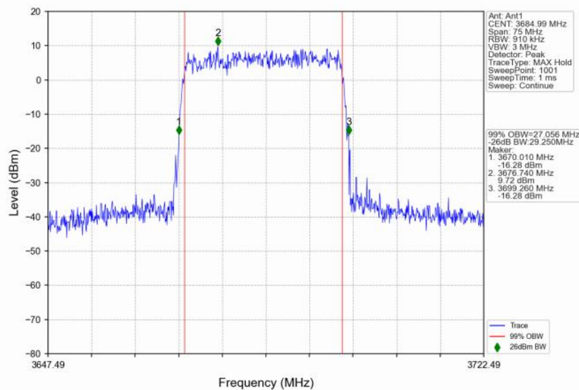
n48_30kHz_SISO_NTNV_30MHz_DFT-s-OFDM_64_QAM_3684.99MHz_Outer_Full
