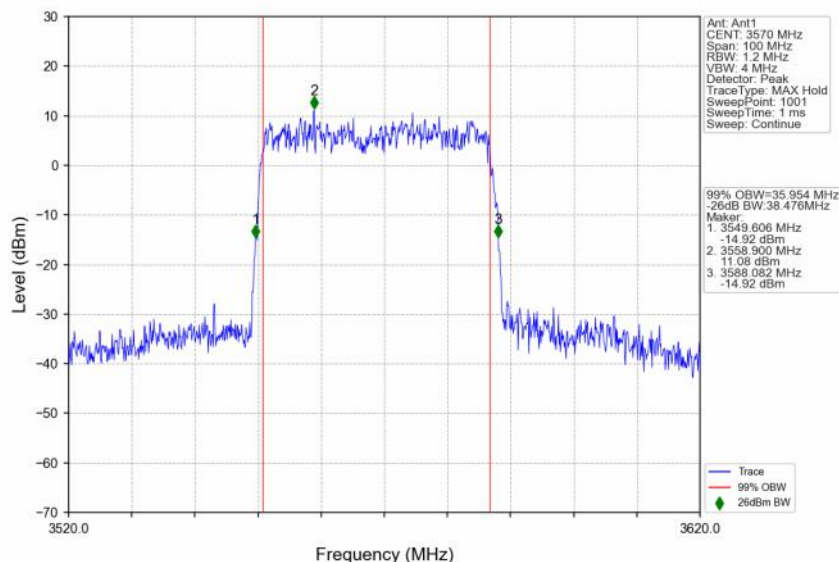
n48_30kHz_SISO_NTNV_40MHz_DFT-s-OFDM 64 QAM_3570MHz_Outer_Full
