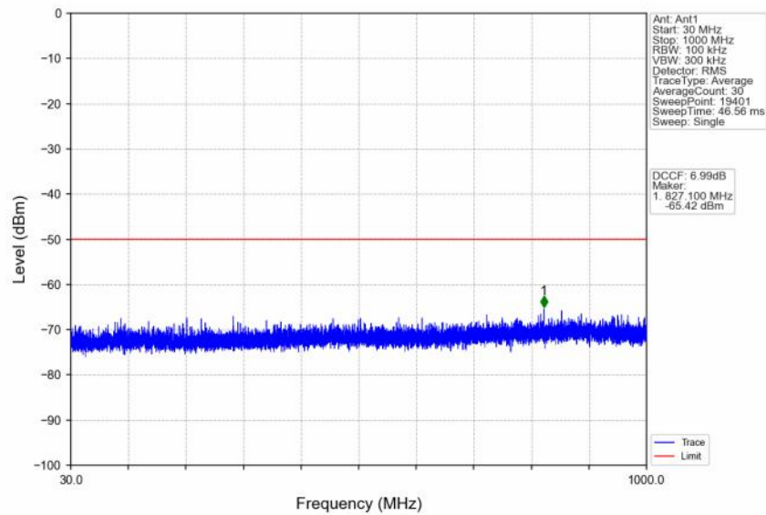
n48_30kHz_SISO_NTNV_10MHz_DFT-s-OFDM PI/2 BPSK_3624.99MHz_Edge_1RB_Left
