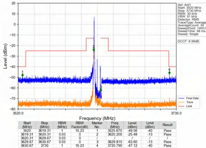
n48_30kHz_SISO_NTNV_10MHz_DFT-s-OFDM QPSK_3624.99MHz_Edge_1RB_Left
