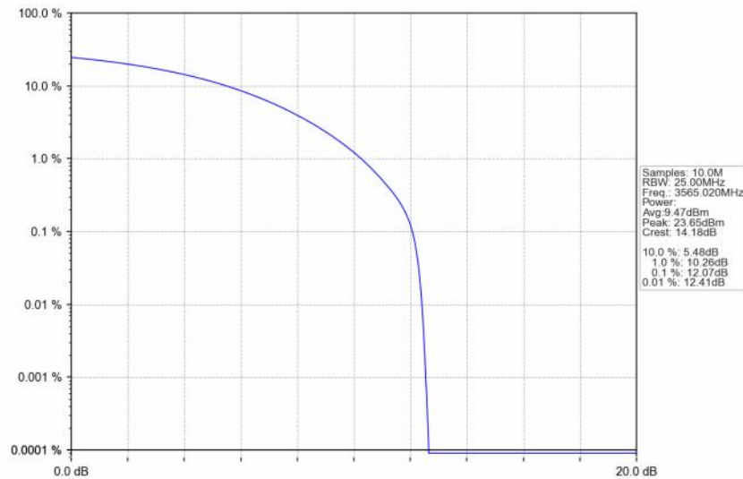
n48_30kHz_SISO_NTNV_30MHz_CP-OFDM_16_QAM_3565.02MHz_Outer_Full
