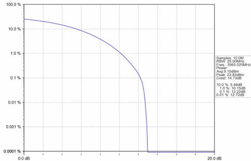
n48_30kHz_SISO_NTNV_30MHz_CP-OFDM_64_QAM_3565.02MHz_Outer_Full
