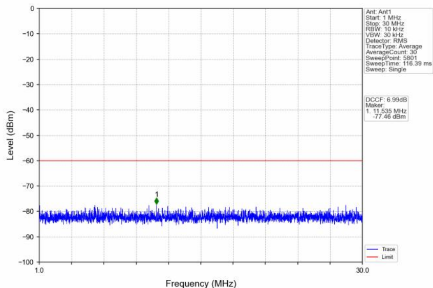
n48_30kHz_SISO_NTNV_10MHz_DFT-s-OFDM QPSK_3624.99MHz_Edge_1RB_Left
