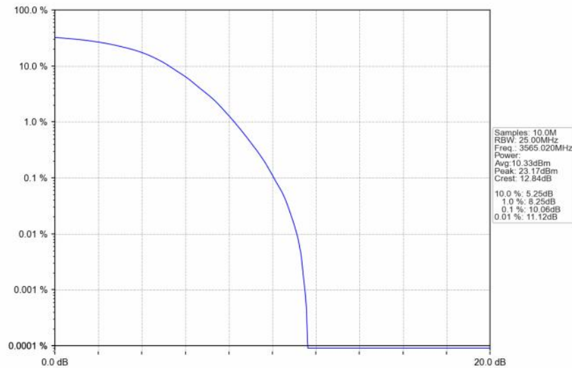
n48_30kHz_SISO_NTNV_30MHz_DFT-s-OFDM_64_QAM_3565.02MHz_Outer_Full
