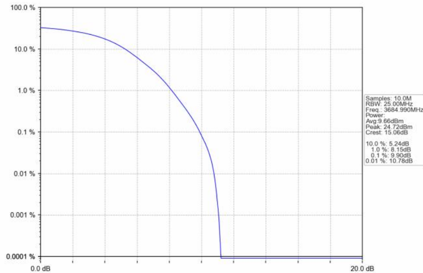
n48_30kHz_SISO_NTNV_30MHz_DFT-s-OFDM_64_QAM_3684.99MHz_Outer_Full
