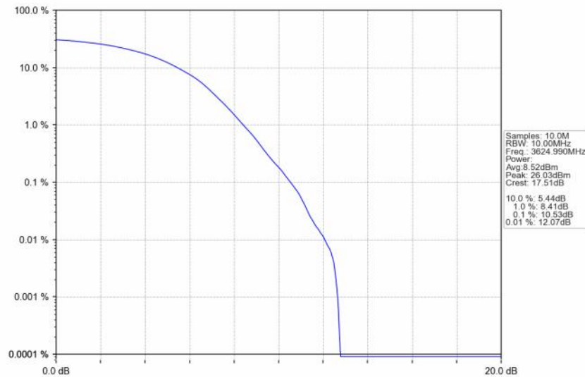
n48_30kHz_SISO_NTNV_10MHz_DFT-s-OFDM_256_QAM_3624.99MHz_Outer_Full
