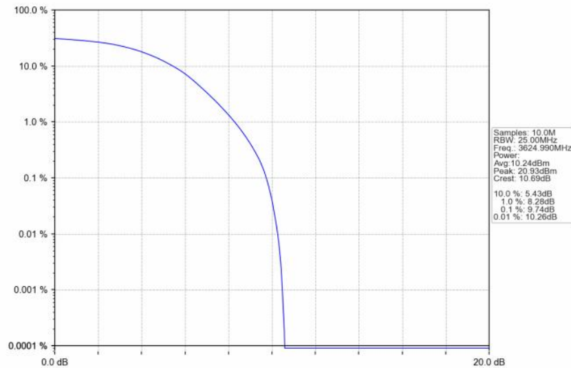
n48_30kHz_SISO_NTNV_30MHz_DFT-s-OFDM_16_QAM_3624.99MHz_Outer_Full
