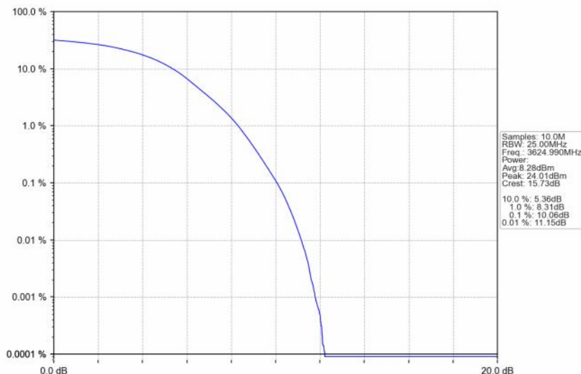
n48_30kHz_SISO_NTNV_30MHz_DFT-s-OFDM_256_QAM_3624.99MHz_Outer_Full
