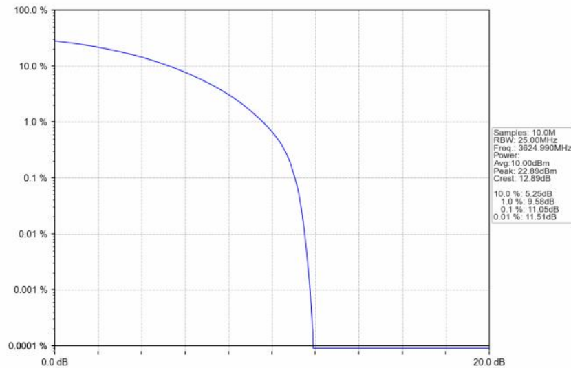
n48_30kHz_SISO_NTNV_30MHz_CP-OFDM QPSK_3624.99MHz_Outer_Full
