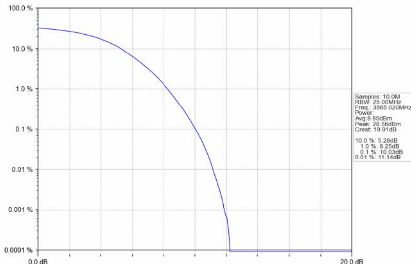
n48_30kHz_SISO_NTNV_30MHz_DFT-s-OFDM_256_QAM_3565.02MHz_Outer_Full
