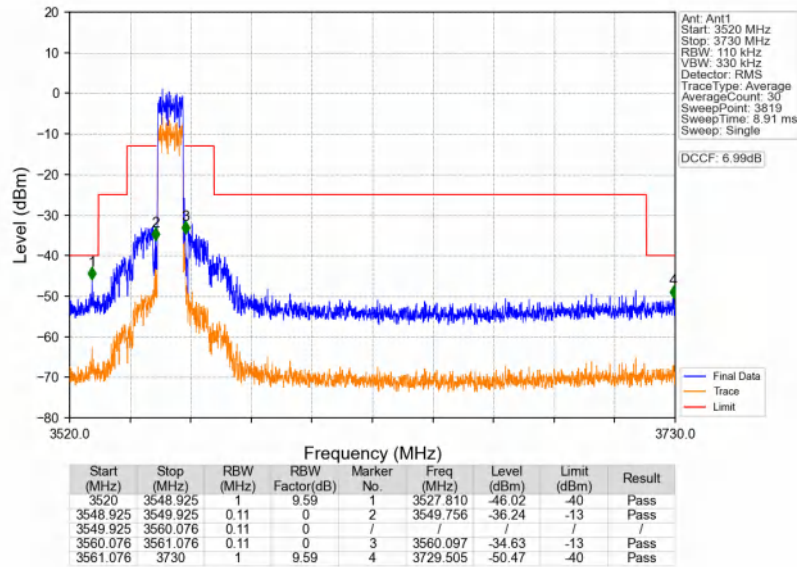
n48_30kHz_SISO_NTNV_10MHz_DFT-s-OFDM QPSK_3555MHz_Outer_Full
