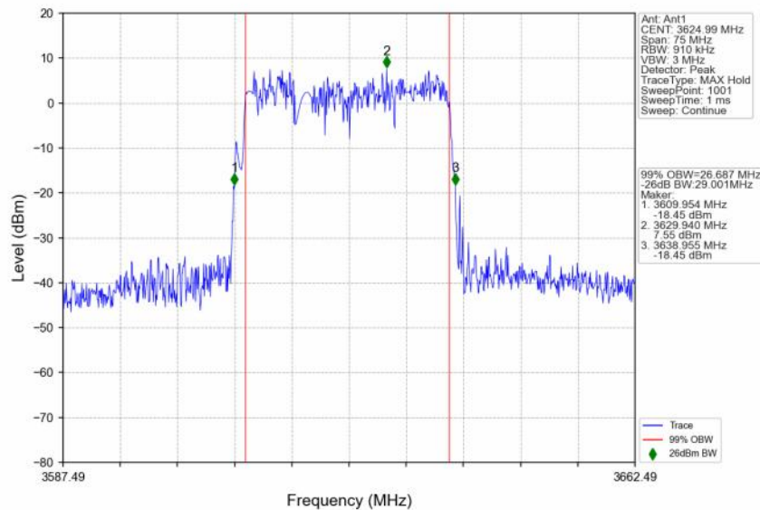
n48_30kHz_SISO_NTNV_30MHz_DFT-s-OFDM 256 QAM_3624.99MHz_Outer_Full
