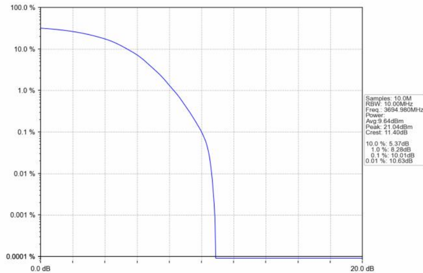
n48_30kHz_SISO_NTNV_10MHz_DFT-s-OFDM_64_QAM_3694.98MHz_Outer_Full
