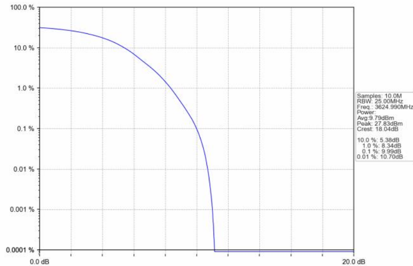
n48_30kHz_SISO_NTNV_30MHz_DFT-s-OFDM_64_QAM_3624.99MHz_Outer_Full
