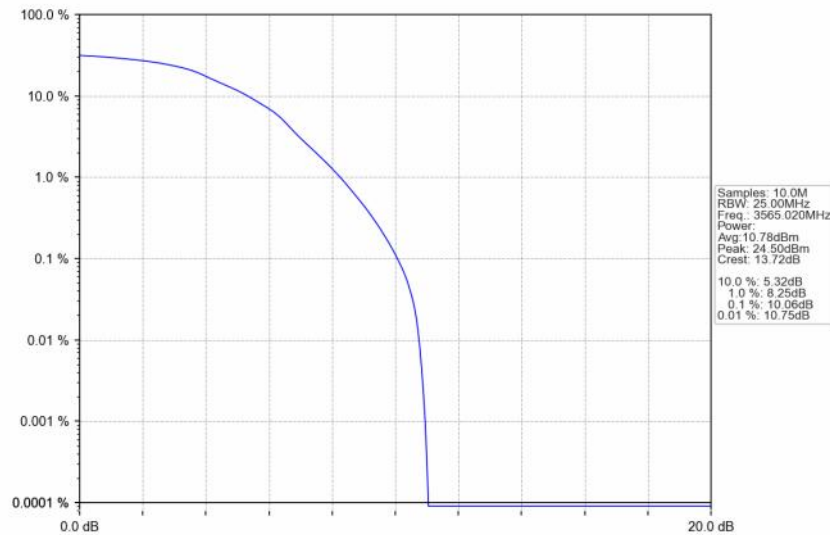
n48_30kHz_SISO_NTNV_30MHz_DFT-s-OFDM_16_QAM_3565.02MHz_Outer_Full
