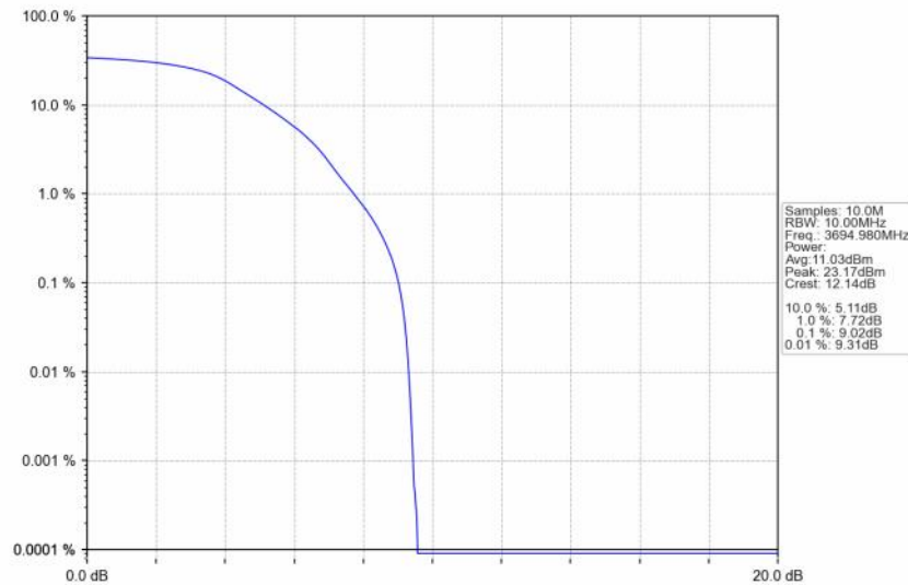
n48_30kHz_SISO_NTNV_10MHz_DFT-s-OFDM QPSK_3694.98MHz_Outer_Full
