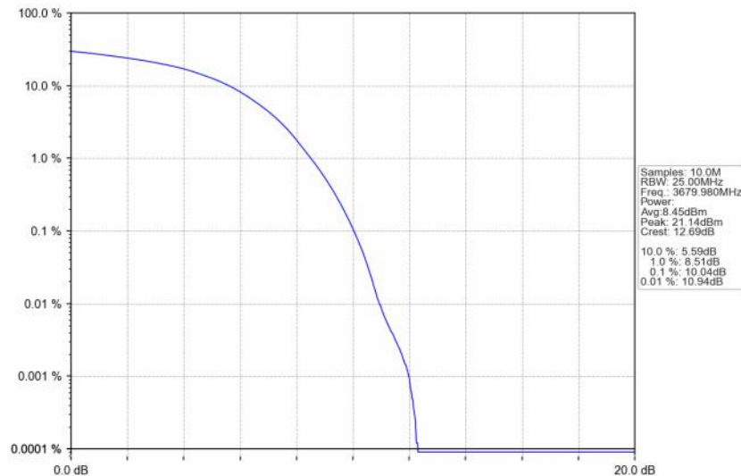
n48_30kHz_SISO_NTNV_40MHz_DFT-s-OFDM_64_QAM_3679.98MHz_Outer_Full
