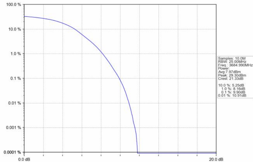
n48_30kHz_SISO_NTNV_30MHz_DFT-s-OFDM 256 QAM_3684.99MHz_Outer_Full
