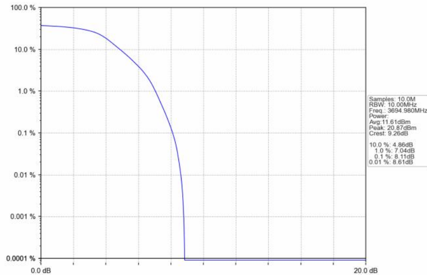
n48_30kHz_SISO_NTNV_10MHz_DFT-s-OFDM PI/2 BPSK_3694.98MHz_Outer_Full
