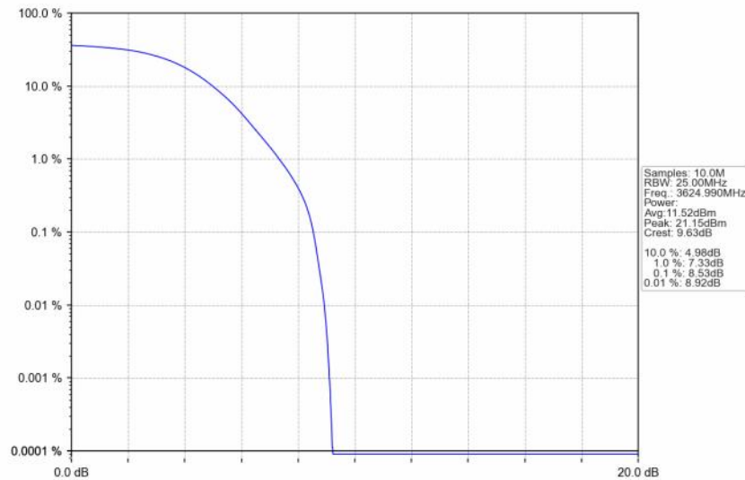
n48_30kHz_SISO_NTNV_30MHz_DFT-s-OFDM QPSK_3624.99MHz_Outer_Full
