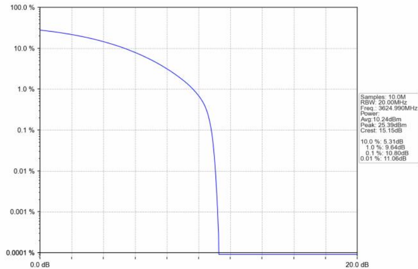
n48_30kHz_SISO_NTNV_20MHz_CP-OFDM QPSK_3624.99MHz_Outer_Full
