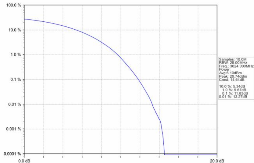
n48_30kHz_SISO_NTNV_30MHz_CP-OFDM 256 QAM_3624.99MHz_Outer_Full
