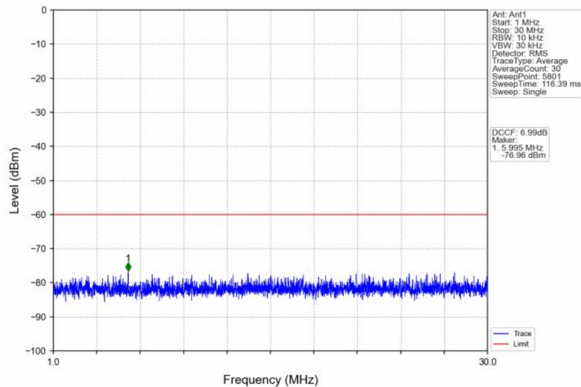
n48_30kHz_SISO_NTNV_10MHz_DFT-s-OFDM_PI/2_BPSK_3555MHz_Outer_Full
