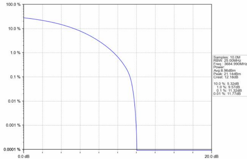
n48_30kHz_SISO_NTNV_30MHz_CP-OFDM_64_QAM_3684.99MHz_Outer_Full
