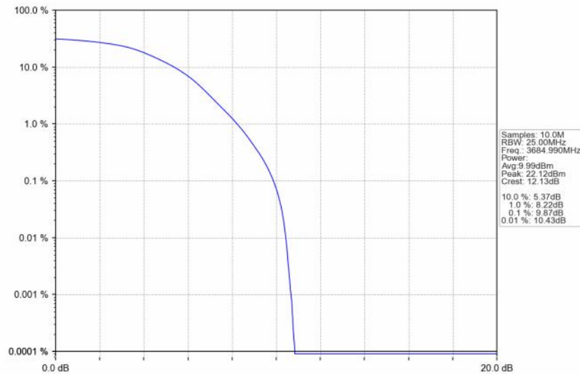
n48_30kHz_SISO_NTNV_30MHz_DFT-s-OFDM_16_QAM_3684.99MHz_Outer_Full
