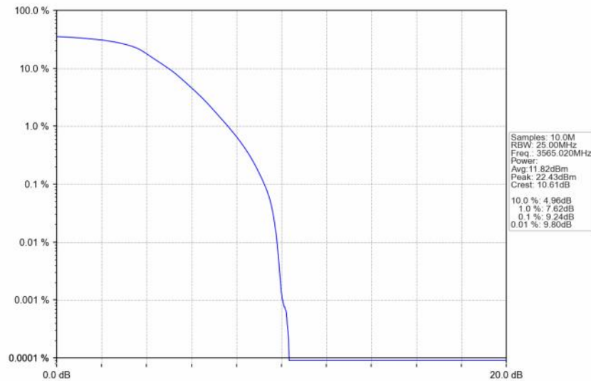
n48_30kHz_SISO_NTNV_30MHz_DFT-s-OFDM QPSK_3565.02MHz_Outer_Full
