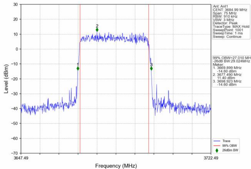
n48_30kHz_SISO_NTNV_30MHz_DFT-s-OFDM QPSK_3684.99MHz_Outer_Full
