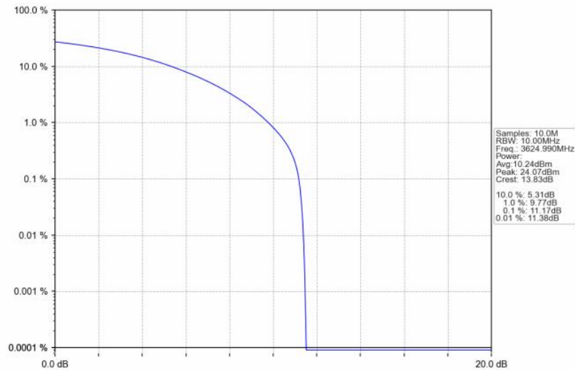
n48_30kHz_SISO_NTNV_10MHz_CP-OFDM_16_QAM_3624.99MHz_Outer_Full
