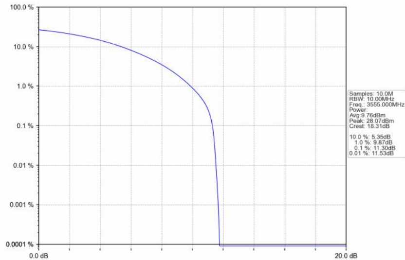
n48_30kHz_SISO_NTNV_10MHz_CP-OFDM_16_QAM_3555MHz_Outer_Full
