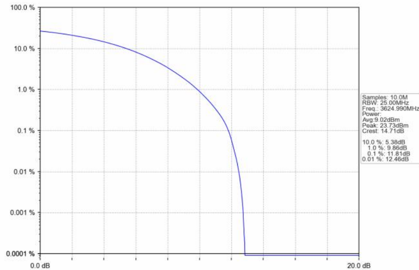
n48_30kHz_SISO_NTNV_30MHz_CP-OFDM_64_QAM_3624.99MHz_Outer_Full
