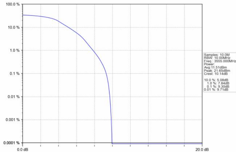
n48_30kHz_SISO_NTNV_10MHz_DFT-s-OFDM QPSK_3555MHz_Outer_Full
