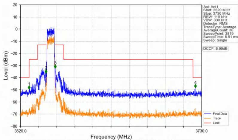
n48_30kHz_SISO_NTNV_10MHz_DFT-s-OFDM PI/2 BPSK_3555MHz_Outer_Full
