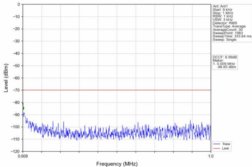
n48_30kHz_SISO_NTNV_10MHz_DFT-s-OFDM QPSK_3555MHz_Outer_Full
