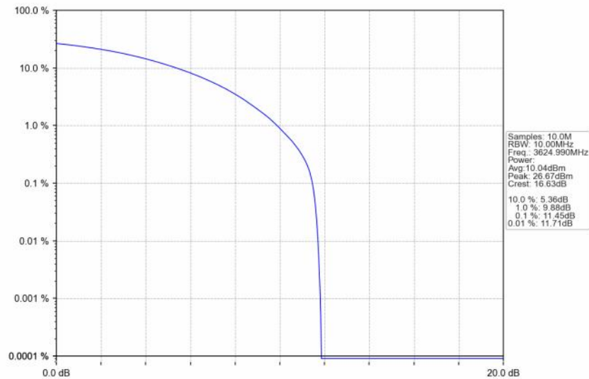
n48_30kHz_SISO_NTNV_10MHz_CP-OFDM QPSK_3624.99MHz_Outer_Full
