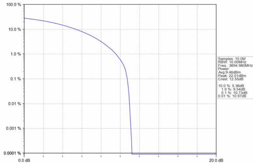
n48_30kHz_SISO_NTNV_10MHz_CP-OFDM QPSK_3694.98MHz_Outer_Full
