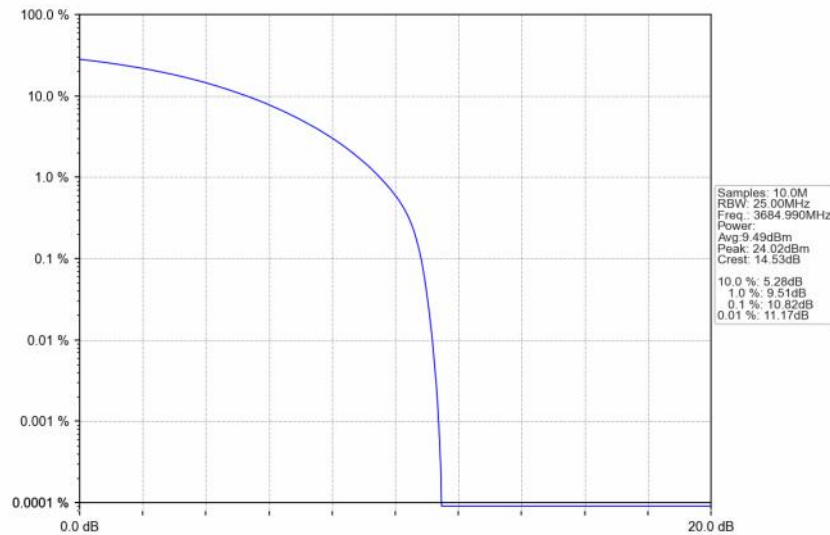
n48_30kHz_SISO_NTNV_30MHz_CP-OFDM QPSK_3684.99MHz_Outer_Full
