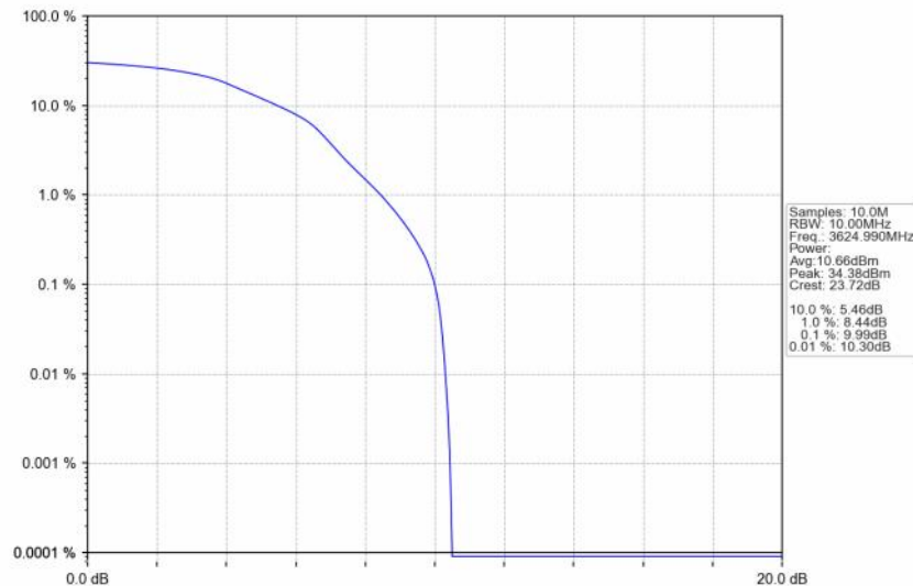
n48_30kHz_SISO_NTNV_10MHz_DFT-s-OFDM_16_QAM_3624.99MHz_Outer_Full
