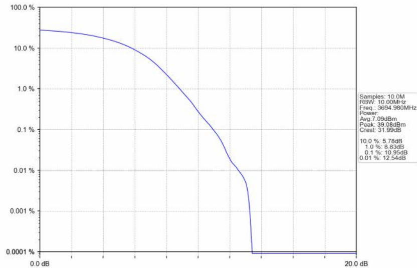
n48_30kHz_SISO_NTNV_10MHz_DFT-s-OFDM 256 QAM_3694.98MHz_Outer_Full
