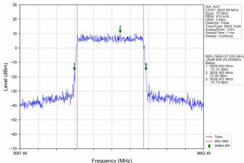
n48_30kHz_SISO_NTNV_30MHz_DFT-s-OFDM_16_QAM_3624.99MHz_Outer_Full
