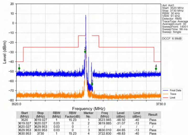
n48_30kHz_SISO_NTNV_10MHz_DFT-s-OFDM PI/2 BPSK_3624.99MHz_Edge_1RB_Left
