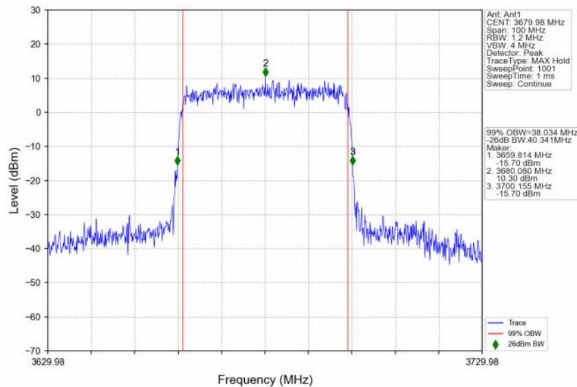
n48_30kHz_SISO_NTNV_40MHz_CP-OFDM QPSK_3679.98MHz_Outer_Full
