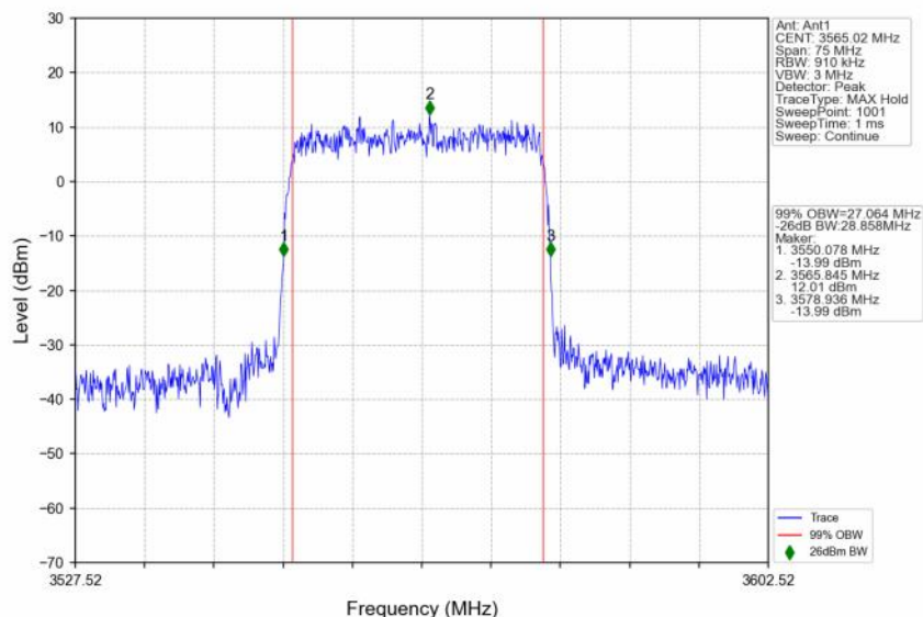
n48_30kHz_SISO_NTNV_30MHz_DFT-s-OFDM QPSK_3565.02MHz_Outer_Full
