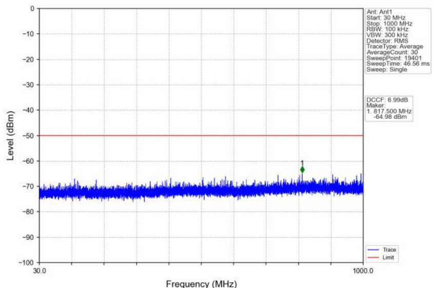
n48_30kHz_SISO_NTNV_10MHz_DFT-s-OFDM QPSK_3555MHz_Outer_Full
