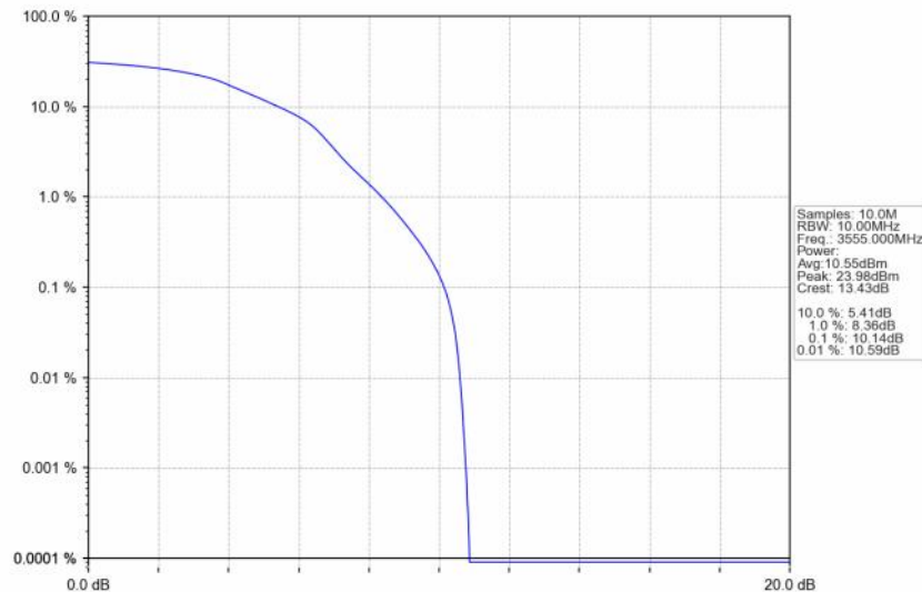
n48_30kHz_SISO_NTNV_10MHz_DFT-s-OFDM_16_QAM_3555MHz_Outer_Full
