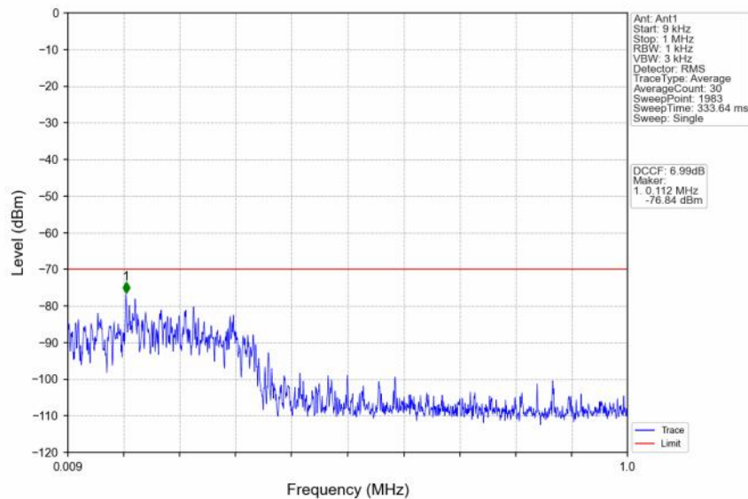
n48_30kHz_SISO_NTNV_10MHz_DFT-s-OFDM QPSK_3624.99MHz_Edge_1RB_Left
