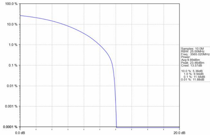
n48_30kHz_SISO_NTNV_30MHz_CP-OFDM QPSK_3565.02MHz_Outer_Full
