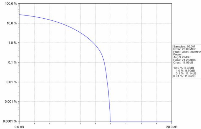
n48_30kHz_SISO_NTNV_30MHz_CP-OFDM_16_QAM_3684.99MHz_Outer_Full
