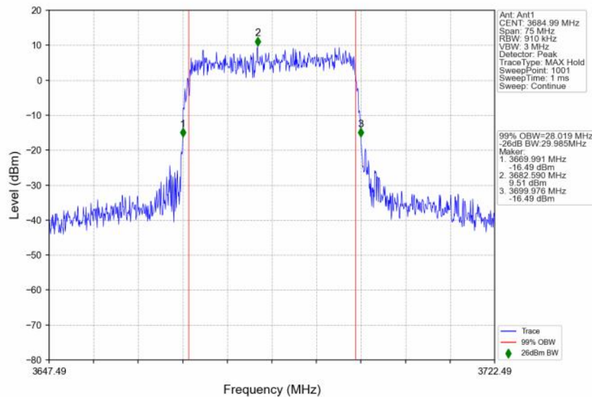
n48_30kHz_SISO_NTNV_30MHz_CP-OFDM QPSK_3684.99MHz_Outer_Full
