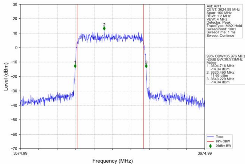
n48_30kHz_SISO_NTNV_40MHz_DFT-s-OFDM_16_QAM_3624.99MHz_Outer_Full
