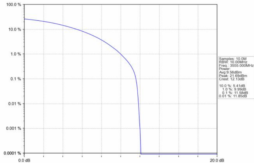
n48_30kHz_SISO_NTNV_10MHz_CP-OFDM QPSK_3555MHz_Outer_Full
