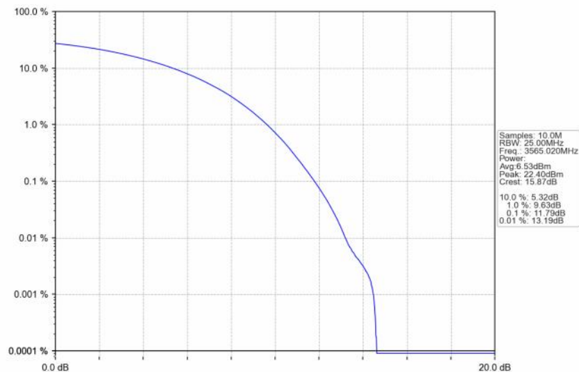
n48_30kHz_SISO_NTNV_30MHz_CP-OFDM 256 QAM_3565.02MHz_Outer_Full
