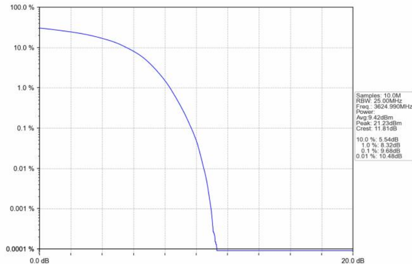
n48_30kHz_SISO_NTNV_40MHz_DFT-s-OFDM_16_QAM_3624.99MHz_Outer_Full
