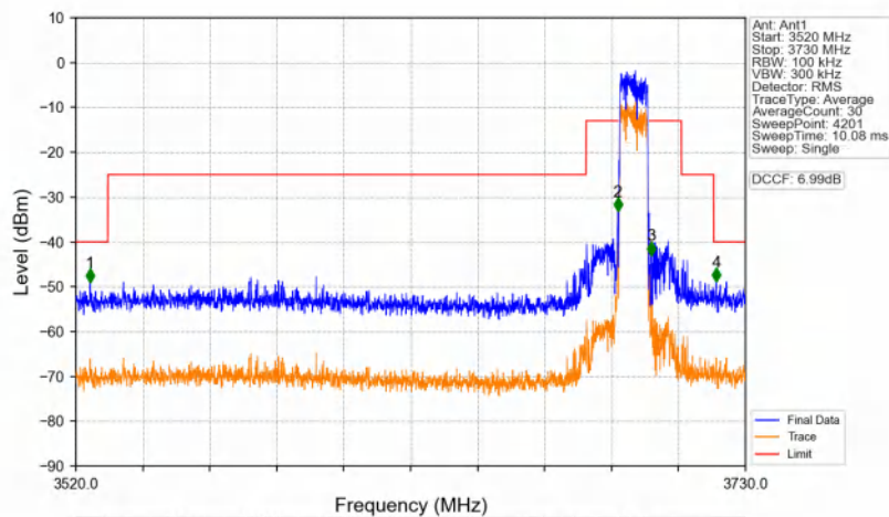
n48_30kHz_SISO_NTNV_10MHz_DFT-s-OFDM PI/2 BPSK_3694.98MHz_Outer_Full
