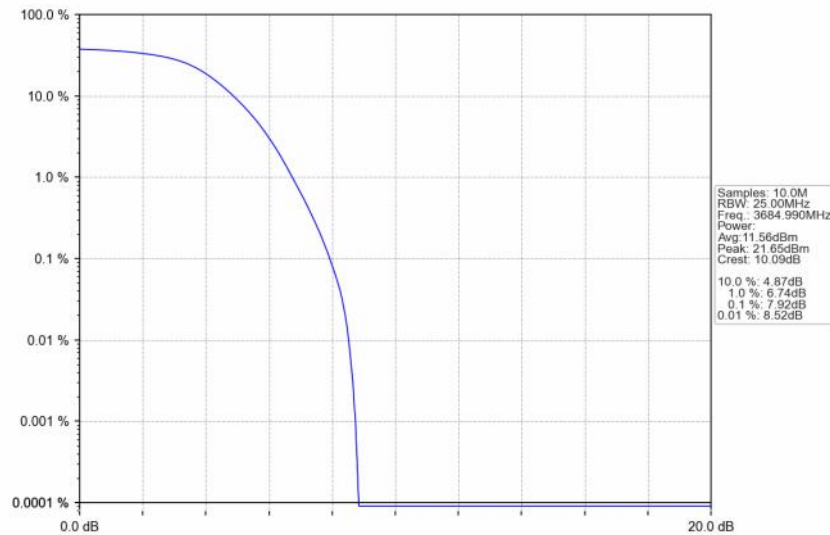
n48_30kHz_SISO_NTNV_30MHz_DFT-s-OFDM PI/2 BPSK_3684.99MHz_Outer_Full
