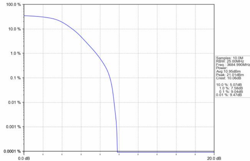
n48_30kHz_SISO_NTNV_30MHz_DFT-s-OFDM QPSK_3684.99MHz_Outer_Full
