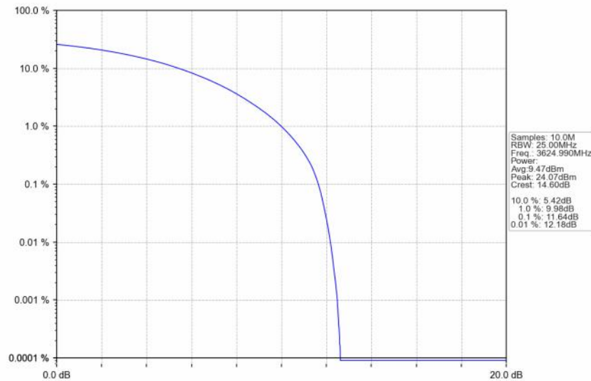
n48_30kHz_SISO_NTNV_30MHz_CP-OFDM_16_QAM_3624.99MHz_Outer_Full
