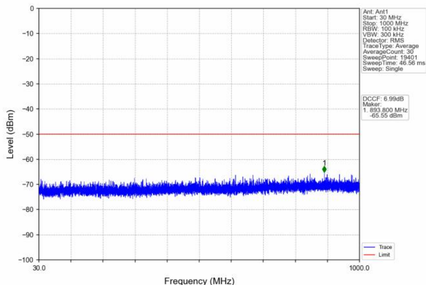
n48_30kHz_SISO_NTNV_10MHz_DFT-s-OFDM QPSK_3624.99MHz_Edge_1RB_Left
