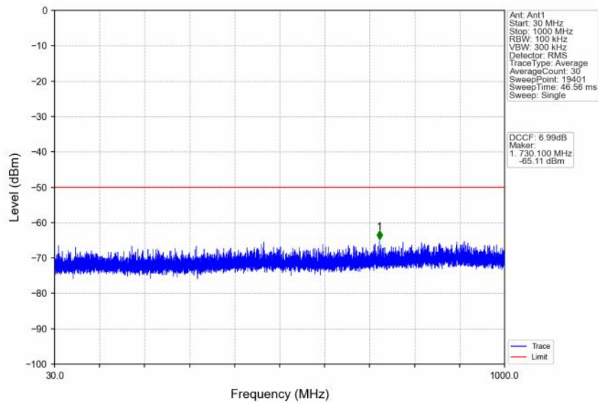
n48_30kHz_SISO_NTNV_30MHz_DFT-s-OFDM_PI/2_BPSK_3565.02MHz_Outer_Full
