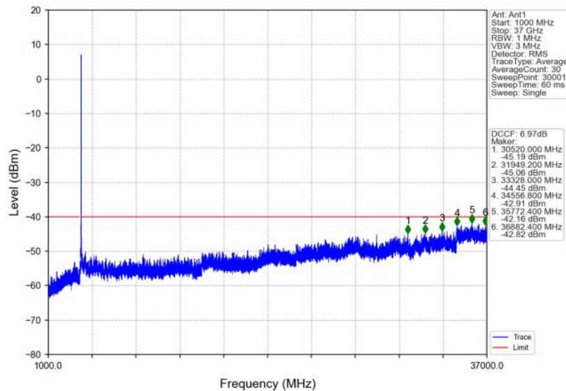
n48_30kHz_SISO_NTNV_20MHz_DFT-s-OFDM_PI/2_BPSK_3690MHz_Outer_Full
