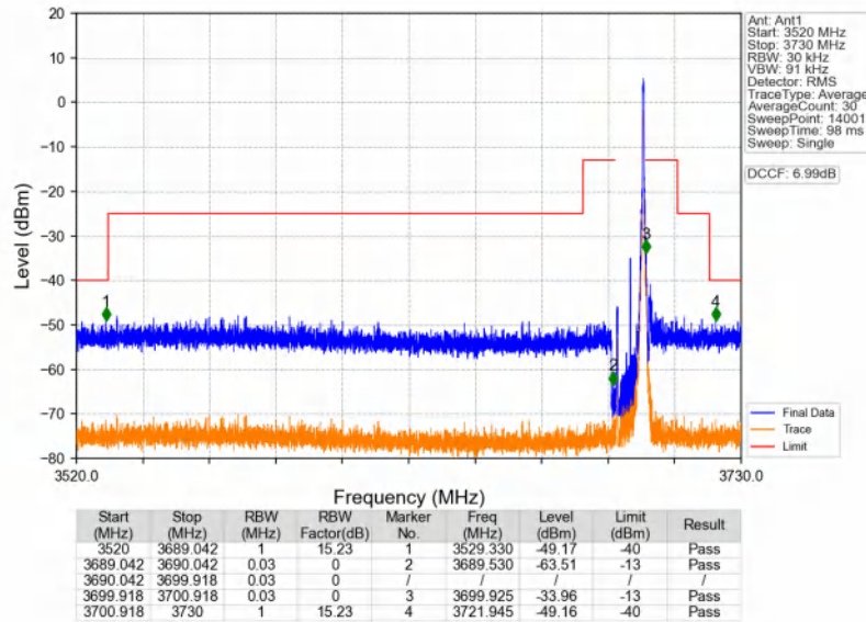
n48_30kHz_SISO_NTNV_10MHz_CP-OFDM QPSK_3694.98MHz_Edge_1RB_Right
