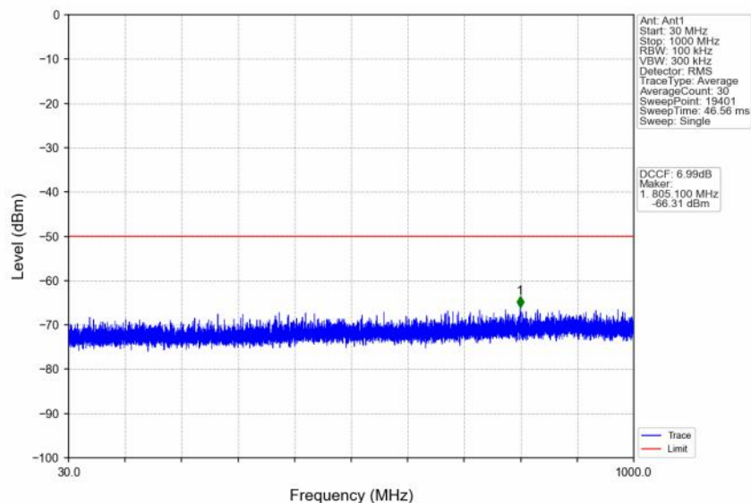
n48_30kHz_SISO_NTNV_10MHz_DFT-s-OFDM QPSK_3694.98MHz_Inner_1RB_Right
