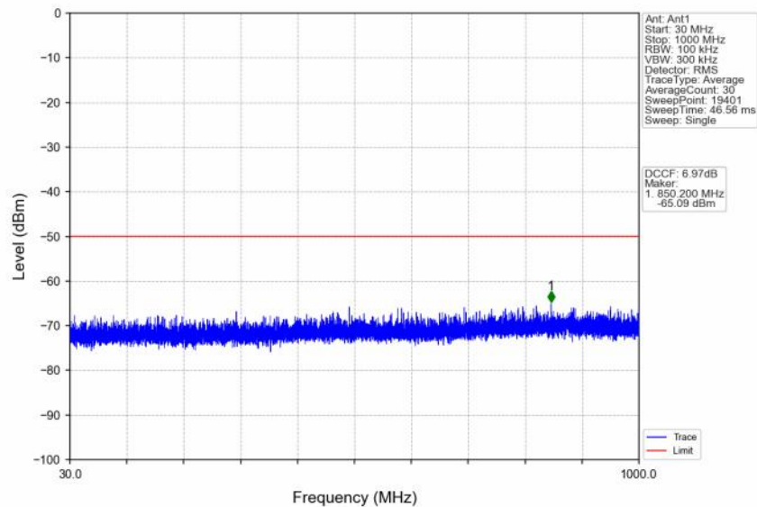
n48_30kHz_SISO_NTNV_20MHz_DFT-s-OFDM_PI/2_BPSK_3690MHz_Outer_Full
