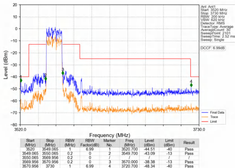
n48_30kHz_SISO_NTNV_20MHz_DFT-s-OFDM PI/2 BPSK_3560.01MHz_Outer_Full
