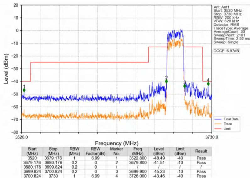
n48_30kHz_SISO_NTNV_20MHz_DFT-s-OFDM PI/2 BPSK_3690MHz_Outer_Full
