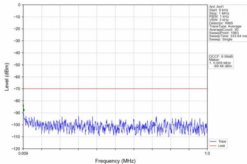
n48_30kHz_SISO_NTNV_10MHz_CP-OFDM QPSK_3694.98MHz_Outer_Full
