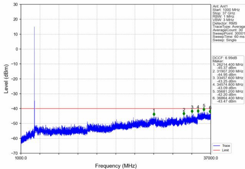
n48_30kHz_SISO_NTNV_30MHz_DFT-s-OFDM PI/2 BPSK_3624.99MHz_Edge_1RB_Left
