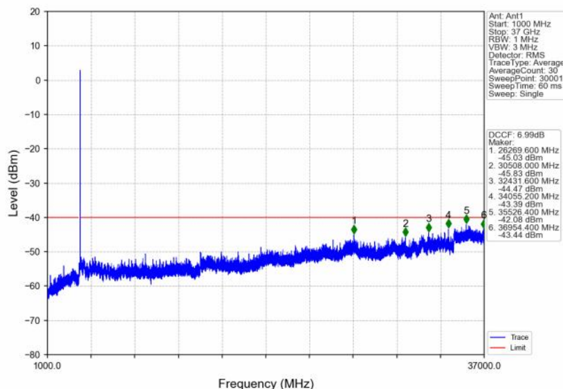
n48_30kHz_SISO_NTNV_10MHz_CP-OFDM QPSK_3694.98MHz_Outer_Full
