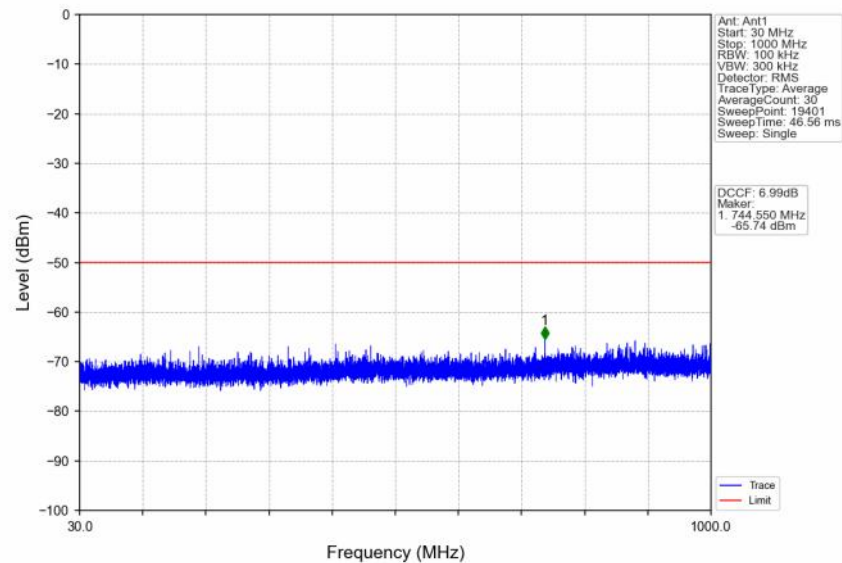
n48_30kHz_SISO_NTNV_10MHz_CP-OFDM QPSK_3694.98MHz_Edge_1RB_Right
