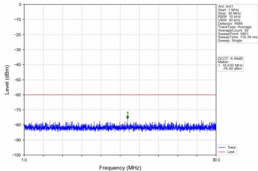
n48_30kHz_SISO_NTNV_10MHz_CP-OFDM QPSK_3694.98MHz_Edge_1RB_Right
