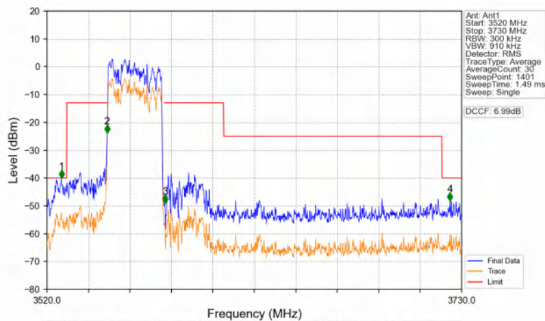
n48_30kHz_SISO_NTNV_30MHz_DFT-s-OFDM PI/2 BPSK_3565.02MHz_Outer_Full
