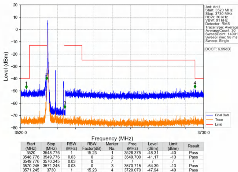
n48_30kHz_SISO_NTNV_20MHz_DFT-s-OFDM QPSK_3560.01MHz_Edge_1RB_Left
