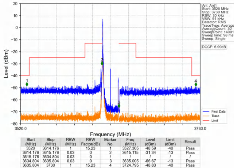
n48_30kHz_SISO_NTNV_20MHz_DFT-s-OFDM PI/2 BPSK_3624.99MHz_Edge_1RB_Left
