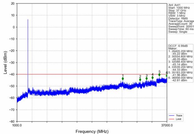
n48_30kHz_SISO_NTNV_10MHz_CP-OFDM QPSK_3624.99MHz_Edge_1RB_Left
