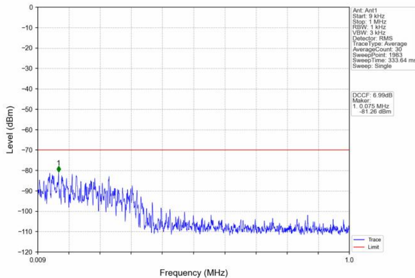
n48_30kHz_SISO_NTNV_10MHz_CP-OFDM QPSK_3694.98MHz_Edge_1RB_Right
