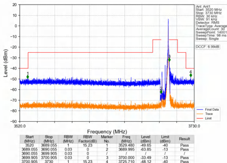
n48_30kHz_SISO_NTNV_10MHz_CP-OFDM QPSK_3694.98MHz_Inner_1RB_Right
