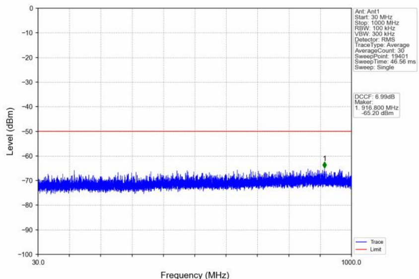
n48_30kHz_SISO_NTNV_20MHz_CP-OFDM QPSK_3690MHz_Edge_1RB_Right
