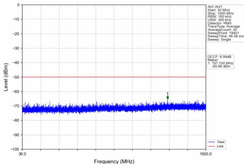
n48_30kHz_SISO_NTNV_10MHz_CP-OFDM QPSK_3694.98MHz_Outer_Full
