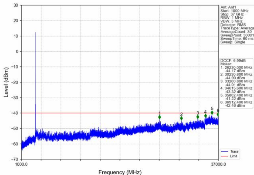
n48_30kHz_SISO_NTNV_30MHz_DFT-s-OFDM PI/2 BPSK_3565.02MHz_Outer_Full
