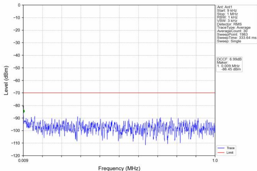
n48_30kHz_SISO_NTNV_10MHz_CP-OFDM QPSK_3555MHz_Outer_Full
