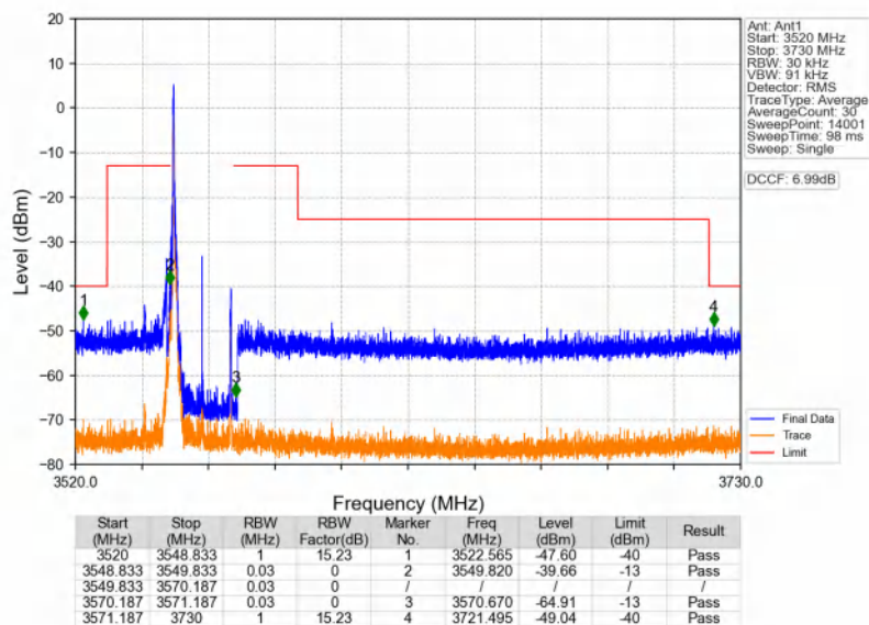
n48_30kHz_SISO_NTNV_20MHz_DFT-s-OFDM_PI/2_BPSK_3560.01MHz_Edge_1RB_Left
