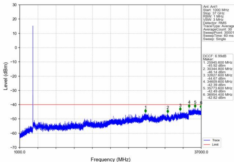
n48_30kHz_SISO_NTNV_10MHz_DFT-s-OFDM QPSK_3694.98MHz_Edge_1RB_Right
