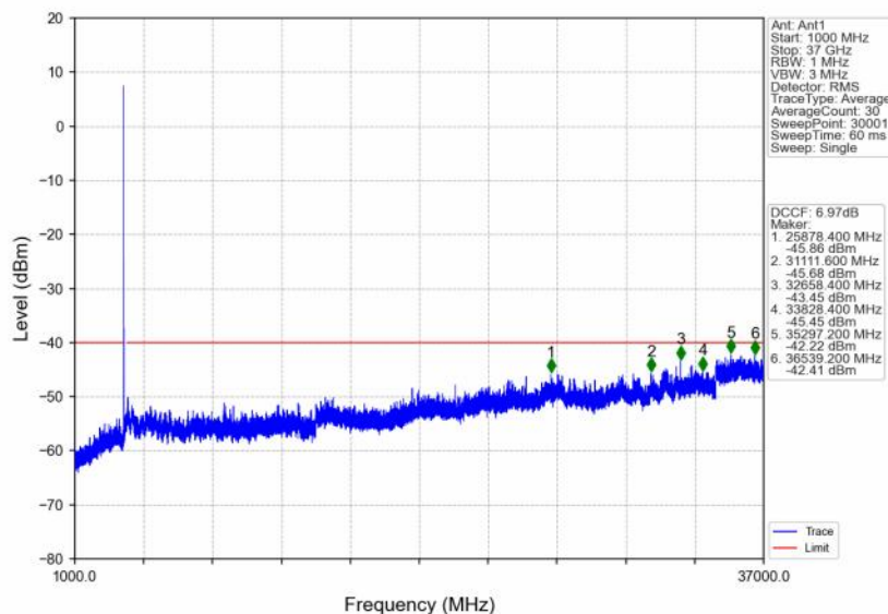
n48_30kHz_SISO_NTNV_10MHz_CP-OFDM QPSK_3555MHz_Outer_Full
