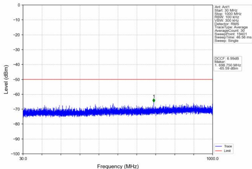
n48_30kHz_SISO_NTNV_10MHz_DFT-s-OFDM QPSK_3694.98MHz_Edge_1RB_Right
