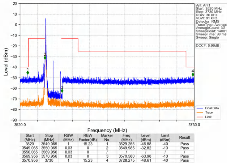
n48_30kHz_SISO_NTNV_20MHz_CP-OFDM QPSK_3560.01MHz_Edge_1RB_Left
