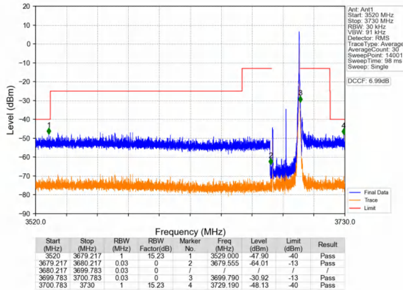
n48_30kHz_SISO_NTNV_20MHz_CP-OFDM QPSK_3690MHz_Edge_1RB_Right
