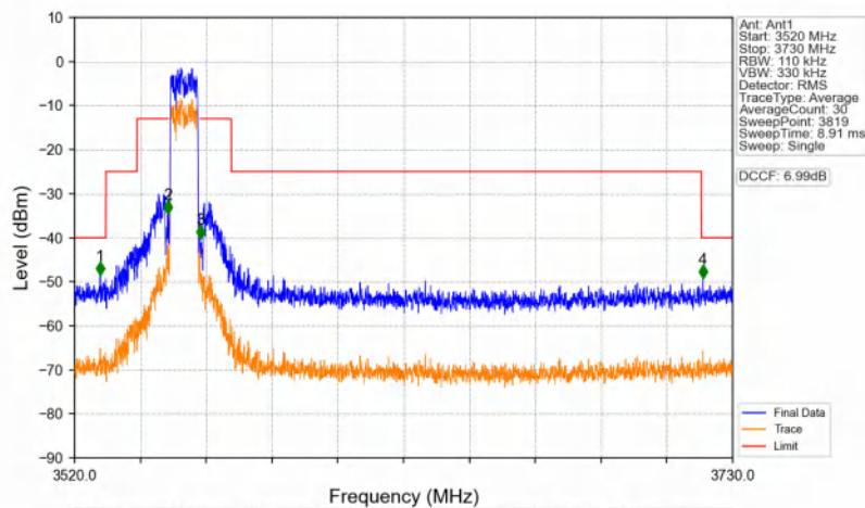
n48_30kHz_SISO_NTNV_10MHz_CP-OFDM QPSK_3555MHz_Outer_Full
