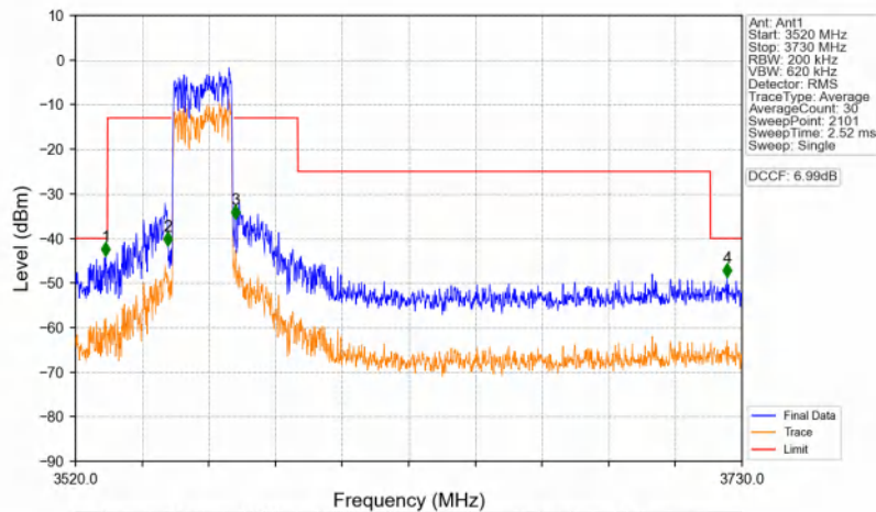
n48_30kHz_SISO_NTNV_20MHz_CP-OFDM QPSK_3560.01MHz_Outer_Full
