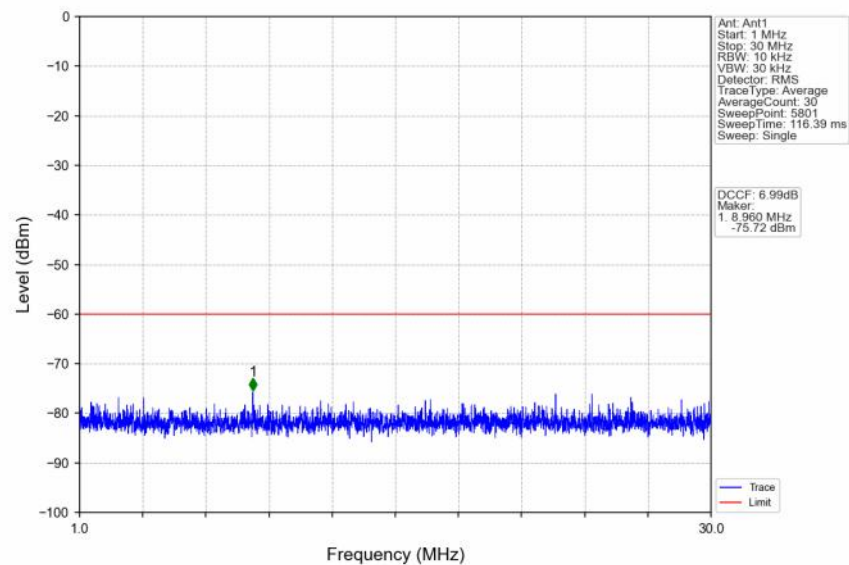
n48_30kHz_SISO_NTNV_10MHz_DFT-s-OFDM QPSK_3694.98MHz_Outer_Full
