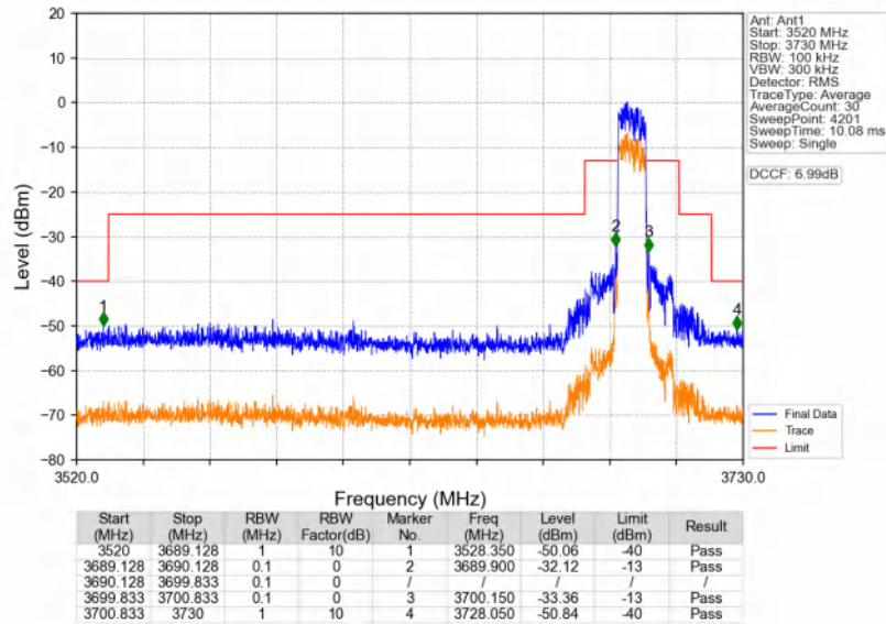
n48_30kHz_SISO_NTNV_10MHz_DFT-s-OFDM QPSK_3694.98MHz_Outer_Full
