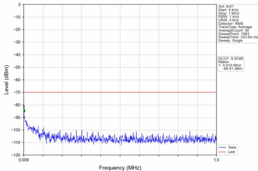
n48_30kHz_SISO_NTNV_20MHz_DFT-s-OFDM_PI/2_BPSK_3690MHz_Outer_Full
