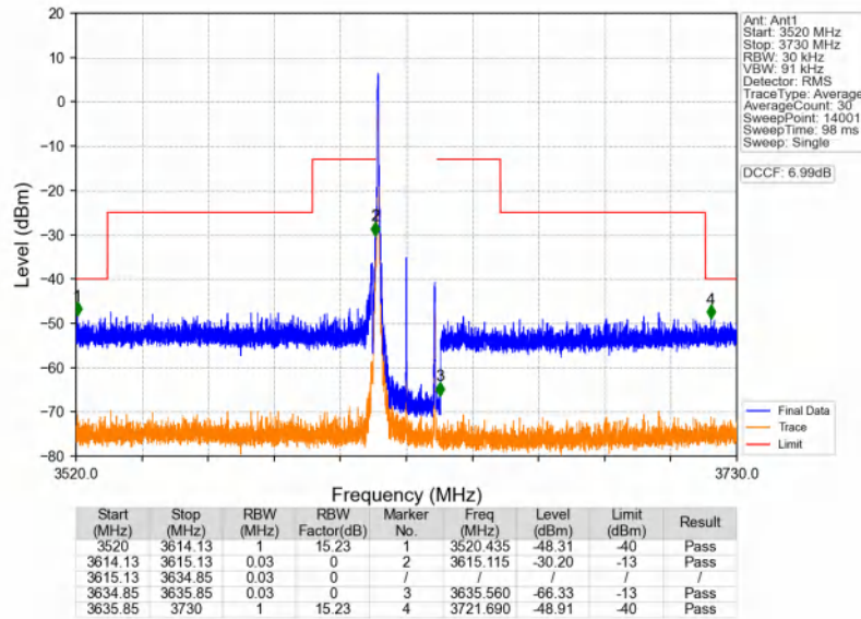
n48_30kHz_SISO_NTNV_20MHz_DFT-s-OFDM QPSK_3624.99MHz_Edge_1RB_Left
