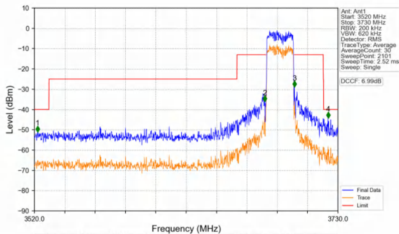
n48_30kHz_SISO_NTNV_20MHz_CP-OFDM QPSK_3690MHz_Outer_Full
