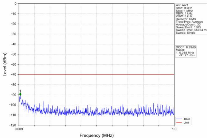
n48_30kHz_SISO_NTNV_10MHz_DFT-s-OFDM QPSK_3694.98MHz_Outer_Full
