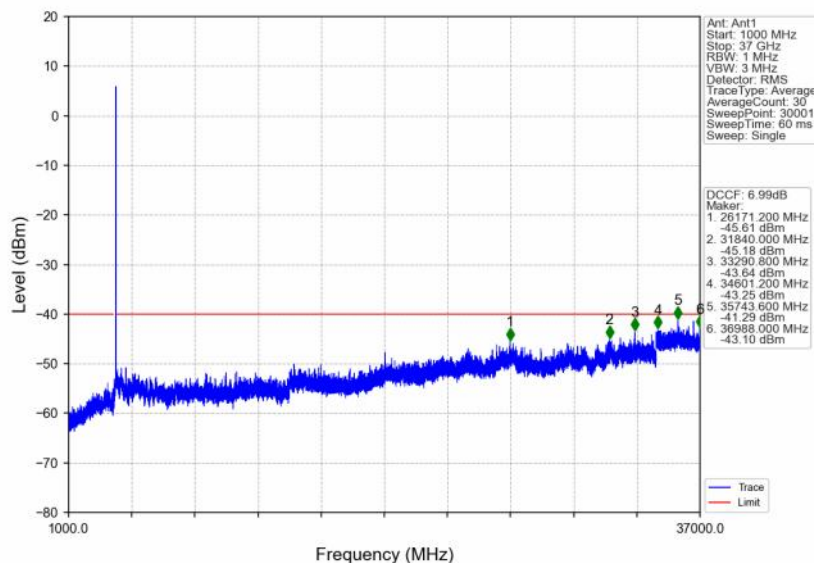
n48_30kHz_SISO_NTNV_10MHz_DFT-s-OFDM QPSK_3694.98MHz_Inner_1RB_Right
