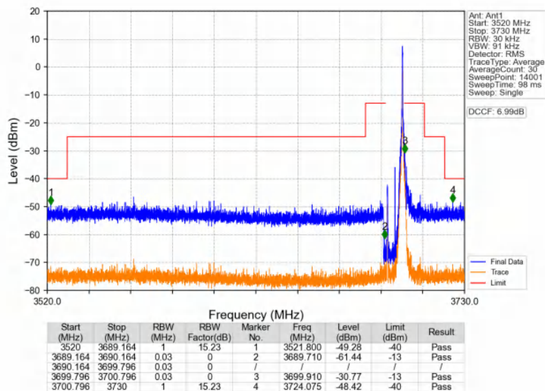
n48_30kHz_SISO_NTNV_10MHz_DFT-s-OFDM QPSK_3694.98MHz_Inner_1RB_Right
