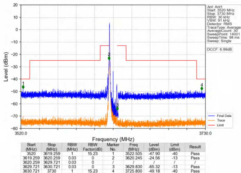
n48_30kHz_SISO_NTNV_10MHz_CP-OFDM QPSK_3624.99MHz_Edge_1RB_Left
