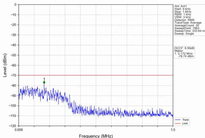
n48_30kHz_SISO_NTNV_10MHz_CP-OFDM QPSK_3694.98MHz_Inner_1RB_Right
