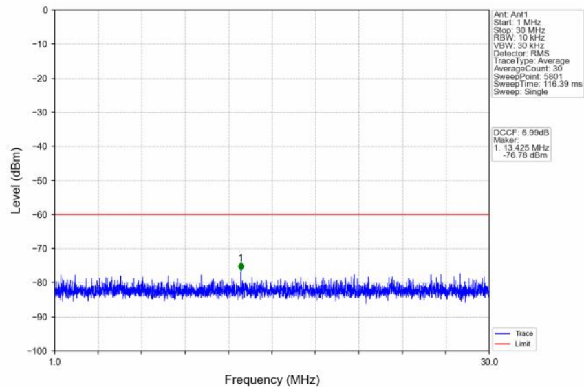
n48_30kHz_SISO_NTNV_10MHz_CP-OFDM QPSK_3624.99MHz_Edge_1RB_Left
