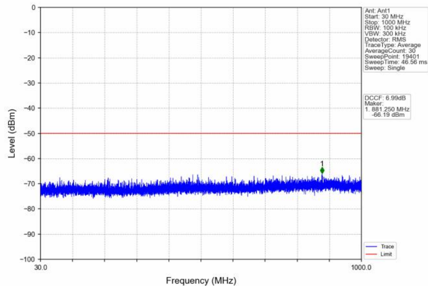
n48_30kHz_SISO_NTNV_10MHz_CP-OFDM QPSK_3624.99MHz_Edge_1RB_Left
