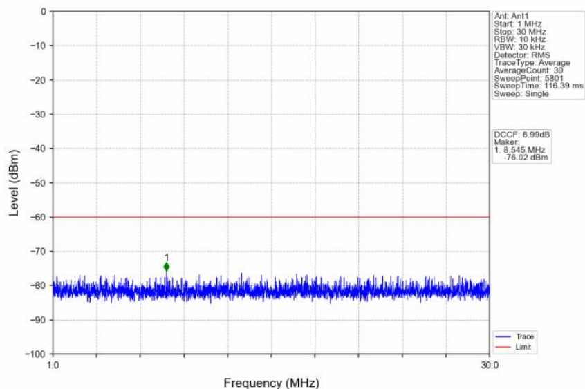
n48_30kHz_SISO_NTNV_30MHz_DFT-s-OFDM PI/2 BPSK_3565.02MHz_Inner_1RB_Left
