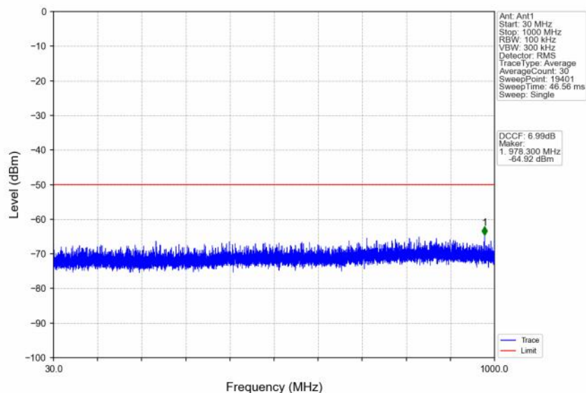
n48_30kHz_SISO_NTNV_30MHz_DFT-s-OFDM PI/2 BPSK_3624.99MHz_Edge_1RB_Left
