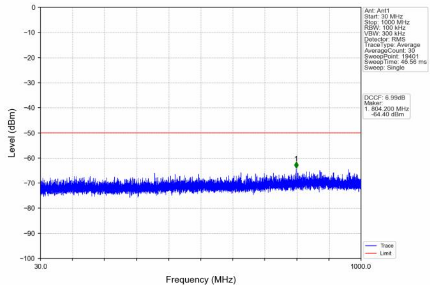
n48_30kHz_SISO_NTNV_20MHz_DFT-s-OFDM QPSK_3690MHz_Outer_Full
