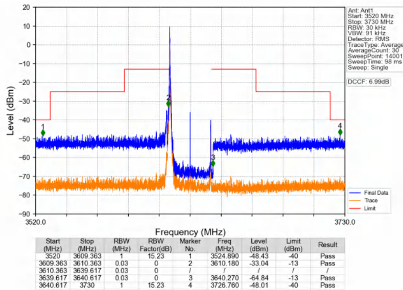
n48_30kHz_SISO_NTNV_30MHz_DFT-s-OFDM PI/2 BPSK_3624.99MHz_Edge_1RB_Left
