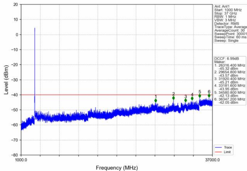
n48_30kHz_SISO_NTNV_30MHz_DFT-s-OFDM_PI/2_BPSK_3565.02MHz_Outer_Full
