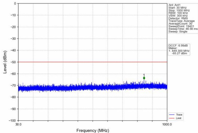
n48_30kHz_SISO_NTNV_10MHz_CP-OFDM QPSK_3555MHz_Outer_Full
