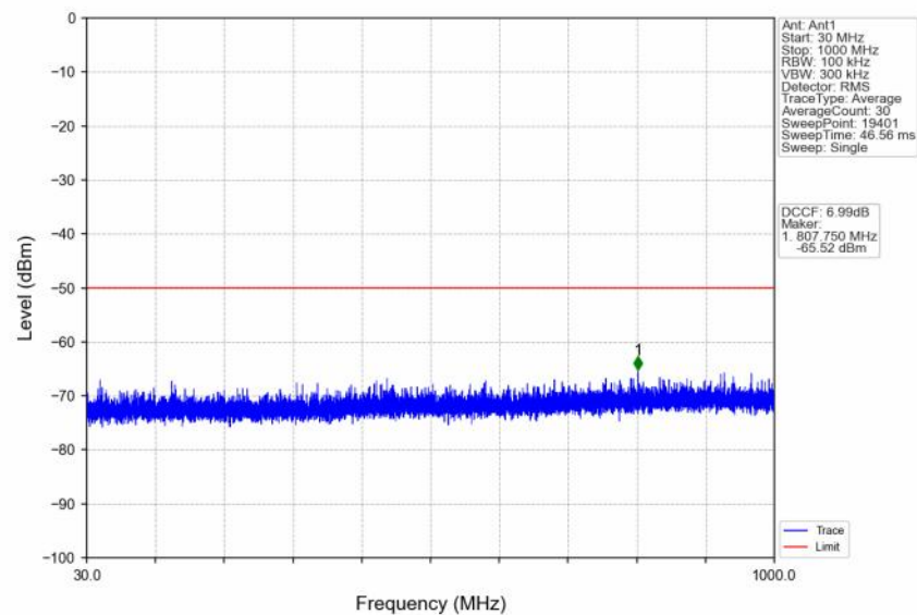
n48_30kHz_SISO_NTNV_10MHz_DFT-s-OFDM QPSK_3694.98MHz_Outer_Full
