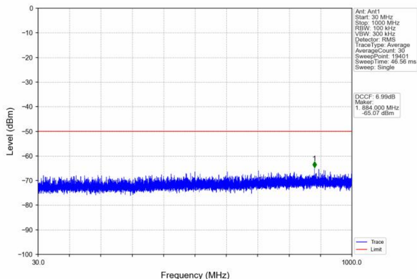
n48_30kHz_SISO_NTNV_20MHz_DFT-s-OFDM QPSK_3624.99MHz_Edge_1RB_Left
