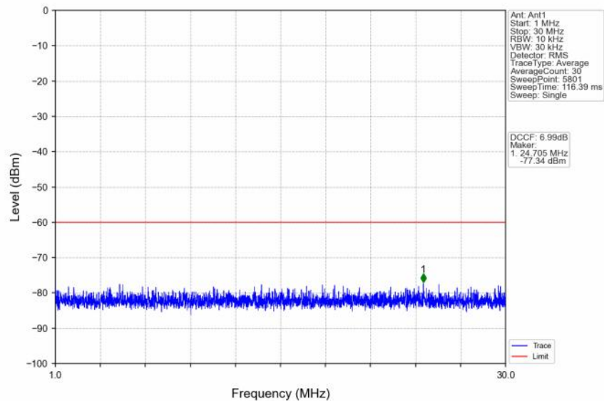
n48_30kHz_SISO_NTNV_10MHz_DFT-s-OFDM QPSK_3694.98MHz_Edge_1RB_Right
