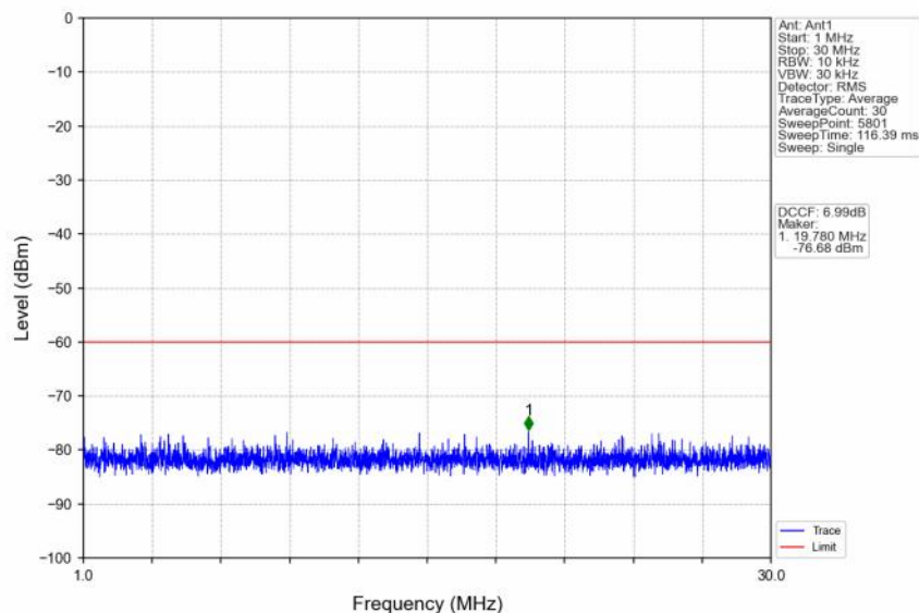
n48_30kHz_SISO_NTNV_10MHz_CP-OFDM QPSK_3694.98MHz_Inner_1RB_Right
