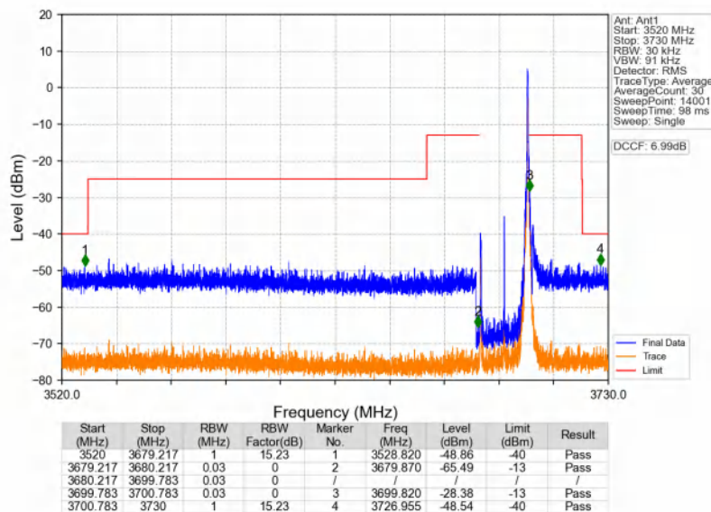
n48_30kHz_SISO_NTNV_20MHz_DFT-s-OFDM QPSK_3690MHz_Edge_1RB_Right
