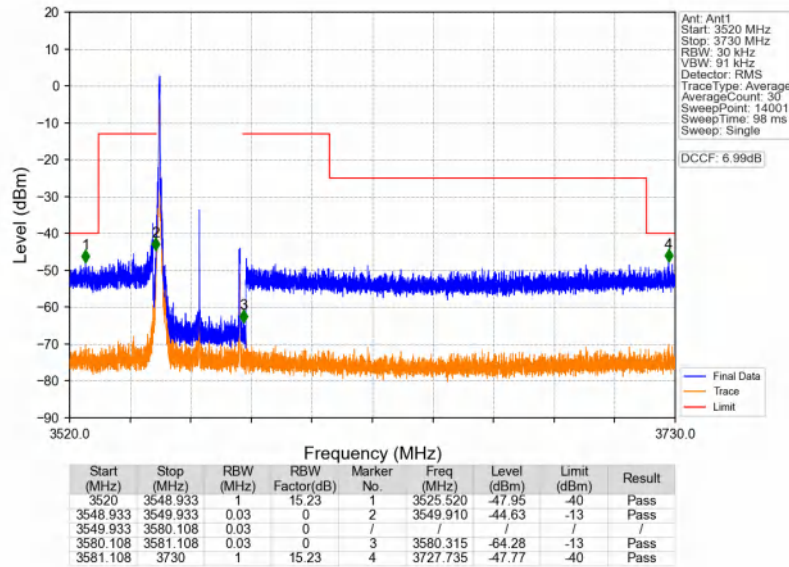
n48_30kHz_SISO_NTNV_30MHz_CP-OFDM QPSK_3565.02MHz_Edge_1RB_Left
