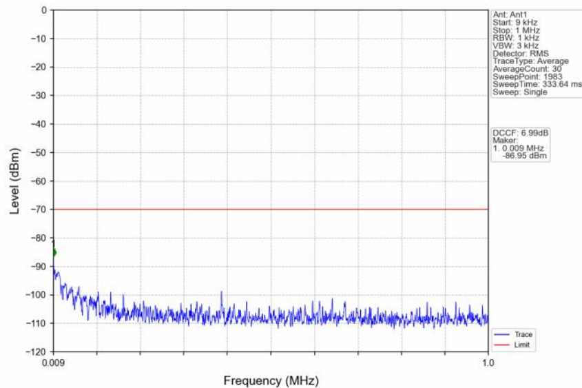
n48_30kHz_SISO_NTNV_30MHz_DFT-s-OFDM QPSK_3684.99MHz_Outer_Full
