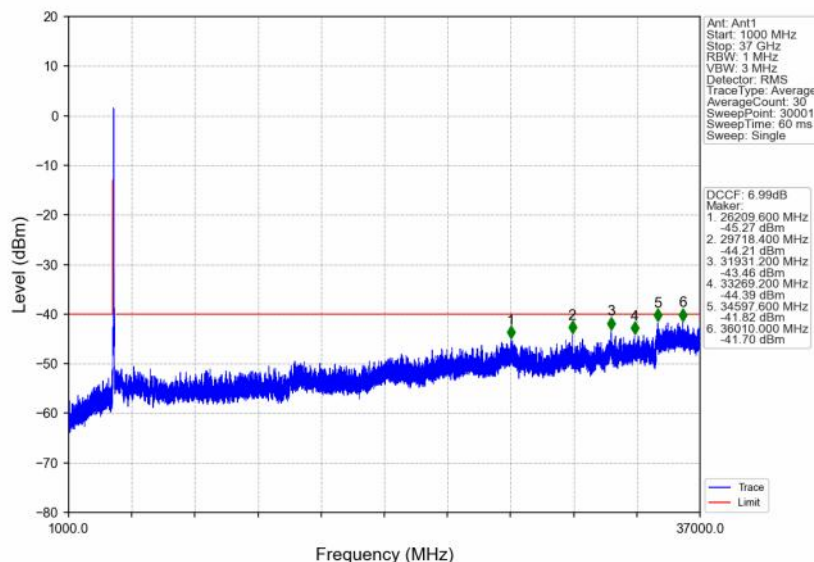
n48_30kHz_SISO_NTNV_40MHz_DFT-s-OFDM_PI/2_BPSK_3570MHz_Outer_Full
