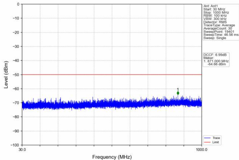
n48_30kHz_SISO_NTNV_30MHz_DFT-s-OFDM QPSK_3624.99MHz_Edge_1RB_Left
