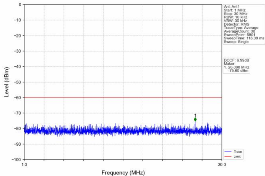
n48_30kHz_SISO_NTNV_30MHz_CP-OFDM QPSK_3565.02MHz_Inner_1RB_Left
