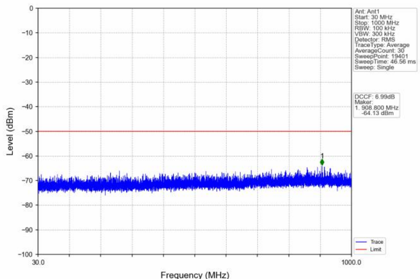
n48_30kHz_SISO_NTNV_30MHz_DFT-s-OFDM QPSK_3684.99MHz_Outer_Full
