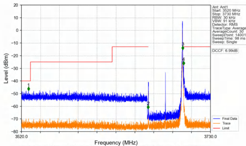
n48_30kHz_SISO_NTNV_40MHz_DFT-s-OFDM QPSK_3679.98MHz_Edge_1RB_Right
