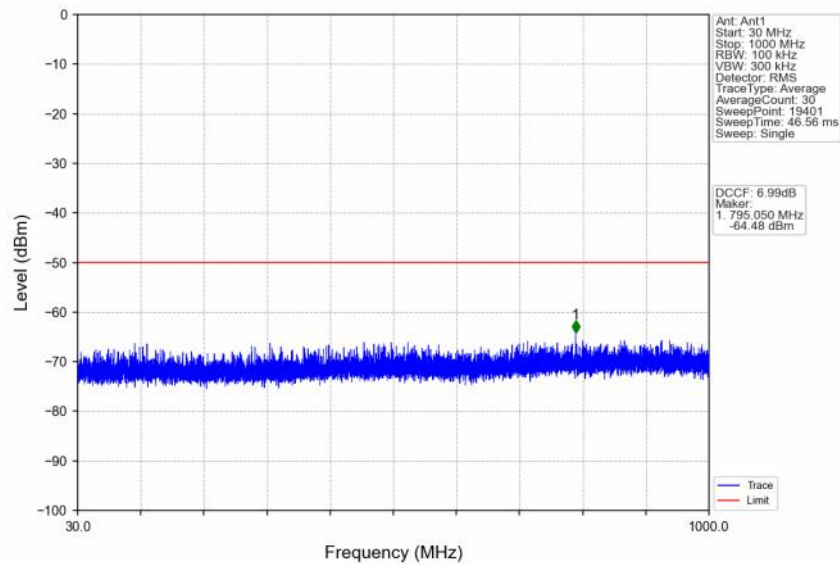
n48_30kHz_SISO_NTNV_40MHz_DFT-s-OFDM QPSK_3679.98MHz_Edge_1RB_Right
