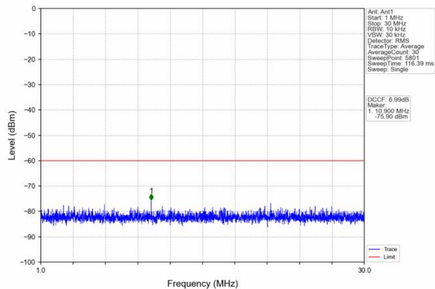
n48_30kHz_SISO_NTNV_30MHz_DFT-s-OFDM QPSK_3565.02MHz_Outer_Full
