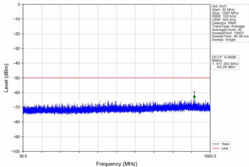
n48_30kHz_SISO_NTNV_30MHz_CP-OFDM QPSK_3565.02MHz_Edge_1RB_Left
