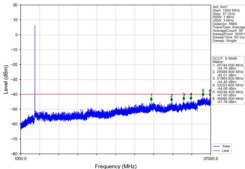
n48_30kHz_SISO_NTNV_30MHz_CP-OFDM QPSK_3684.99MHz_Outer_Full
