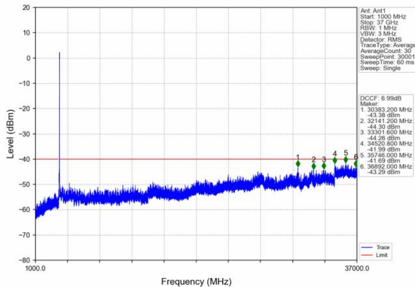
n48_30kHz_SISO_NTNV_30MHz_DFT-s-OFDM_PI/2_BPSK_3684.99MHz_Outer_Full
