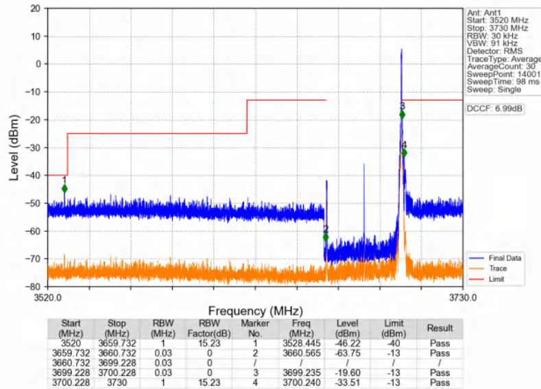
n48_30kHz_SISO_NTNV_40MHz_CP-OFDM QPSK_3679.98MHz_Edge_1RB_Right
