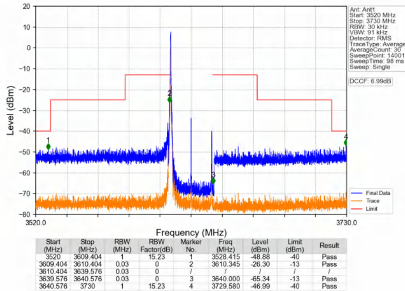
n48_30kHz_SISO_NTNV_30MHz_DFT-s-OFDM QPSK_3624.99MHz_Edge_1RB_Left
