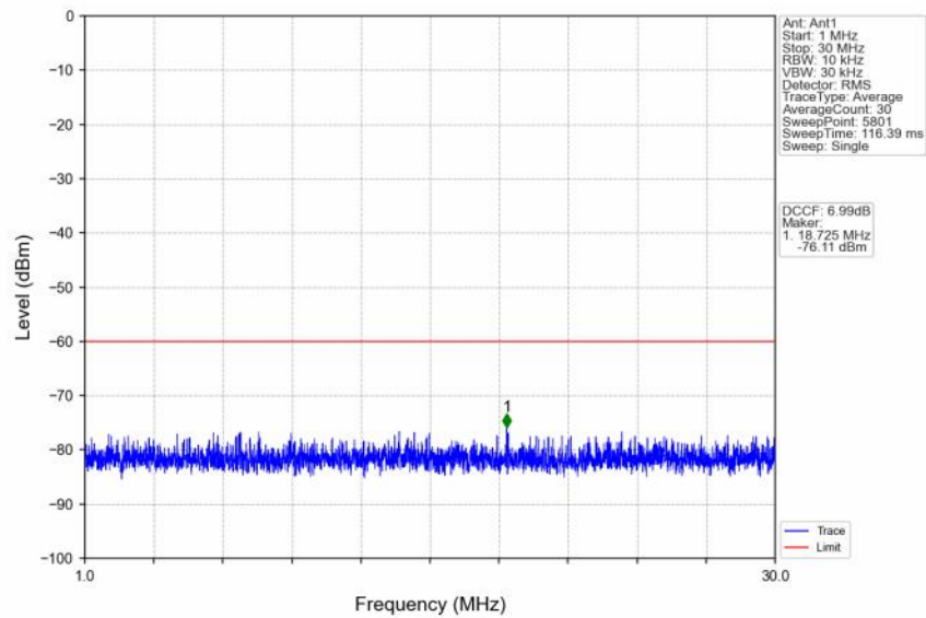
n48_30kHz_SISO_NTNV_30MHz_CP-OFDM QPSK_3565.02MHz_Edge_1RB_Left
