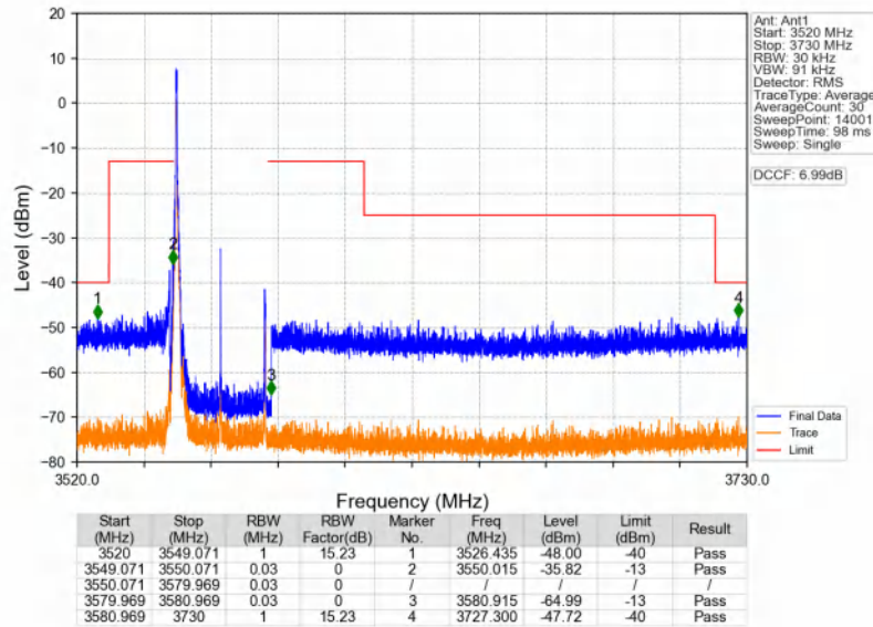
n48_30kHz_SISO_NTNV_30MHz_DFT-s-OFDM QPSK_3565.02MHz_Edge_1RB_Left
