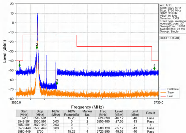
n48_30kHz_SISO_NTNV_30MHz_DFT-s-OFDM QPSK_3565.02MHz_Inner_1RB_Left
