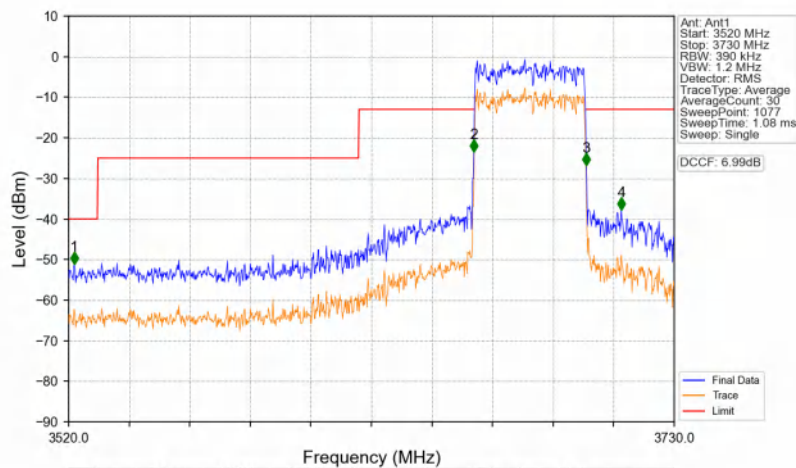
n48_30kHz_SISO_NTNV_40MHz_CP-OFDM QPSK_3679.98MHz_Outer_Full
