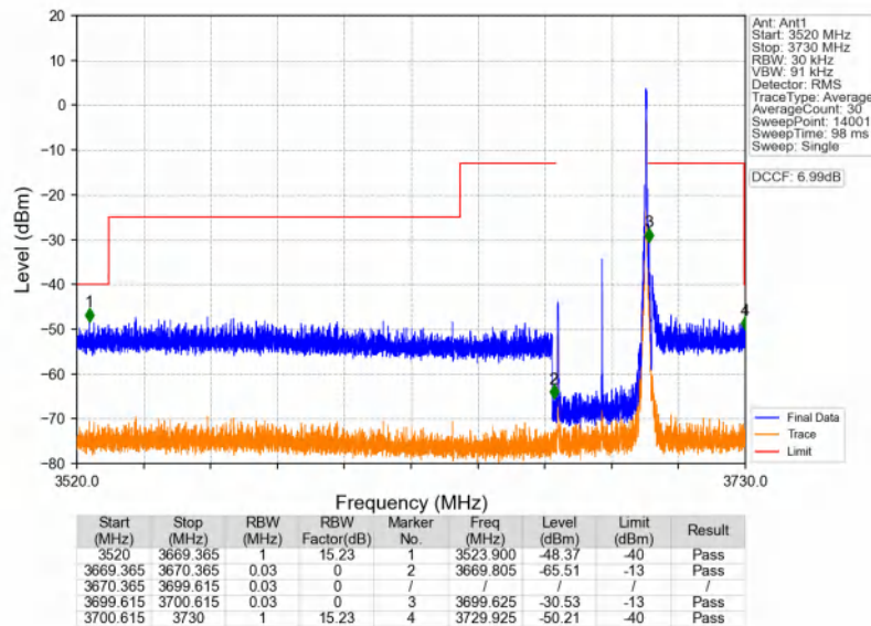
n48_30kHz_SISO_NTNV_30MHz_CP-OFDM QPSK_3684.99MHz_Edge_1RB_Right
