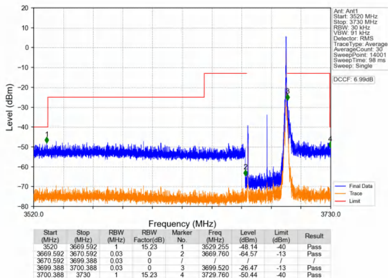
n48_30kHz_SISO_NTNV_30MHz_DFT-s-OFDM QPSK_3684.99MHz_Inner_1RB_Right
