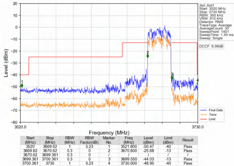
n48_30kHz_SISO_NTNV_30MHz_DFT-s-OFDM QPSK_3684.99MHz_Outer_Full
