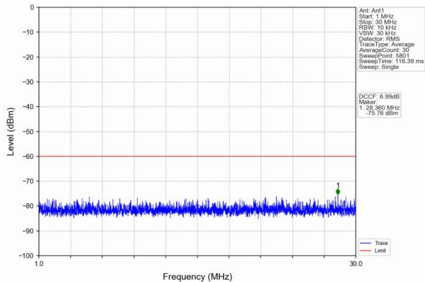
n48_30kHz_SISO_NTNV_30MHz_CP-OFDM QPSK_3684.99MHz_Inner_1RB_Right
