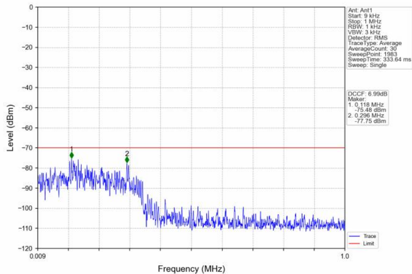
n48_30kHz_SISO_NTNV_30MHz_DFT-s-OFDM QPSK_3565.02MHz_Edge_1RB_Left
