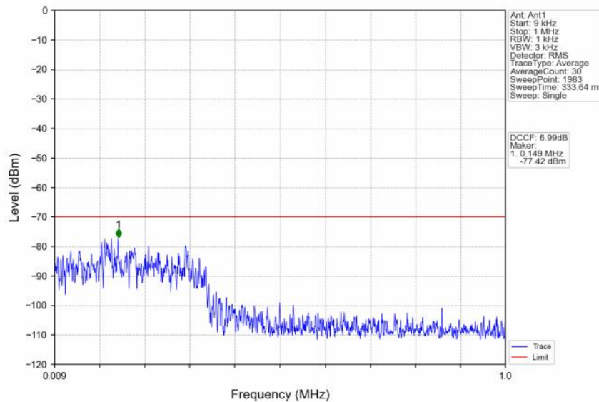
n48_30kHz_SISO_NTNV_40MHz_DFT-s-OFDM QPSK_3624.99MHz_Edge_1RB_Left
