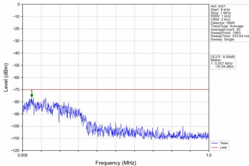
n48_30kHz_SISO_NTNV_30MHz_CP-OFDM QPSK_3565.02MHz_Edge_1RB_Left
