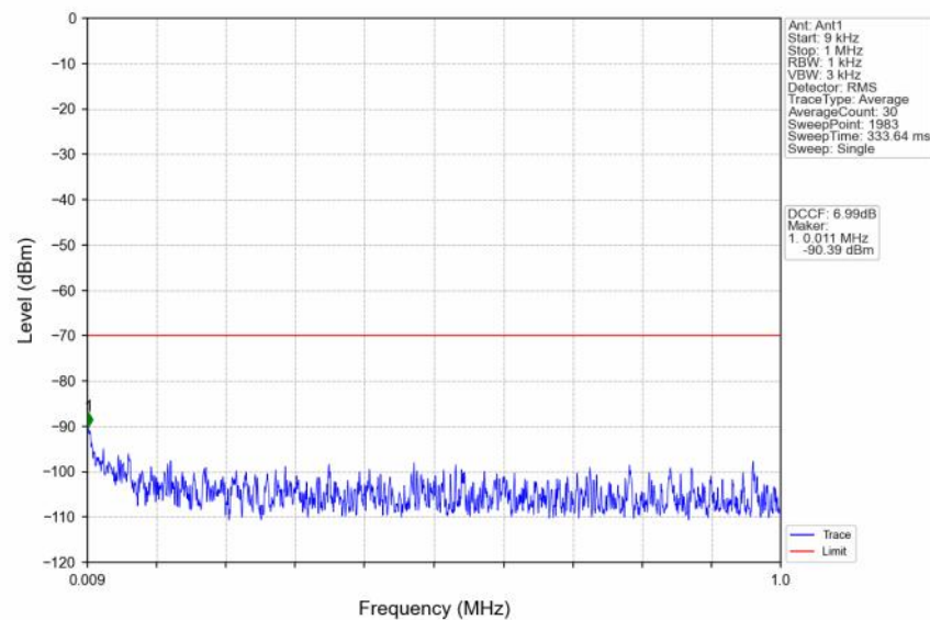
n48_30kHz_SISO_NTNV_40MHz_CP-OFDM QPSK_3679.98MHz_Outer_Full
