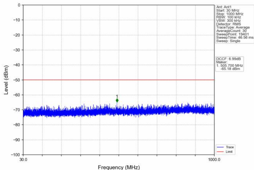
n48_30kHz_SISO_NTNV_30MHz_DFT-s-OFDM QPSK_3684.99MHz_Edge_1RB_Right
