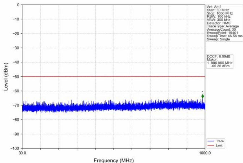
n48_30kHz_SISO_NTNV_30MHz_DFT-s-OFDM QPSK_3684.99MHz_Inner_1RB_Right
