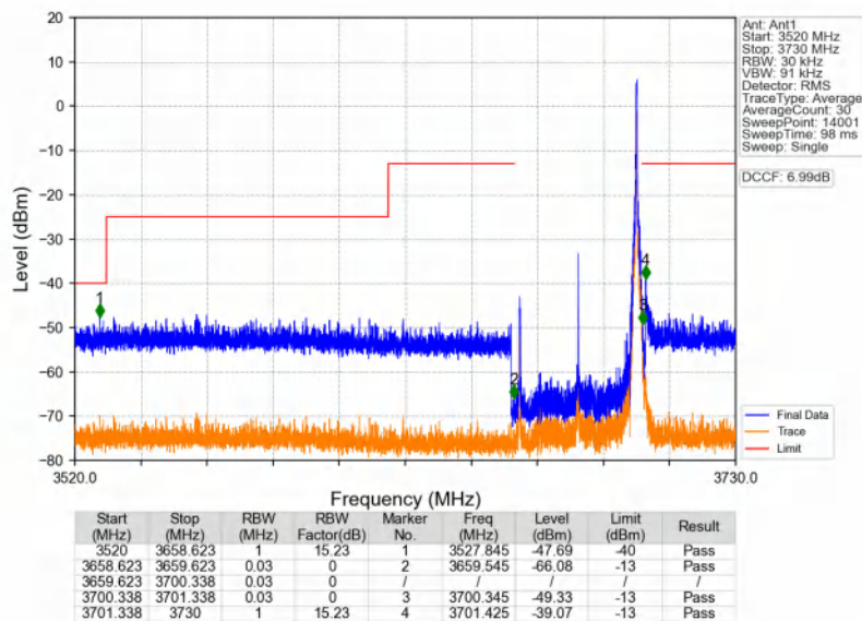
n48_30kHz_SISO_NTNV_40MHz_CP-OFDM QPSK_3679.98MHz_Inner_1RB_Right
