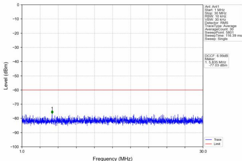
n48_30kHz_SISO_NTNV_30MHz_CP-OFDM QPSK_3565.02MHz_Outer_Full
