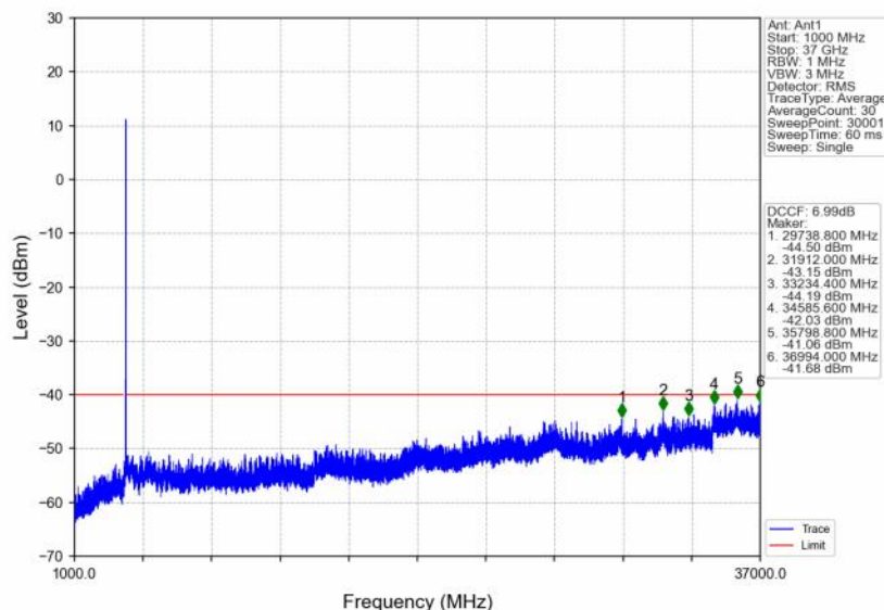
n48_30kHz_SISO_NTNV_30MHz_DFT-s-OFDM QPSK_3684.99MHz_Inner_1RB_Right
