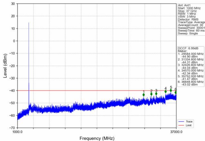
n48_30kHz_SISO_NTNV_30MHz_DFT-s-OFDM QPSK_3565.02MHz_Edge_1RB_Left
