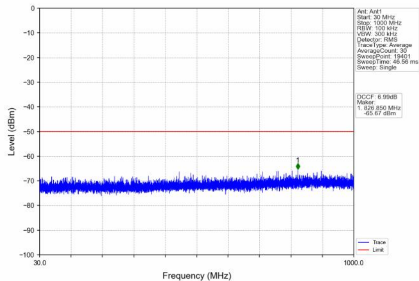
n48_30kHz_SISO_NTNV_30MHz_DFT-s-OFDM QPSK_3565.02MHz_Outer_Full
