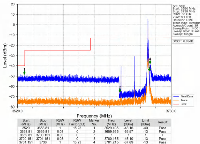
n48_30kHz_SISO_NTNV_40MHz_DFT-s-OFDM QPSK_3679.98MHz_Inner_1RB_Right
