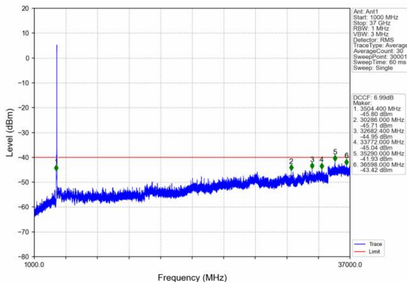
n48_30kHz_SISO_NTNV_30MHz_DFT-s-OFDM QPSK_3565.02MHz_Inner_1RB_Left
