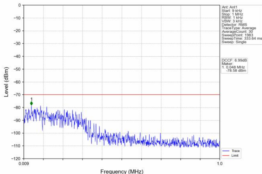
n48_30kHz_SISO_NTNV_40MHz_CP-OFDM QPSK_3679.98MHz_Inner_1RB_Right
