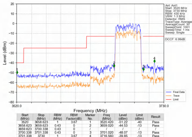
n48_30kHz_SISO_NTNV_40MHz_DFT-s-OFDM QPSK_3679.98MHz_Outer_Full
