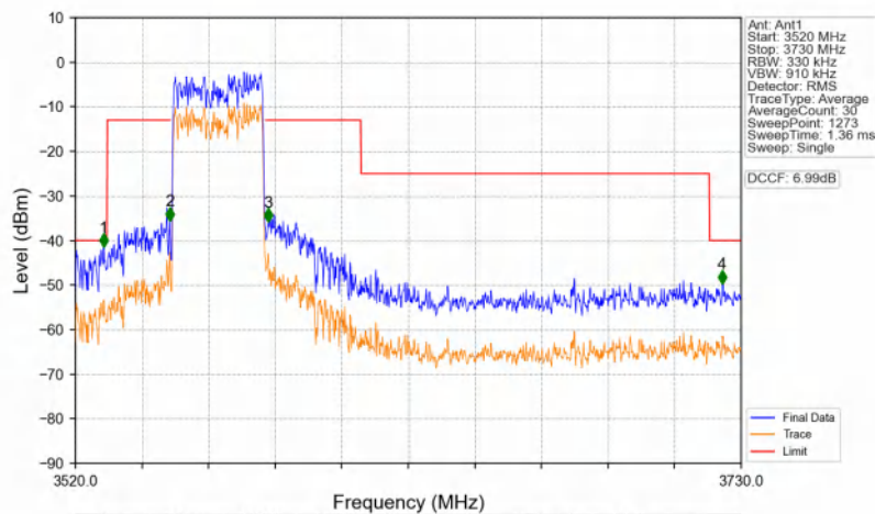
n48_30kHz_SISO_NTNV_30MHz_CP-OFDM QPSK_3565.02MHz_Outer_Full
