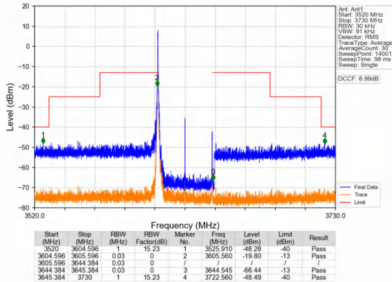
n48_30kHz_SISO_NTNV_40MHz_DFT-s-OFDM QPSK_3624.99MHz_Edge_1RB_Left
