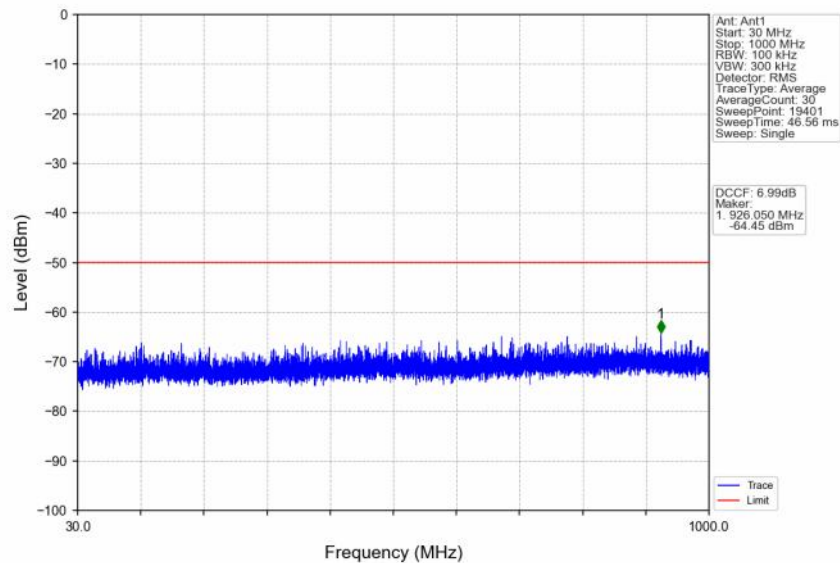
n48_30kHz_SISO_NTNV_30MHz_CP-OFDM QPSK_3624.99MHz_Edge_1RB_Left
