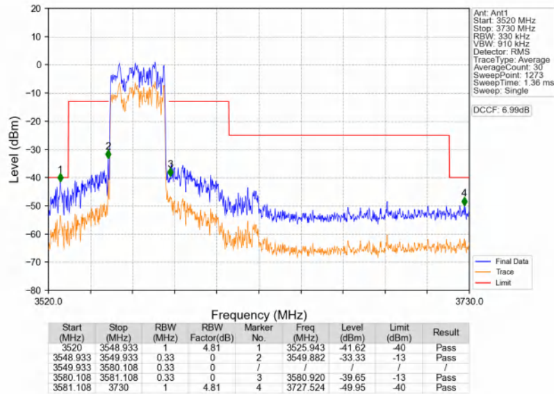
n48_30kHz_SISO_NTNV_30MHz_DFT-s-OFDM QPSK_3565.02MHz_Outer_Full
