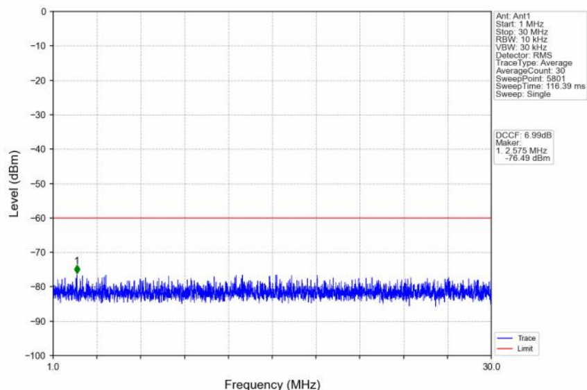
n48_30kHz_SISO_NTNV_30MHz_DFT-s-OFDM_QPSK_3565.02MHz_Inner_1RB_Left
