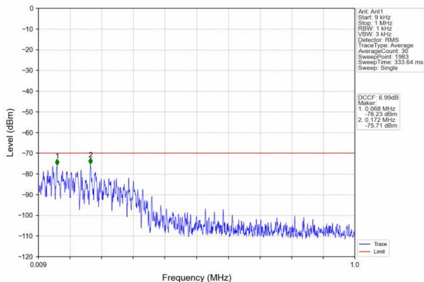
n48_30kHz_SISO_NTNV_30MHz_CP-OFDM QPSK_3624.99MHz_Edge_1RB_Left
