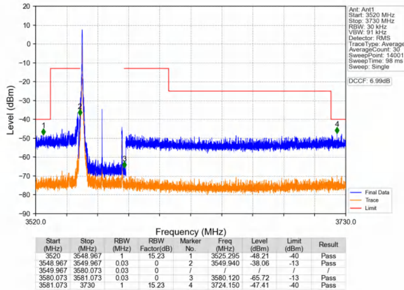
n48_30kHz_SISO_NTNV_30MHz_CP-OFDM QPSK_3565.02MHz_Inner_1RB_Left
