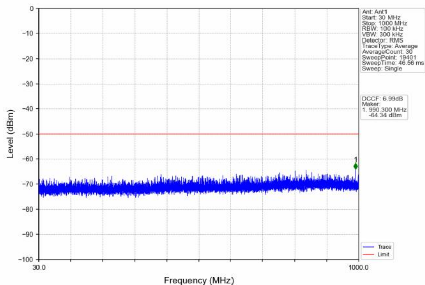
n48_30kHz_SISO_NTNV_30MHz_DFT-s-OFDM QPSK_3565.02MHz_Inner_1RB_Left
