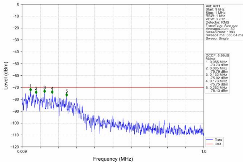
n48_30kHz_SISO_NTNV_30MHz_CP-OFDM QPSK_3565.02MHz_Inner_1RB_Left
