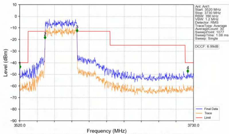
n48_30kHz_SISO_NTNV_40MHz_CP-OFDM QPSK_3570MHz_Outer_Full
