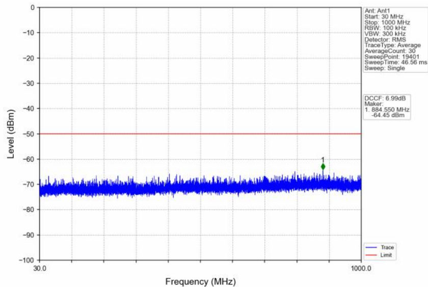
n48_30kHz_SISO_NTNV_30MHz_DFT-s-OFDM QPSK_3565.02MHz_Edge_1RB_Left
