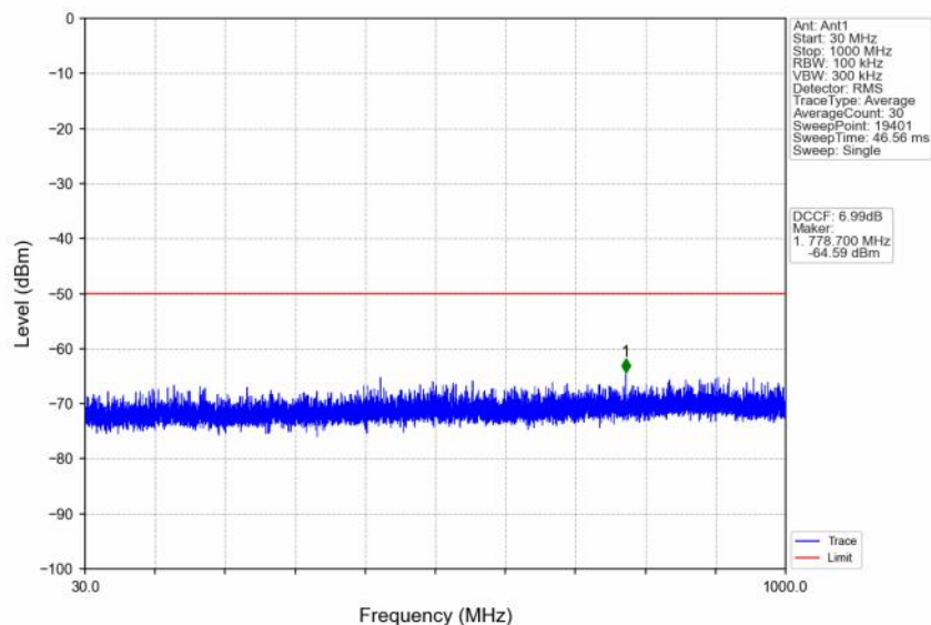
n48_30kHz_SISO_NTNV_40MHz_DFT-s-OFDM_PI/2_BPSK_3570MHz_Outer_Full
