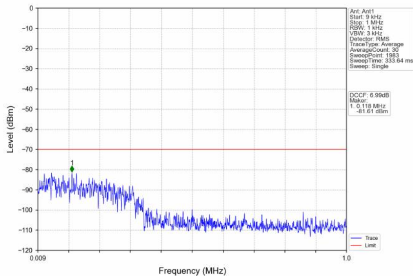
n48_30kHz_SISO_NTNV_30MHz_CP-OFDM QPSK_3684.99MHz_Edge_1RB_Right
