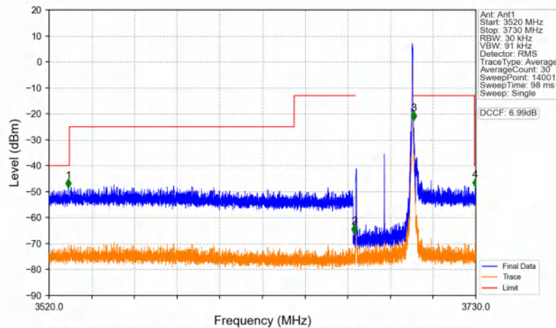
n48_30kHz_SISO_NTNV_30MHz_DFT-s-OFDM QPSK_3684.99MHz_Edge_1RB_Right
