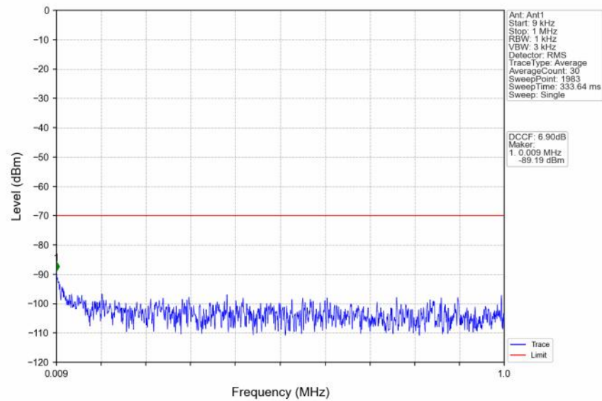
n48_30kHz_SISO_NTNV_30MHz_CP-OFDM QPSK_3684.99MHz_Outer_Full
