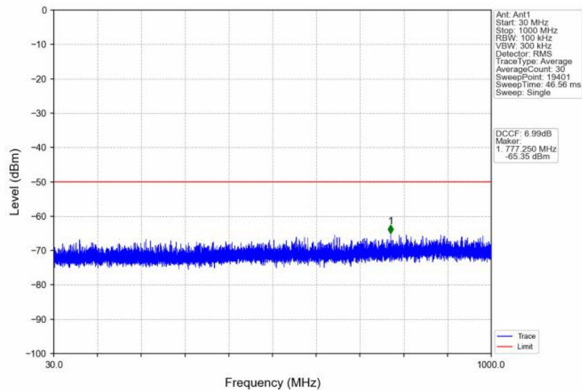
n48_30kHz_SISO_NTNV_30MHz_CP-OFDM QPSK_3684.99MHz_Edge_1RB_Right
