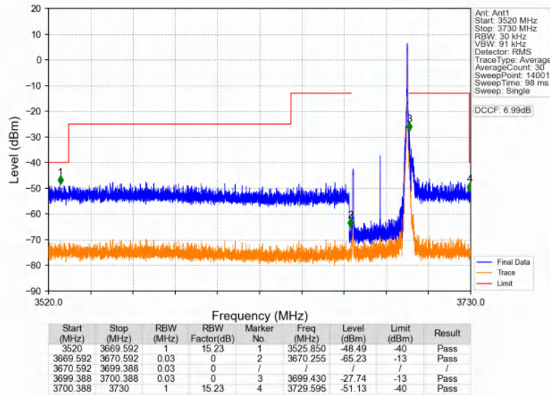
n48_30kHz_SISO_NTNV_30MHz_CP-OFDM QPSK_3684.99MHz_Inner_1RB_Right
