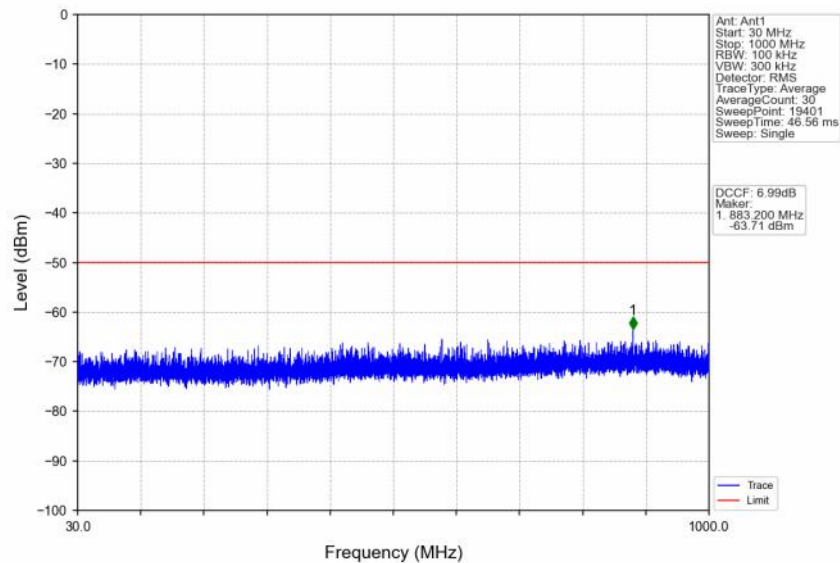
n48_30kHz_SISO_NTNV_30MHz_CP-OFDM QPSK_3684.99MHz_Inner_1RB_Right
