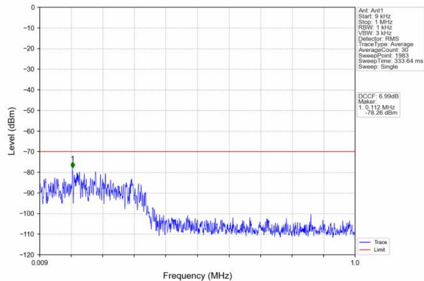
n48_30kHz_SISO_NTNV_30MHz_DFT-s-OFDM QPSK_3684.99MHz_Inner_1RB_Right
