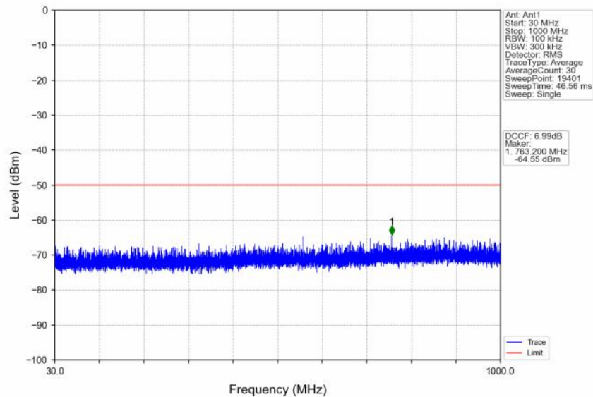
n48_30kHz_SISO_NTNV_30MHz_CP-OFDM QPSK_3565.02MHz_Inner_1RB_Left
