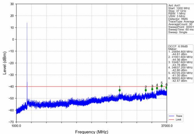
n48_30kHz_SISO_NTNV_30MHz_CP-OFDM QPSK_3624.99MHz_Edge_1RB_Left
