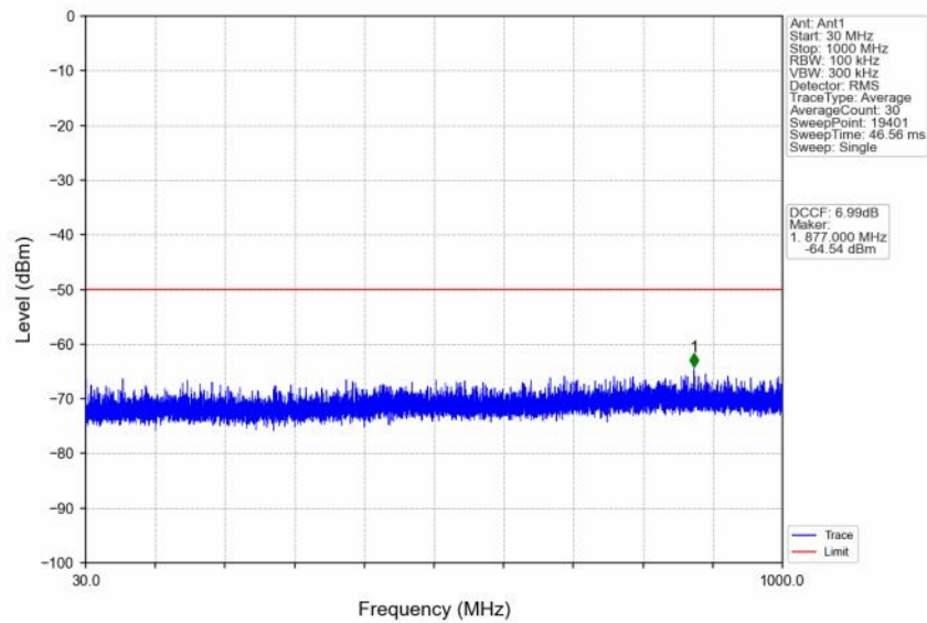
n48_30kHz_SISO_NTNV_30MHz_DFT-s-OFDM_PI/2_BPSK_3684.99MHz_Outer_Full
