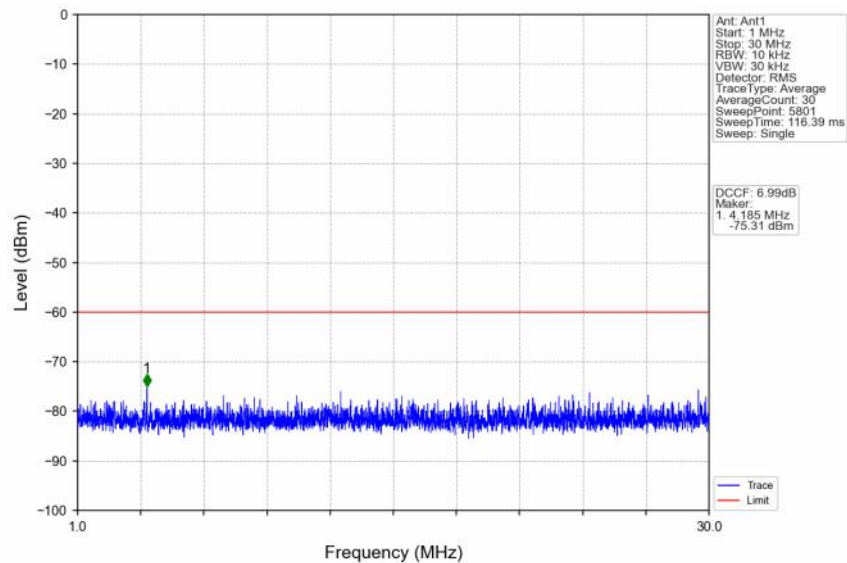
n48_30kHz_SISO_NTNV_30MHz_CP-OFDM QPSK_3684.99MHz_Edge_1RB_Right
