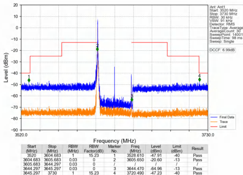
n48_30kHz_SISO_NTNV_40MHz_CP-OFDM QPSK_3624.99MHz_Edge_1RB_Left
