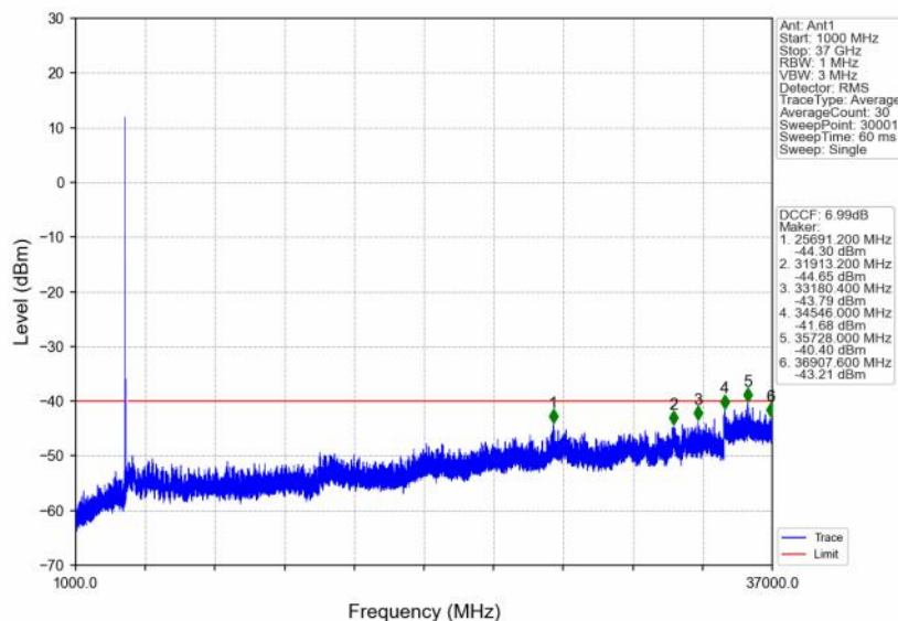
n48_30kHz_SISO_NTNV_30MHz_CP-OFDM QPSK_3565.02MHz_Outer_Full
