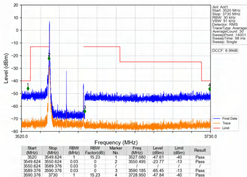
n48_30kHz_SISO_NTNV_40MHz_DFT-s-OFDM QPSK_3570MHz_Edge_1RB_Left
