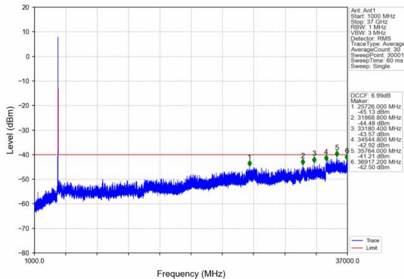
n48_30kHz_SISO_NTNV_40MHz_DFT-s-OFDM QPSK_3679.98MHz_Edge_1RB_Right
