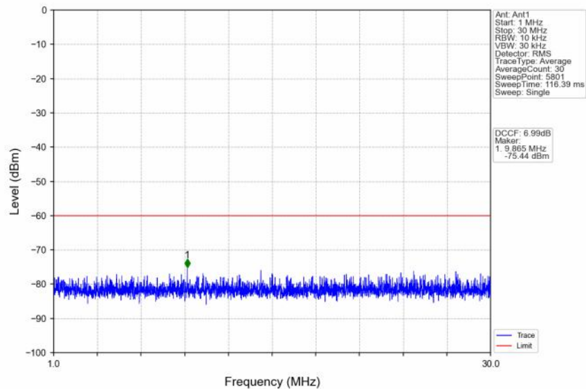
n48_30kHz_SISO_NTNV_30MHz_DFT-s-OFDM QPSK_3624.99MHz_Edge_1RB_Left
