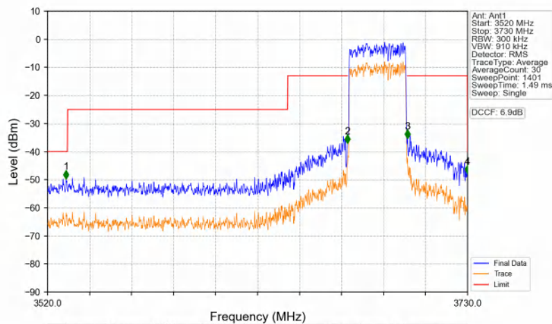
n48_30kHz_SISO_NTNV_30MHz_CP-OFDM QPSK_3684.99MHz_Outer_Full
