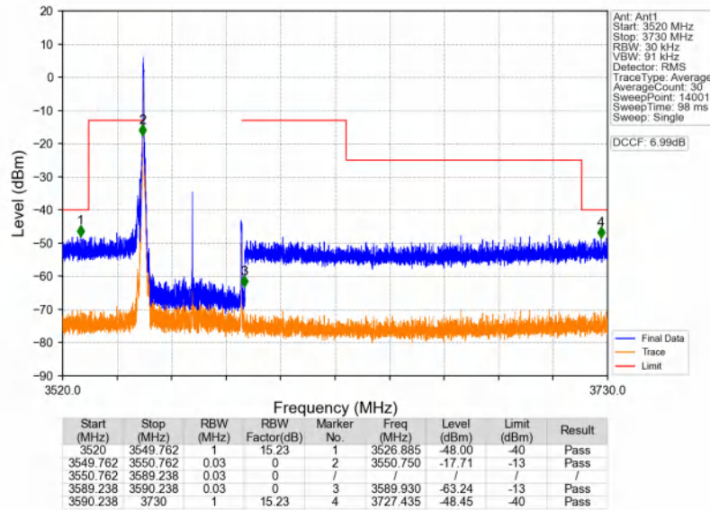
n48_30kHz_SISO_NTNV_40MHz_CP-OFDM_QPSK_3570MHz_Edge_1RB_Left
