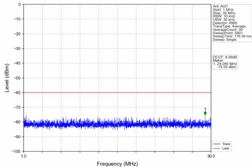
n48_30kHz_SISO_NTNV_30MHz_DFT-s-OFDM QPSK_3684.99MHz_Edge_1RB_Right
