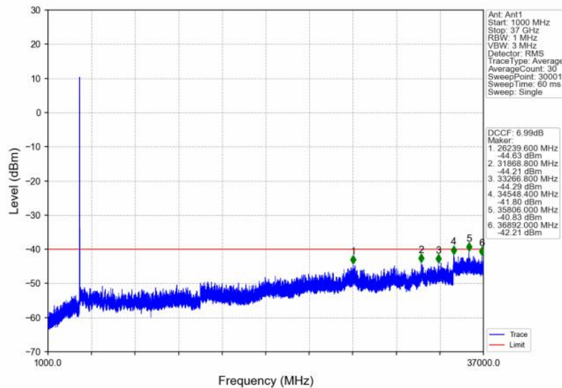
n48_30kHz_SISO_NTNV_30MHz_DFT-s-OFDM QPSK_3684.99MHz_Edge_1RB_Right
