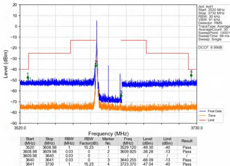
n48_30kHz_SISO_NTNV_30MHz_CP-OFDM QPSK_3624.99MHz_Edge_1RB_Left
