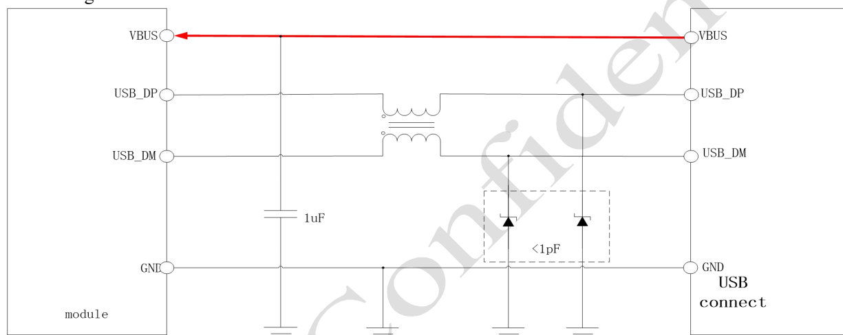
Figure 4.23: USB Connection Diagram
