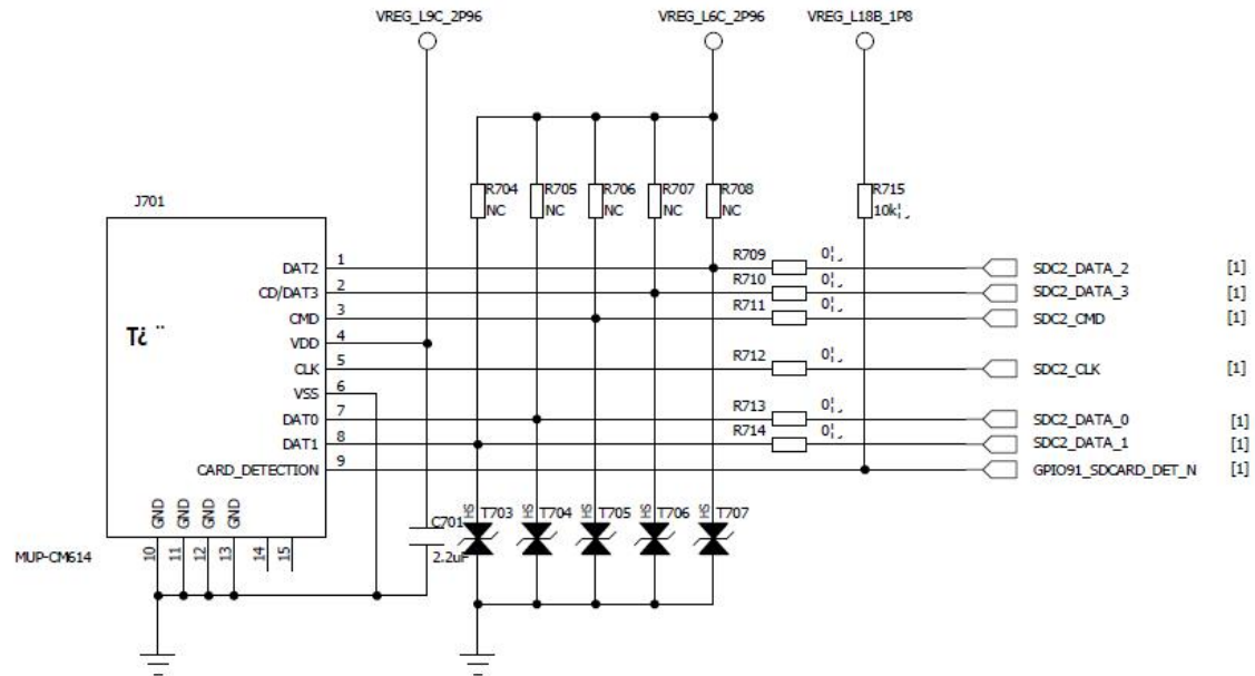
Figure 4.26: SD Card Interface Circuit
