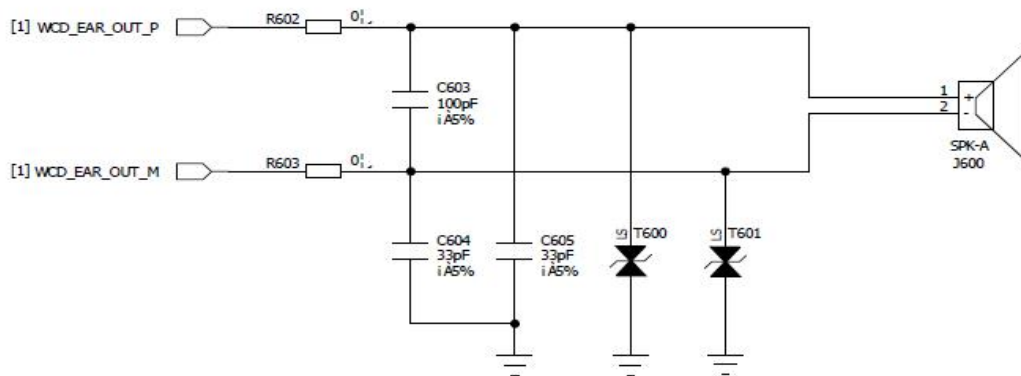
Figure 4.19: Receiver Interface Circuit
