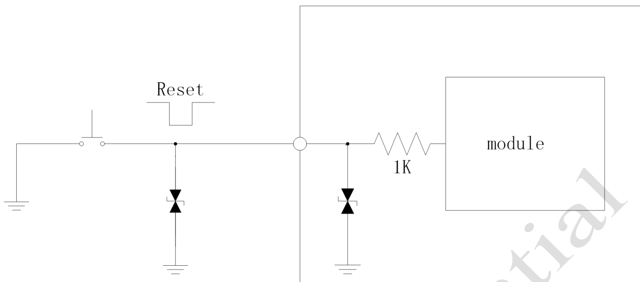
Figure 4.6: Reset using key circuit
