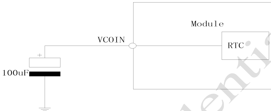
Figure 4.8: External Capacitor Powering the RTC
