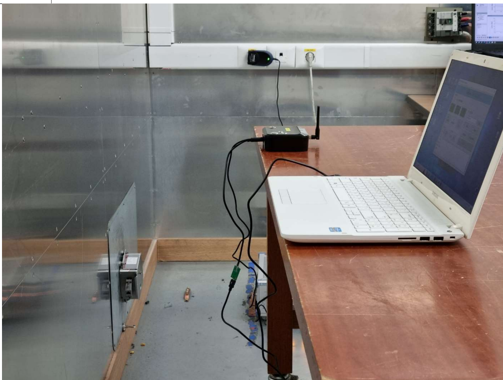
Radiated measurement for Above 1 GHz (Side)
