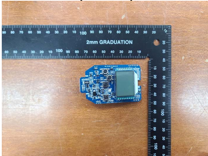
[Mainboard Front]
