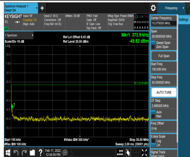
Band26-5MHz-16QAM-26815-1-0-Low-0.15-30--49.83-PASS
