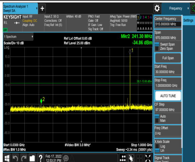
Band26-5MHz-QPSK-27015-1-0-High-30-1000--34.86-PASS
