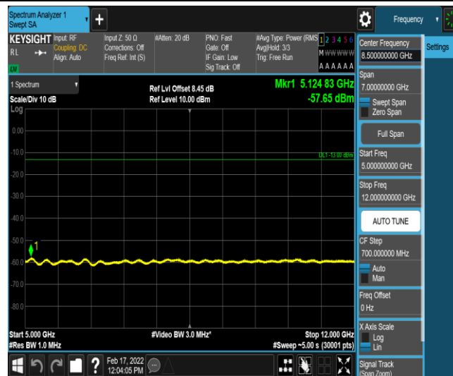
Band26-3MHz-16QAM-26805-1-0-Low-5000-12000--57.65-PASS
