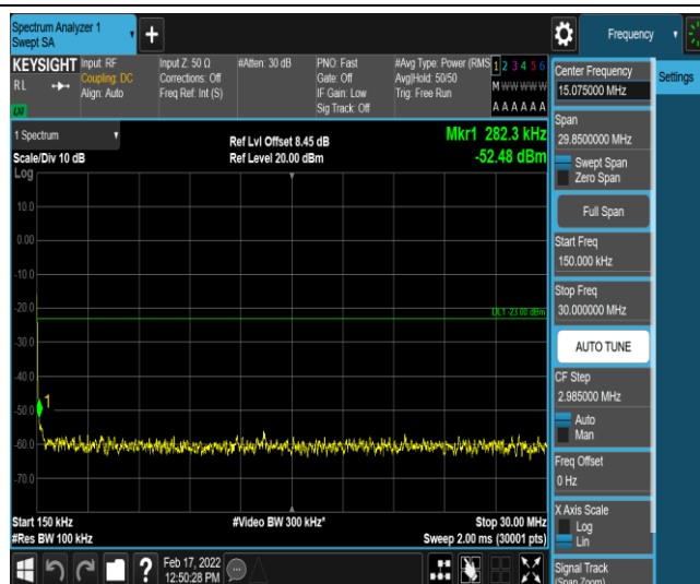
Band26-5MHz-QPSK-26915-1-0-Low-0.15-30--52.48-PASS
