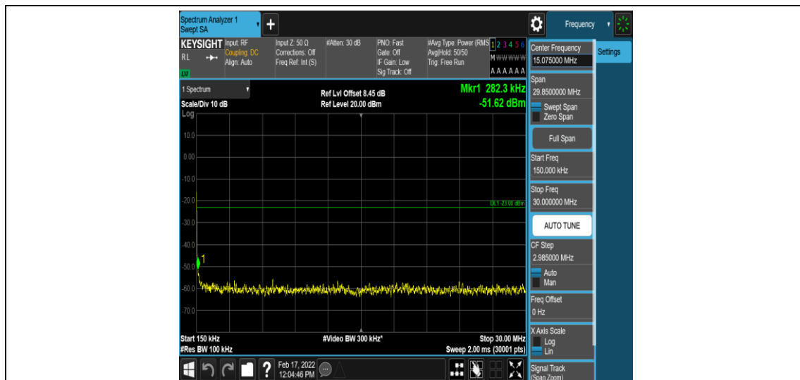
Band26-3MHz-QPSK-26915-1-0-Low-0.15-30--51.62-PASS
