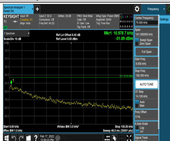
Band26-5MHz-QPSK-26915-1-0-Low-0.009-0.15--51.89-PASS
