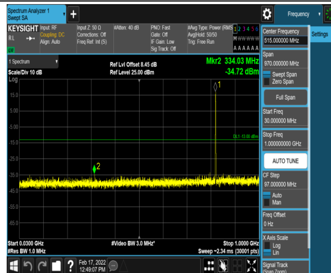
Band26-5MHz-16QAM-26815-1-0-Low-30-1000--34.72-PASS
