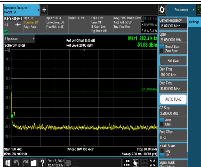
Band26-5MHz-QPSK-26815-1-0-Low-0.15-30--51.53-PASS
