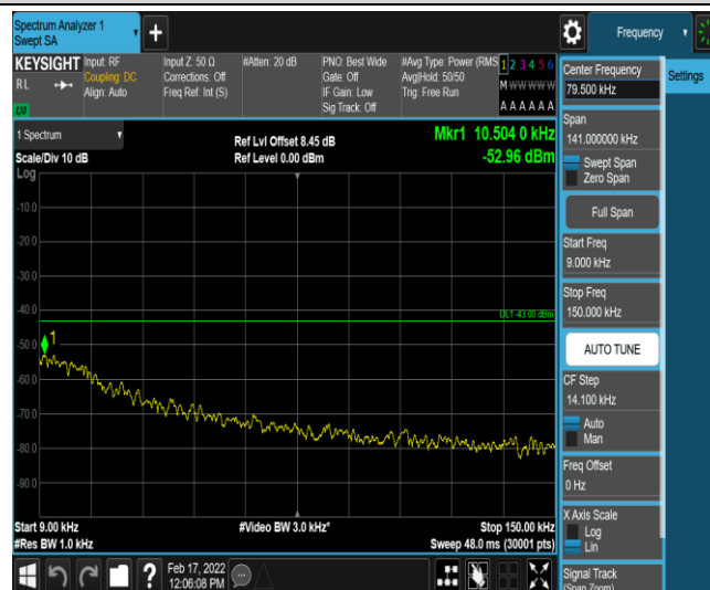
Band26-3MHz-16QAM-26915-1-0-Low-0.009-0.15--52.97-PASS
