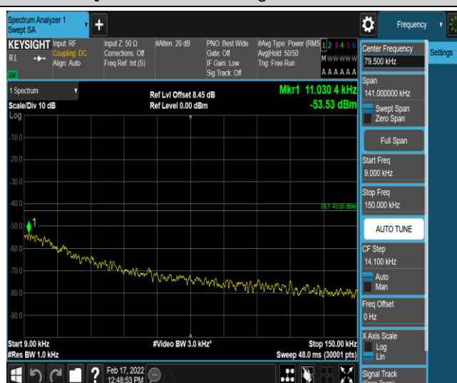
Band26-5MHz-16QAM-26815-1-0-Low-0.009-0.15--53.53-PASS
