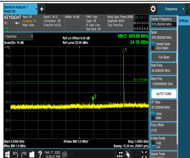
Band26-3MHz-16QAM-26805-1-0-Low-30-1000--34.18-PASS
