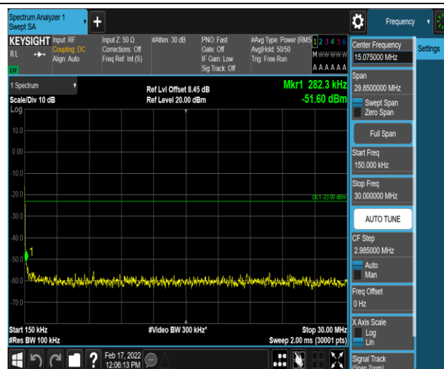
Band26-3MHz-16QAM-26915-1-0-Low-0.15-30--51.6-PASS
