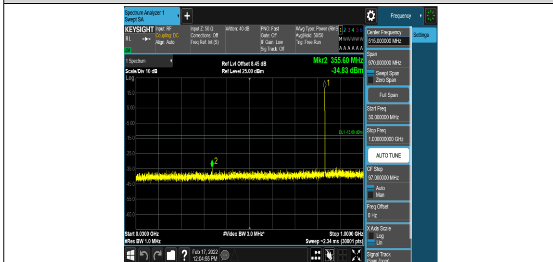
Band26-3MHz-QPSK-26915-1-0-Low-30-1000--34.83-PASS
