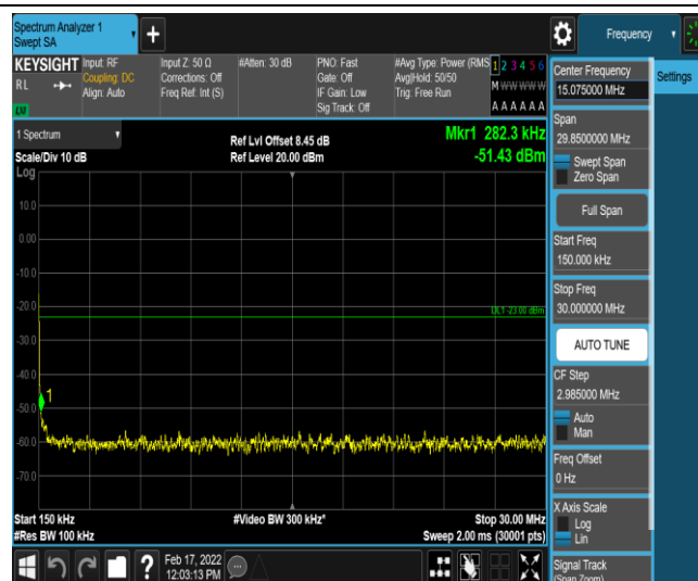
Band26-3MHz-16QAM-26805-1-0-Low-0.15-30--51.43-PASS
