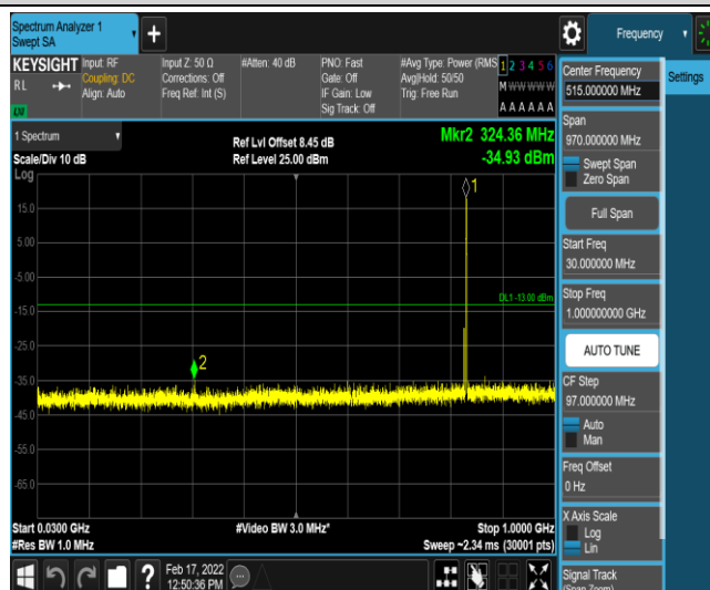
Band26-5MHz-QPSK-26915-1-0-Low-30-1000--34.93-PASS
