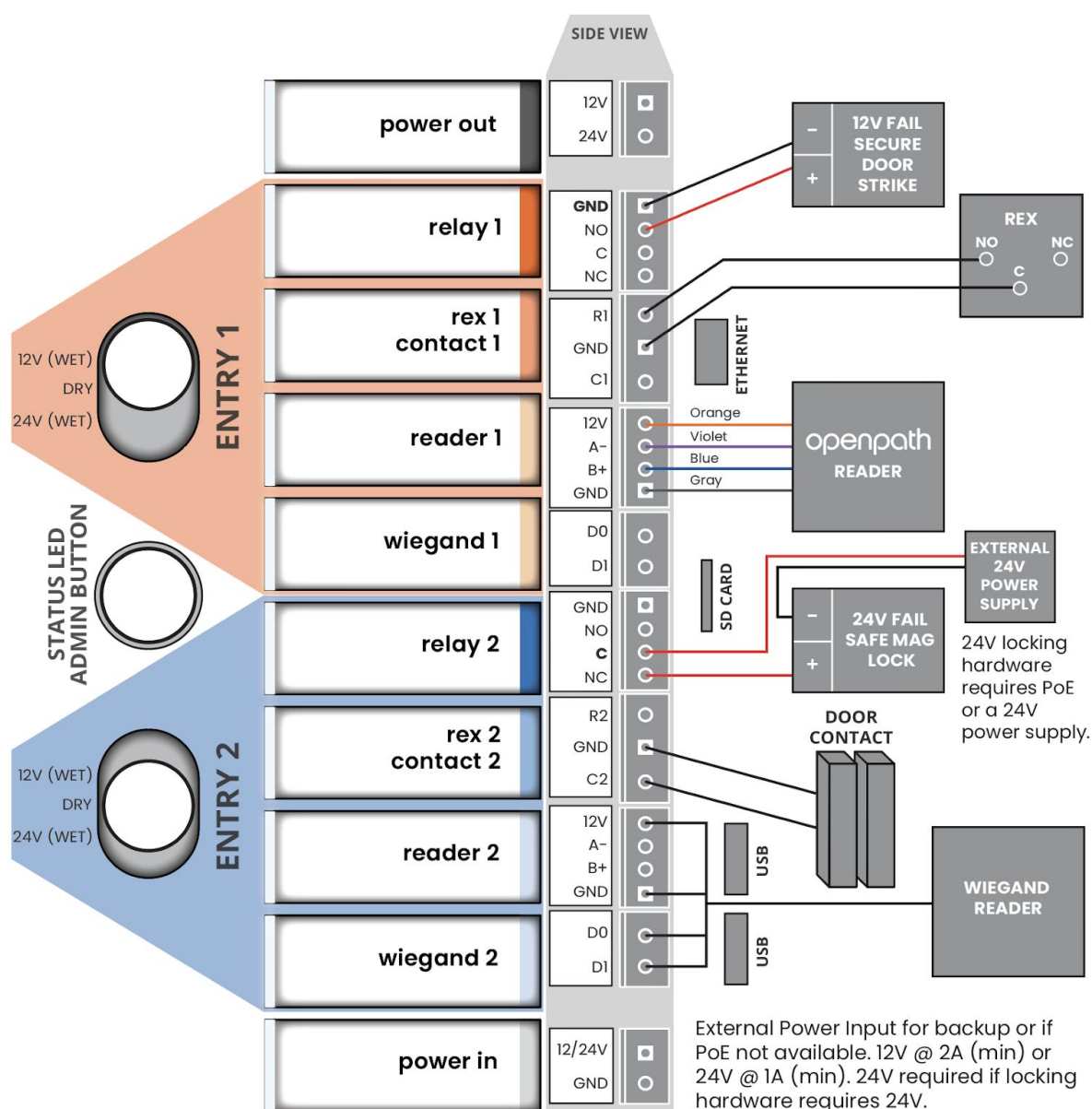
Figure 2: Example SDC wiring
