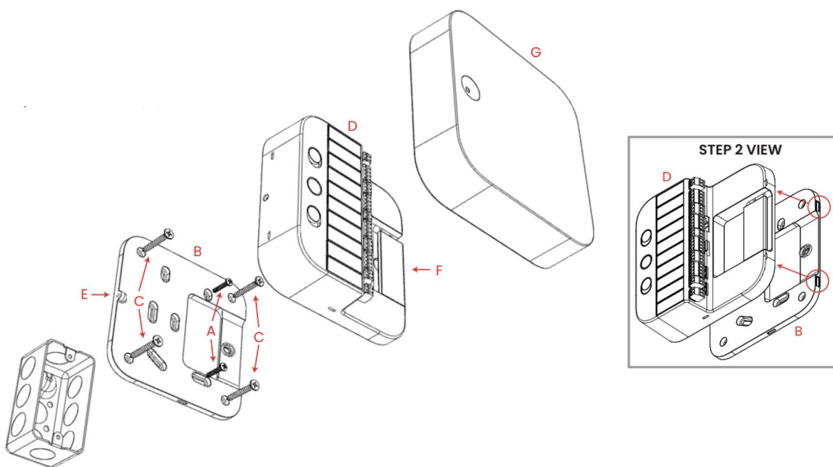
Figure 1: Mounting SDC to wall
