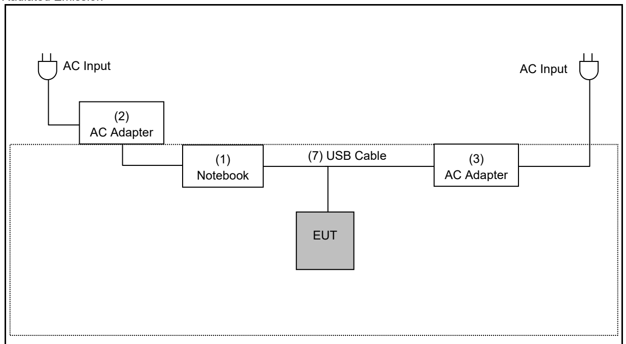
Radiated Emission
