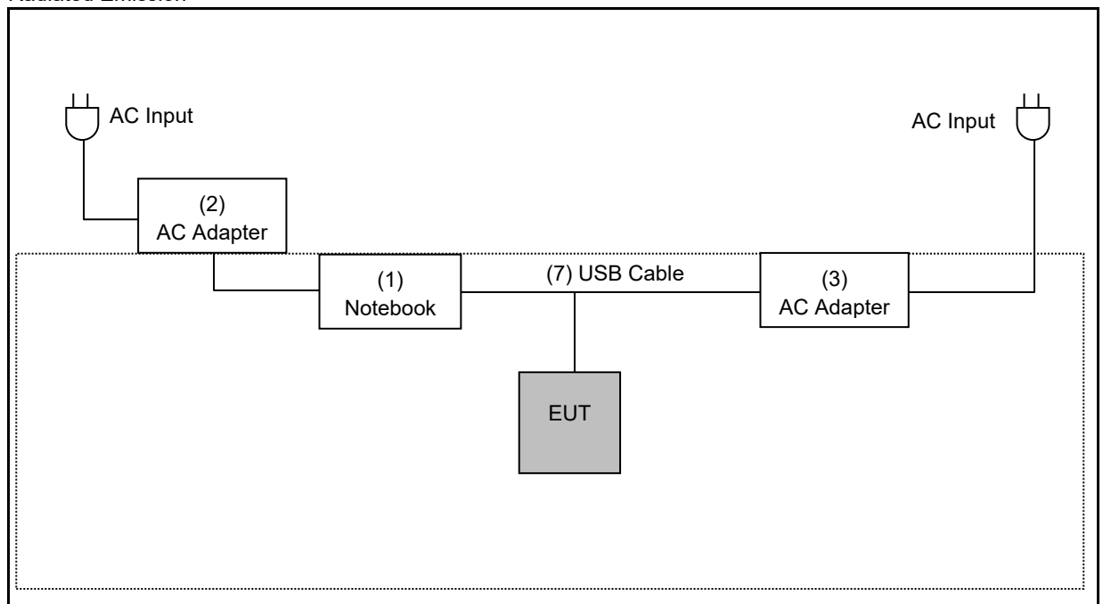
Radiated Emission
