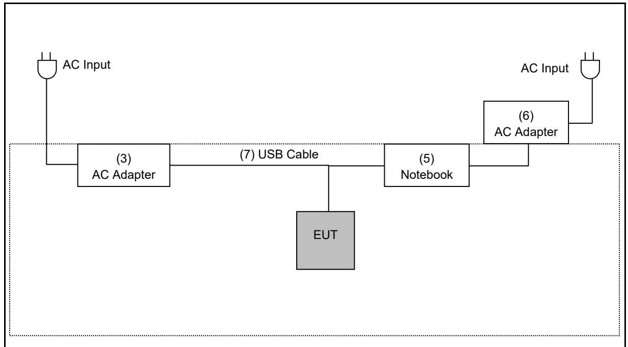
Conducted Emission
