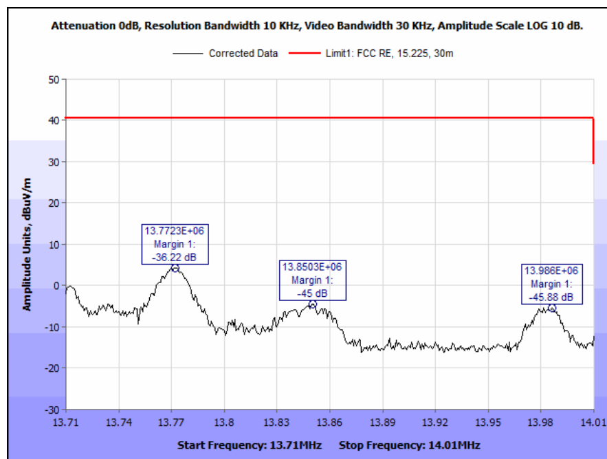
Plot 12. Fundamental Field Strength Within the Band 13.710 – 14.010 MHz, 90°
