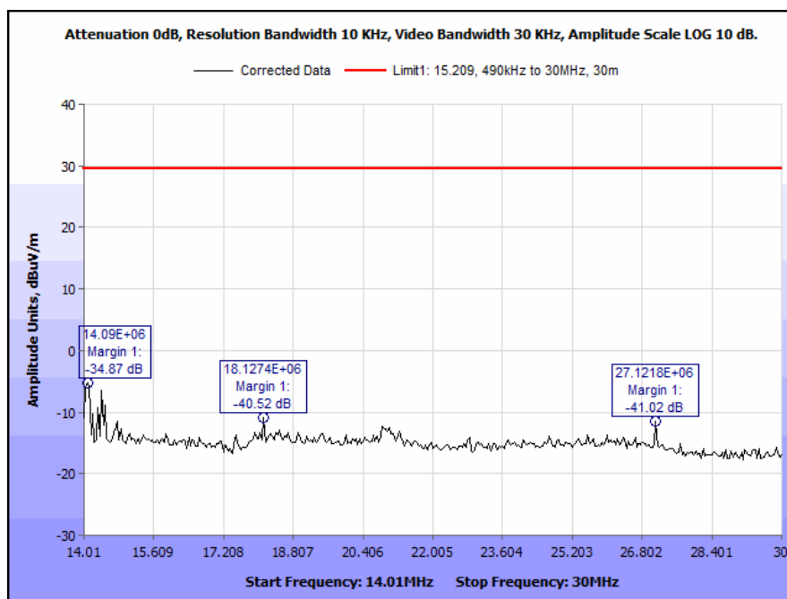
Plot 22. Spurious Emissions, Outside the Bands 13.110 - 14.010 MHz, 14.01 MHz – 30 MHz, 90°
