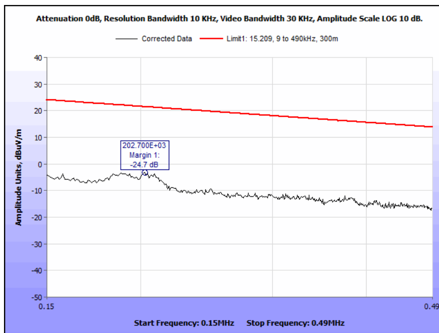
Plot 15. Spurious Emissions, Outside the Bands 13.110 - 14.010 MHz, 150 kHz – 490 kHz, 0°
