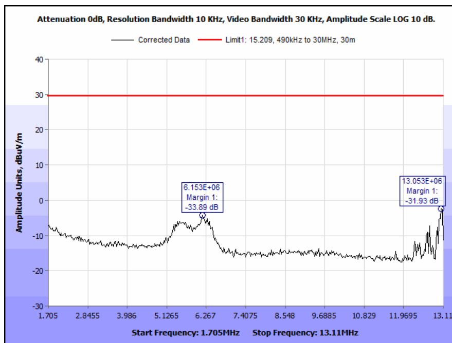
Plot 19. Spurious Emissions, Outside the Bands 13.110 - 14.010 MHz, 1.705 MHz – 13.11 MHz, 0°
