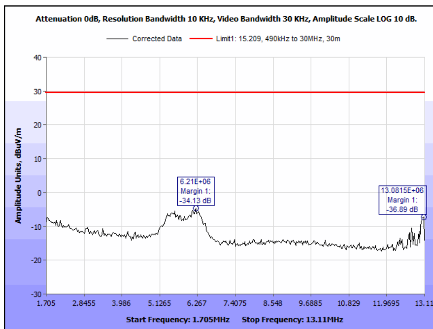
Plot 20. Spurious Emissions, Outside the Bands 13.110 - 14.010 MHz, 1.705 MHz – 13.11 MHz, 90°
