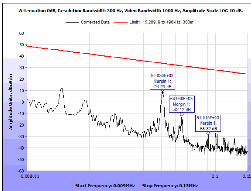
Plot 14. Spurious Emissions, Outside the Bands 13.110 - 14.010 MHz, 9 kHz – 150 kHz, 90°
