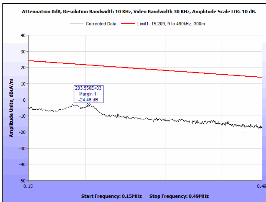
Plot 16. Spurious Emissions, Outside the Bands 13.110 - 14.010 MHz, 150 kHz – 490 kHz, 90°
