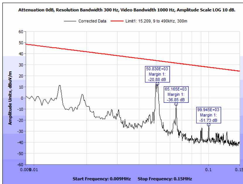
Plot 13. Spurious Emissions, Outside the Bands 13.110 - 14.010 MHz, 9 kHz – 150 kHz, 0°
