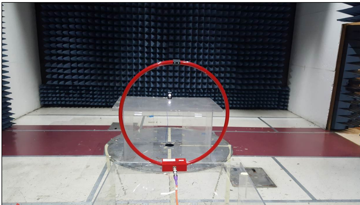
Photograph 3. Spurious Emissions, Test Setup, 150 kHz – 30 MHz
