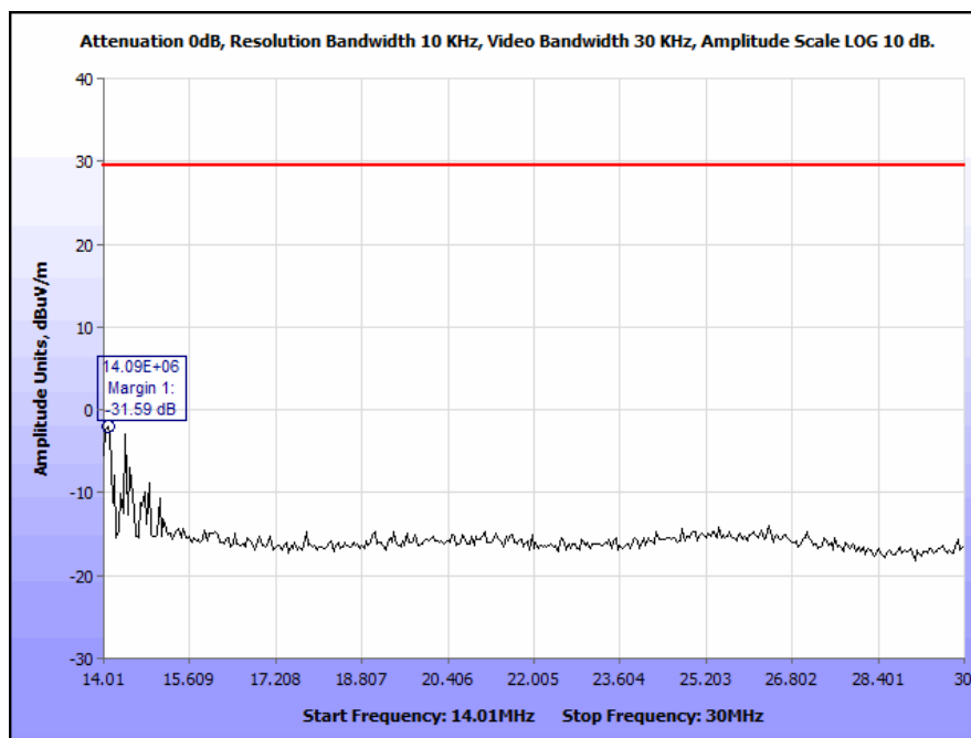
Plot 21. Spurious Emissions, Outside the Bands 13.110 - 14.010 MHz, 14.01 MHz – 30 MHz, 0°
