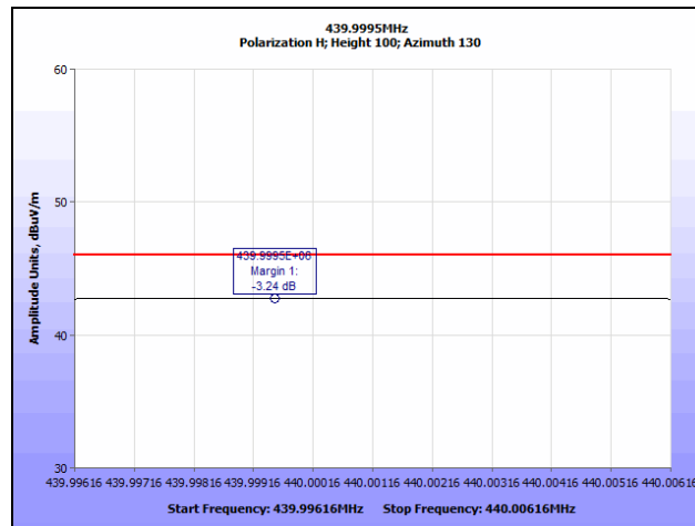
Plot 19. Radiated Spurious Emissions, Low Channel, 439.9995 MHz QP
