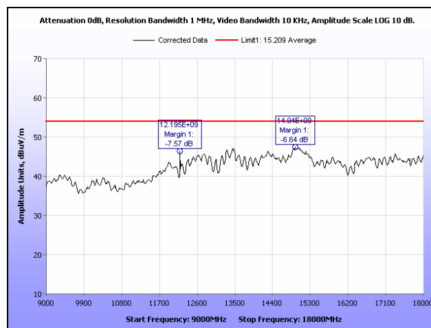
Plot 123. Radiated Spurious Emissions, Mid Channel, 9 GHz – 18 GHz, Average
