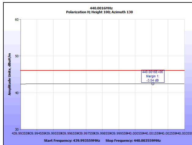
Plot 20. Radiated Spurious Emissions, Mid Channel, 440.0016 MHz QP
