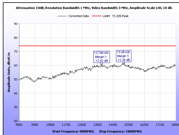
Plot 154. Radiated Spurious Emissions, High Channel, 9 GHz – 18 GHz, Peak
