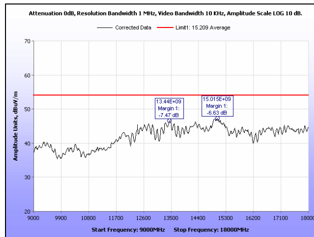
Plot 14. Radiated Spurious Emissions, High Channel, 9 GHz – 18 GHz, Average
