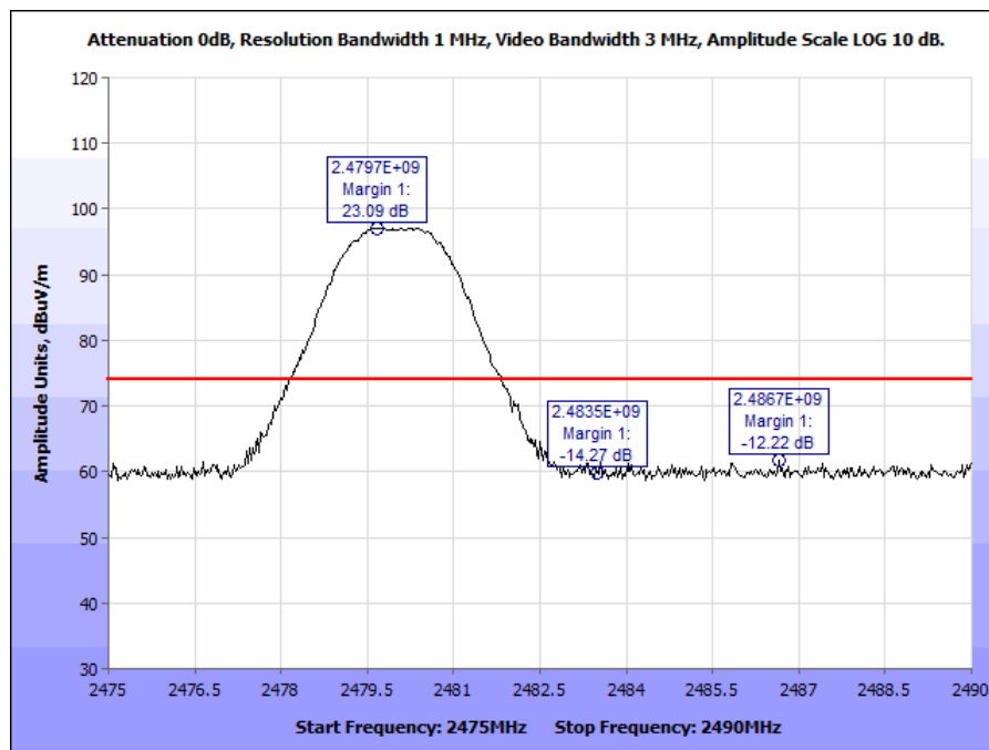
Plot 10. Radiated Restricted Band Edge, High Channel, 2483.5 MHz, Peak
