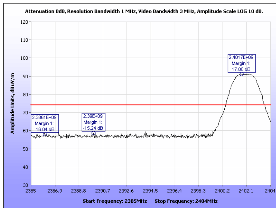
Plot31. Radiated Restricted Band Edge, Low Channel, 2390 MHz, Peak
