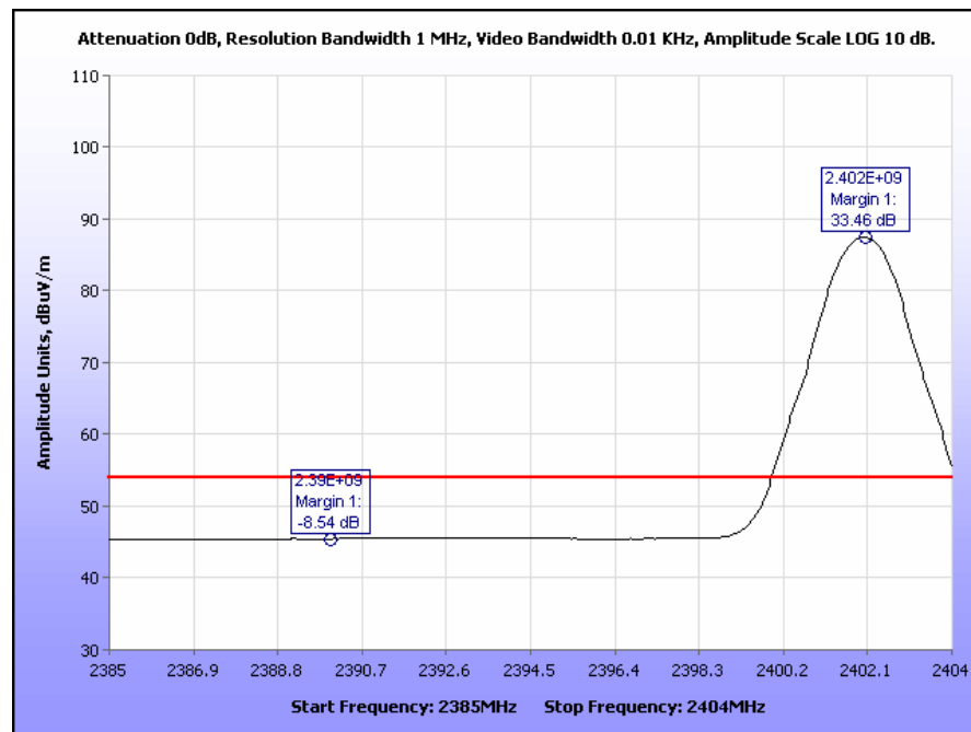
Plot 30. Radiated Restricted Band Edge, Low Channel, 2390 MHz, Average
