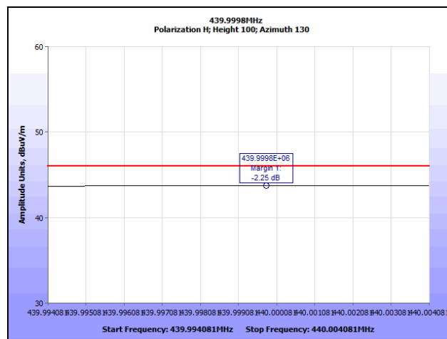
Plot 21. Radiated Spurious Emissions, High Channel, 439.9998 MHz QP
