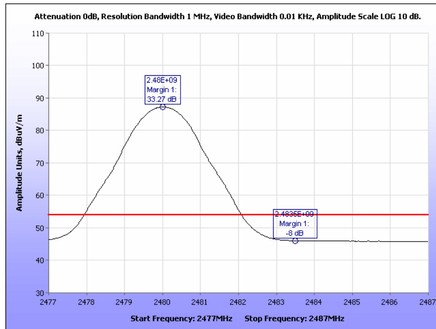
Plot 32. Radiated Restricted Band Edge, High Channel, 2483.5 MHz, Average
