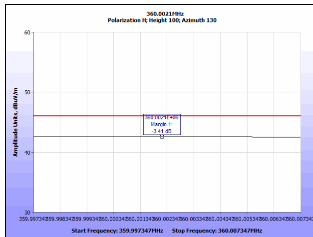
Plot 18. Radiated Spurious Emissions, High Channel, 360.0021 MHz QP
