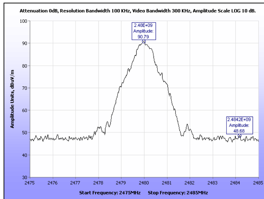
Plot 29. Radiated Restricted Band Edge, High Channel, 20 dBc, 2483.5 MHz
