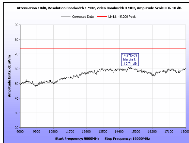
Plot 11. Radiated Spurious Emissions, Low Channel, 9 GHz – 18 GHz, Peak
