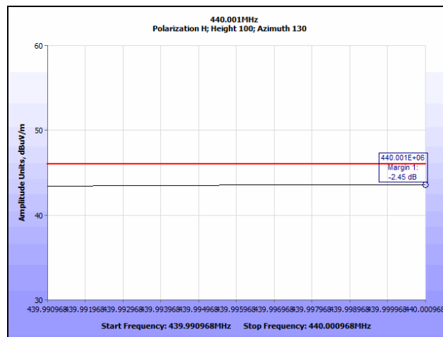
Plot 19. Radiated Spurious Emissions, Low Channel, 440.001 MHz QP
