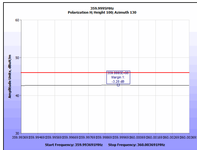
Plot 17. Radiated Spurious Emissions, Mid Channel, 359.9995 MHz QP
