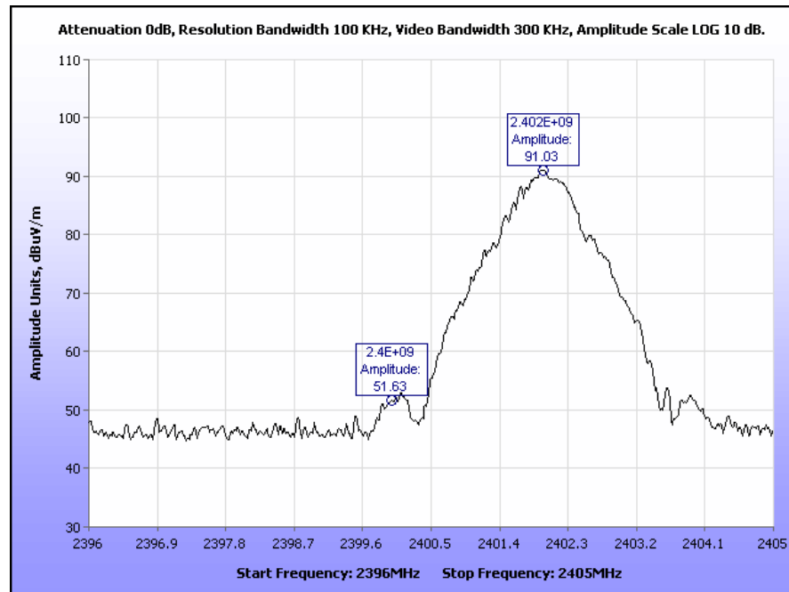
Plot 28. Radiated Restricted Band Edge, Low Channel, 20 dBc, 2400 MHz
