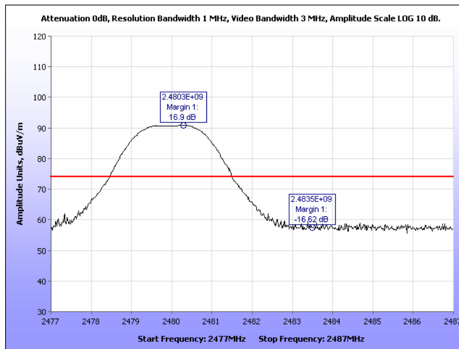
Plot 33. Radiated Restricted Band Edge, High Channel, 2483.5 MHz, Peak
