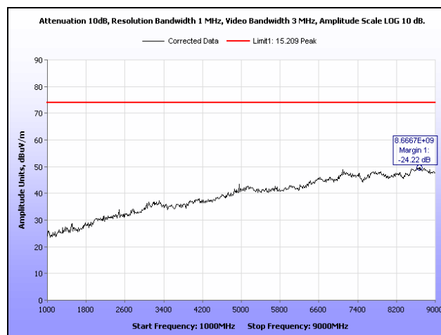
Plot 9. Radiated Spurious Emissions, High Channel, 1 GHz – 9 GHz, Peak
