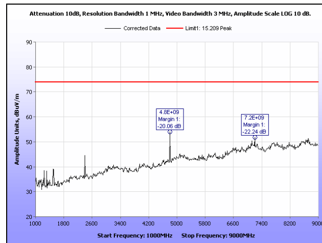
Plot 5. Radiated Spurious Emissions, Low Channel, 1 GHz – 9 GHz, Peak
