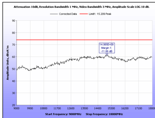
Plot 15. Radiated Spurious Emissions, Mid Channel, 9 GHz – 18 GHz, Peak
