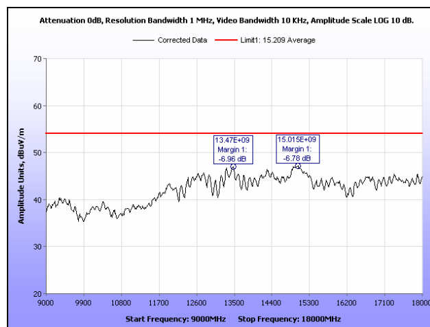
Plot 14. Radiated Spurious Emissions, Mid Channel, 9 GHz – 18 GHz, Average
