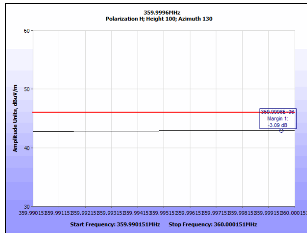
Plot 18. Radiated Spurious Emissions, Low Channel, 359.996 MHz QP
