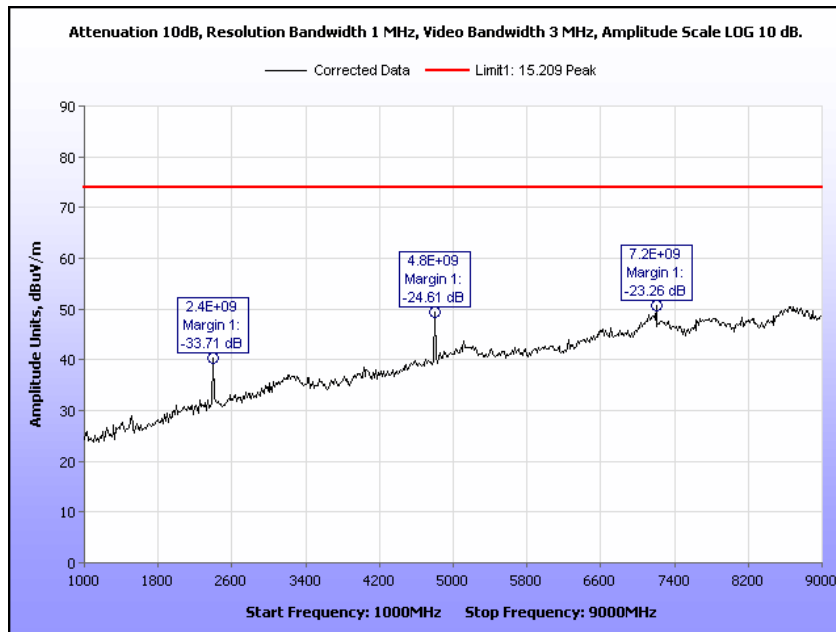
Plot 26. Radiated Spurious Emissions, All Tx Active, 1-9GHz Peak
