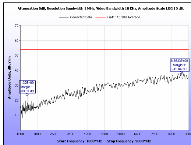
Plot 10. Radiated Spurious Emissions, High Channel, 1 GHz – 9 GHz, Average
