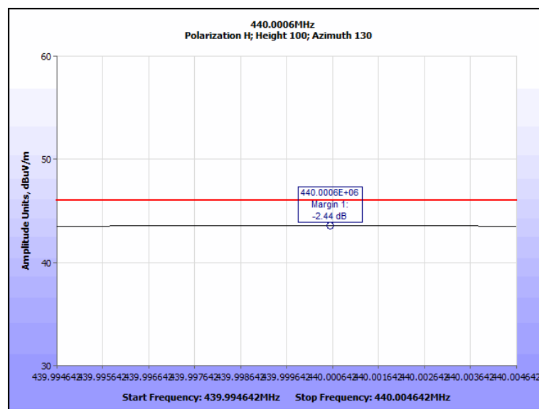
Plot 29. Radiated Spurious Emissions, All Tx Active, 440 MHz QP
