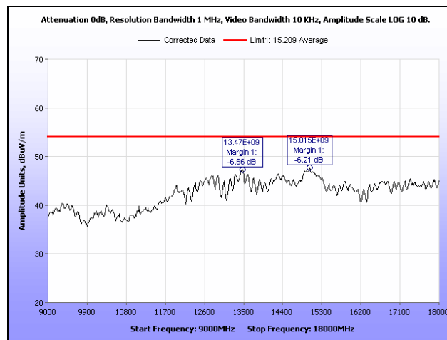
Plot 12. Radiated Spurious Emissions, Low Channel, 9 GHz – 18 GHz, Average
