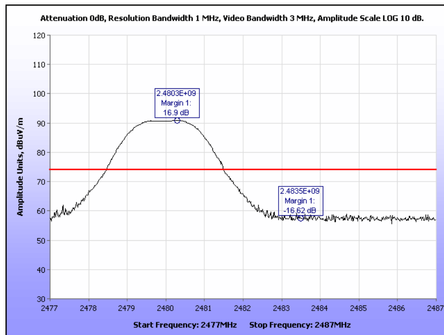
Plot 36. Radiated Restricted Band Edge, High Channel, 2483.5 MHz, Peak
