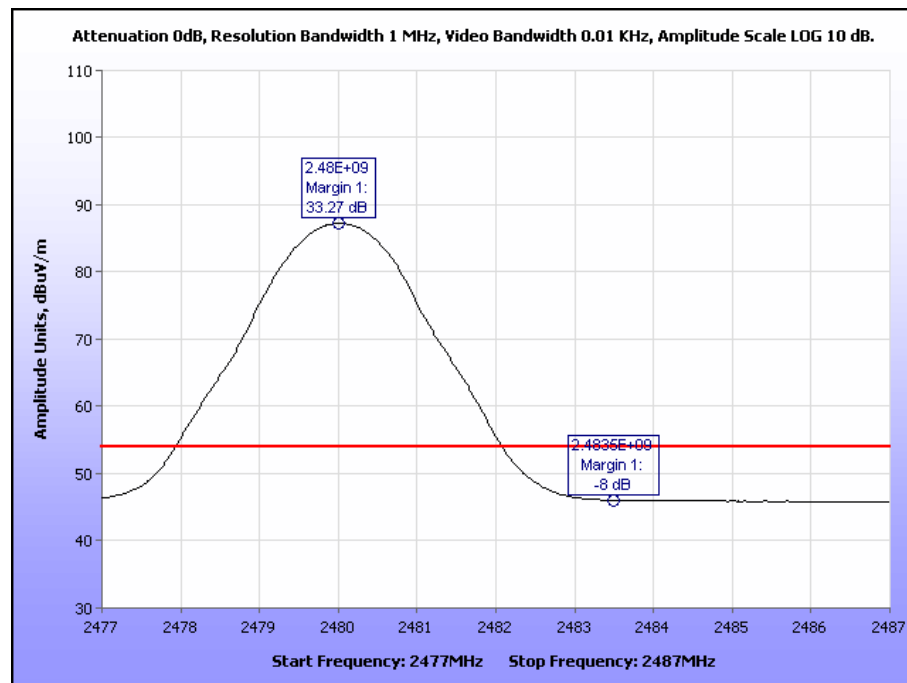
Plot 35. Radiated Restricted Band Edge, High Channel, 2483.5 MHz, Average
