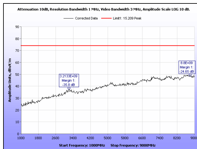
Plot 11. Radiated Spurious Emissions, High Channel, 1 GHz – 9 GHz, Peak
