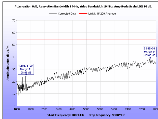
Plot 6. Radiated Spurious Emissions, Low Channel, 1 GHz – 9 GHz, Average
