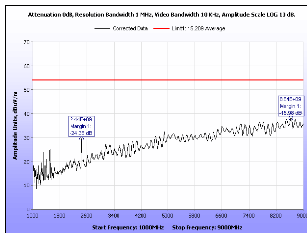
Plot 8. Radiated Spurious Emissions, Mid Channel, 1 GHz – 9 GHz, Average
