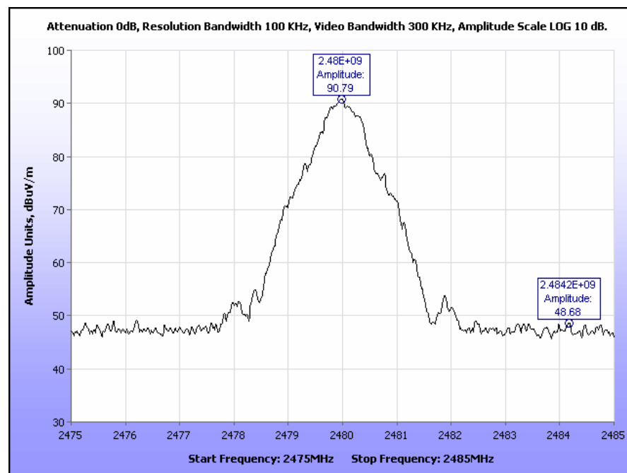
Plot 32. Radiated Restricted Band Edge, High Channel, 20 dBc, 2483.5 MHz
