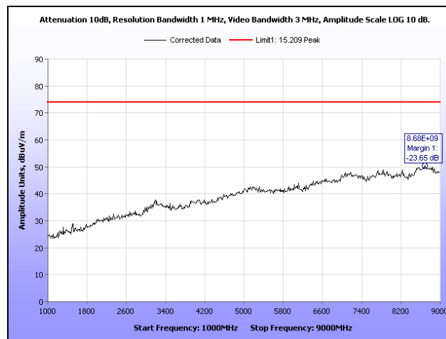
Plot 9. Radiated Spurious Emissions, Mid Channel, 1 GHz – 9 GHz, Peak
