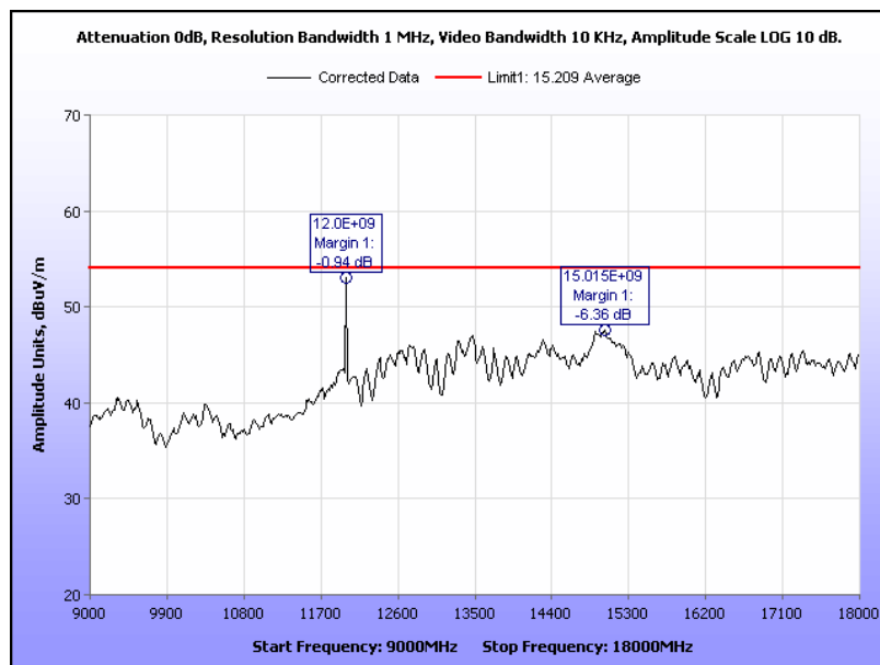
Plot 27. Radiated Spurious Emissions, All Tx Active, 9-18GHz Average
