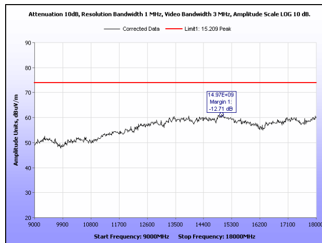
Plot 13. Radiated Spurious Emissions, Low Channel, 9 GHz – 18 GHz, Peak
