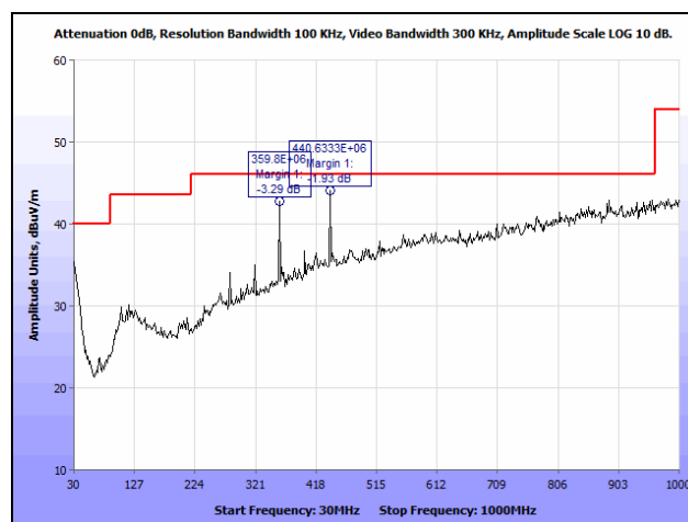
Plot 5. Radiated Spurious Emissions, High Channel, 30 MHz – 1 GHz
