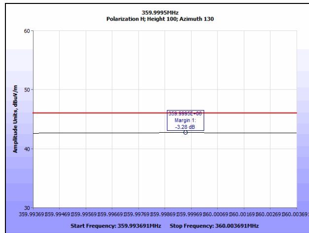
Plot 19. Radiated Spurious Emissions, Mid Channel, 359.995 MHz QP
