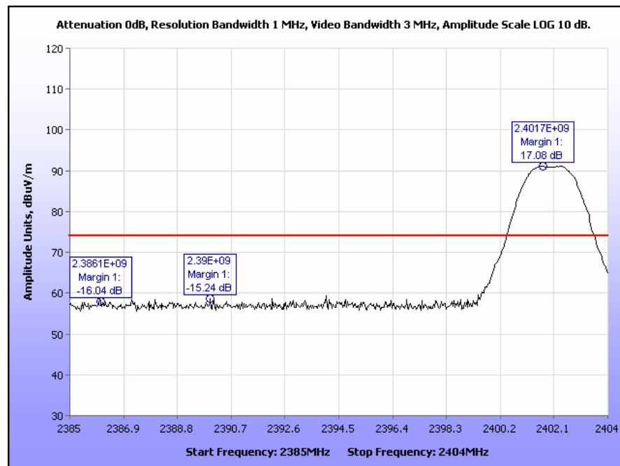
Plot 34. Radiated Restricted Band Edge, Low Channel, 2390 MHz, Peak
