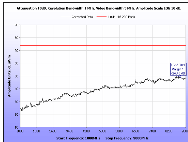
Plot 7. Radiated Spurious Emissions, Low Channel, 1 GHz – 9 GHz, Peak
