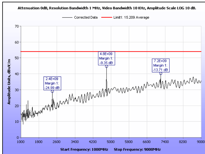
Plot 25. Radiated Spurious Emissions, All Tx Active, 1-9GHz Average
