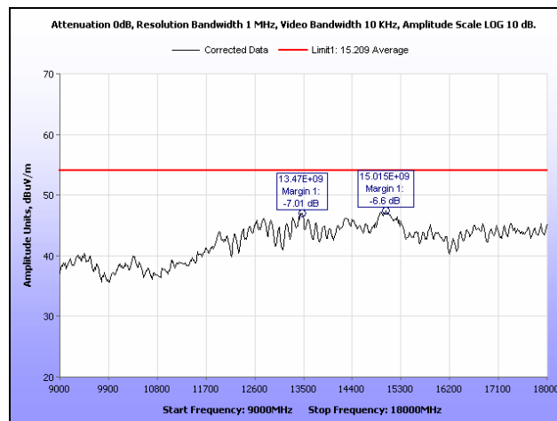
Plot 16. Radiated Spurious Emissions, High Channel, 9 GHz – 18 GHz, Average
