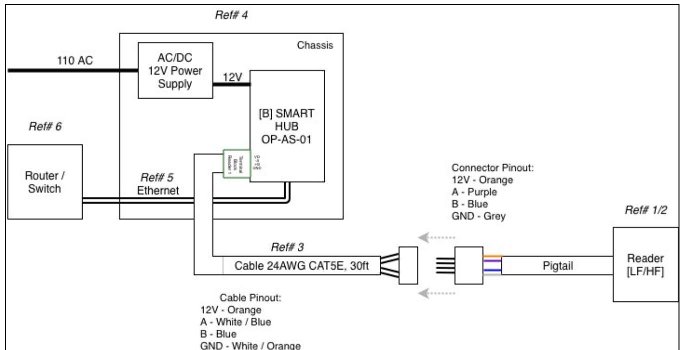
Figure 1. Block Diagram of Test Configuration, Standard Smart Reader (LF)
