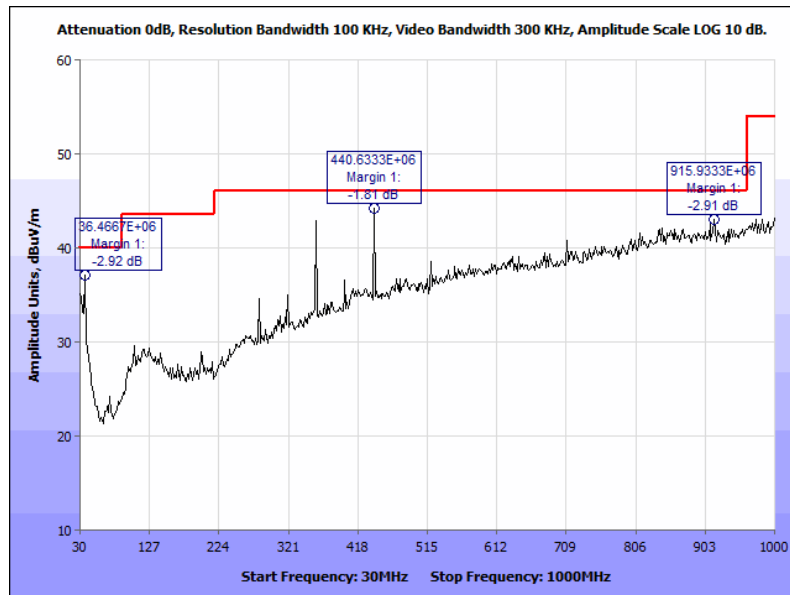
Plot 24. Radiated Spurious Emissions, All Tx Active, 30-1000MHz
