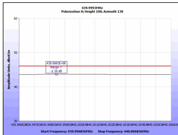
Plot 22. Radiated Spurious Emissions, Mid Channel, 439.9993 MHz QP
