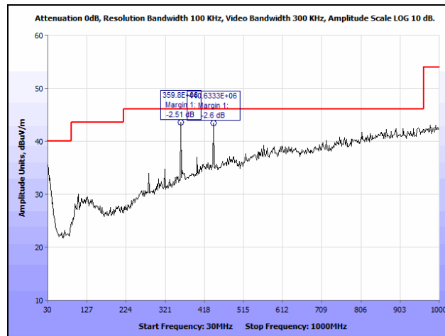
Plot 3. Radiated Spurious Emissions, Low Channel, 30 MHz – 1 GHz
