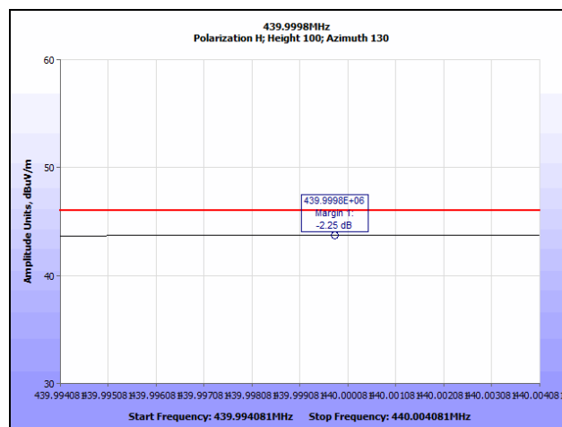
Plot 23. Radiated Spurious Emissions, High Channel, 439.9998 MHz QP
