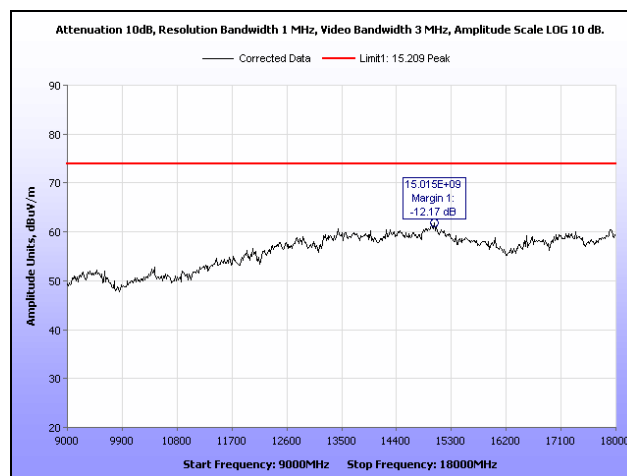
Plot 17. Radiated Spurious Emissions, High Channel, 9 GHz – 18 GHz, Peak
