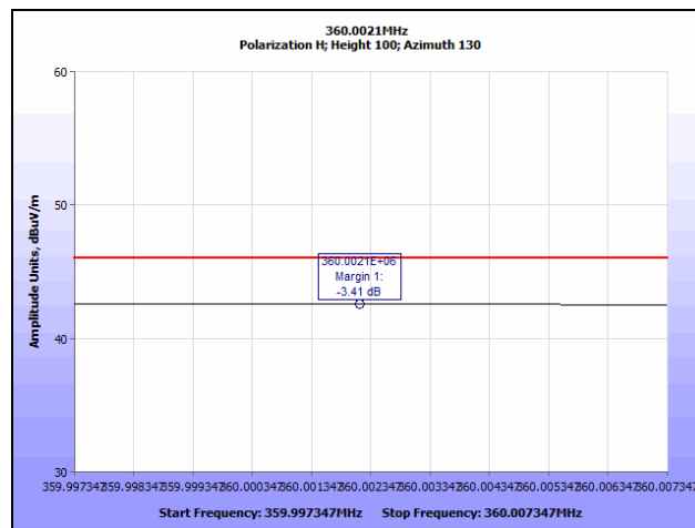
Plot 20. Radiated Spurious Emissions, High Channel, 360.0021 MHz QP
