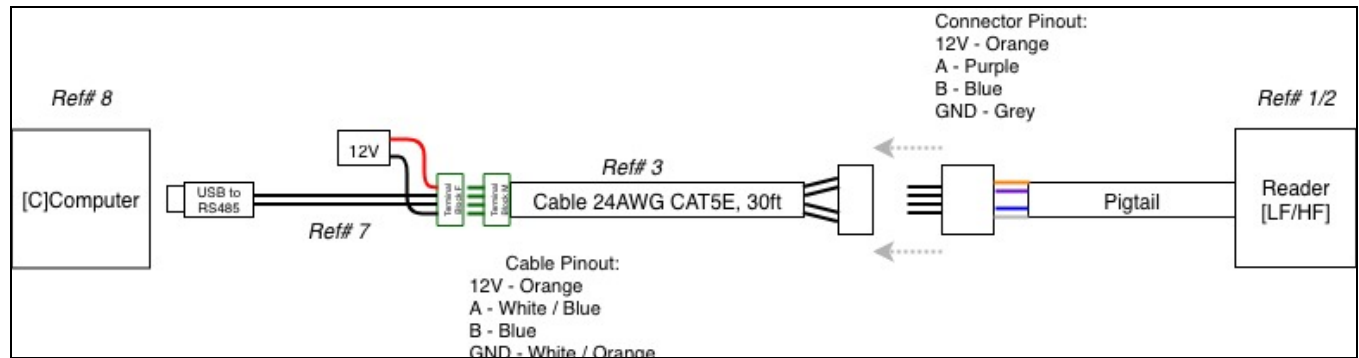
Figure 2. Block Diagram of Test Configuration, Mullion Smart Reader (LF)
