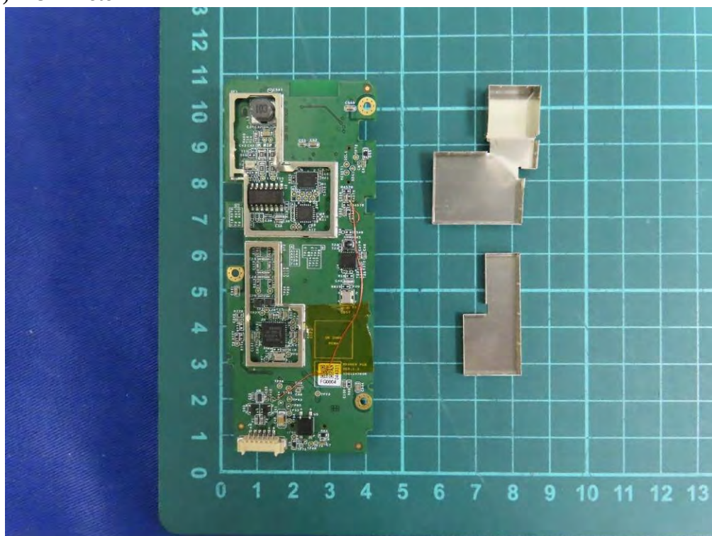
(26) EUT Photo
