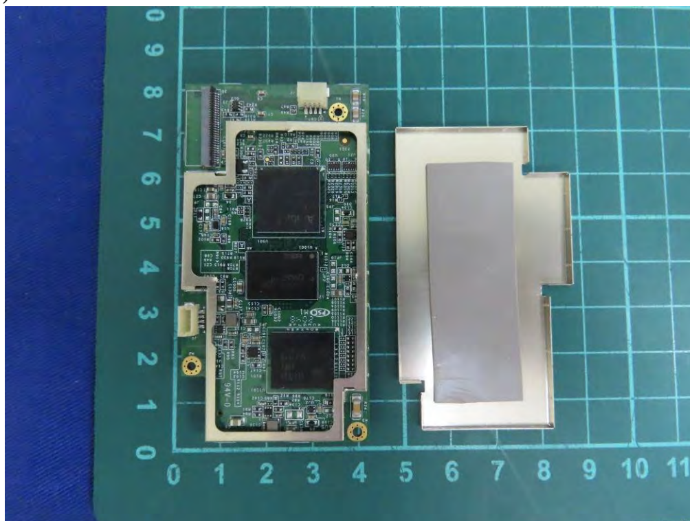
(55) EUT Photo
