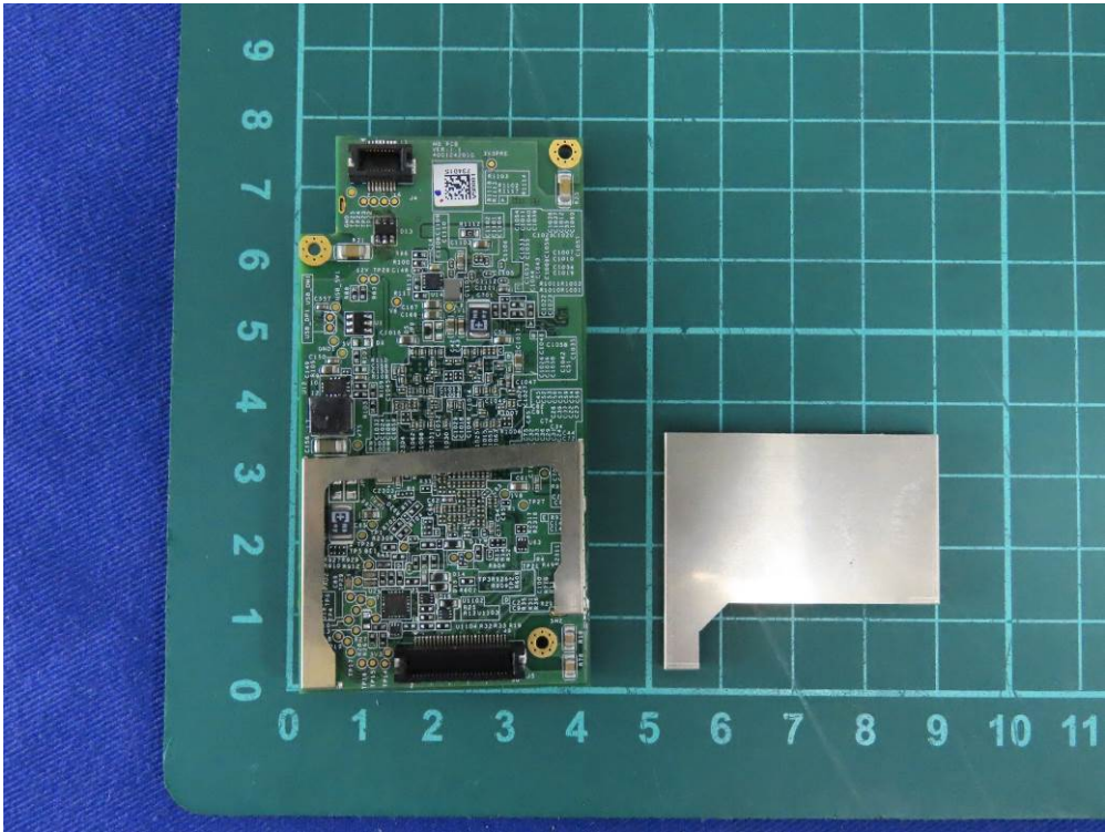
(45) EUT Photo
