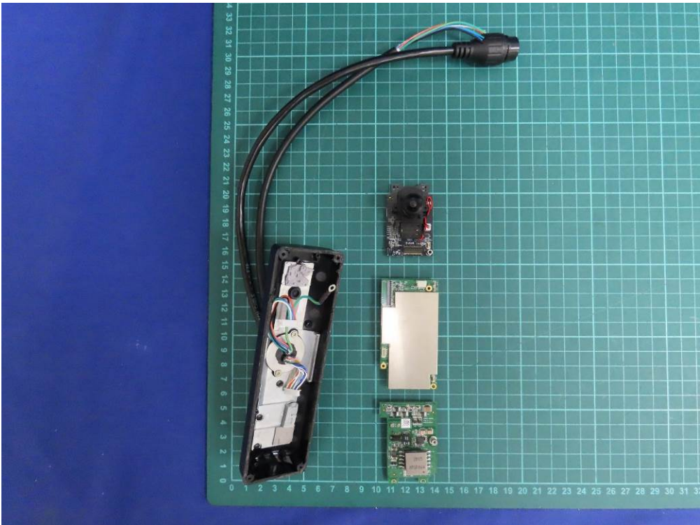
(34) EUT Photo
