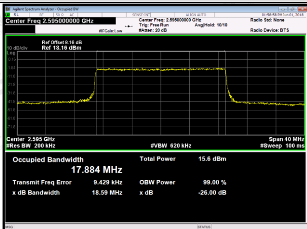
MCH_QPSK_100RB#0
