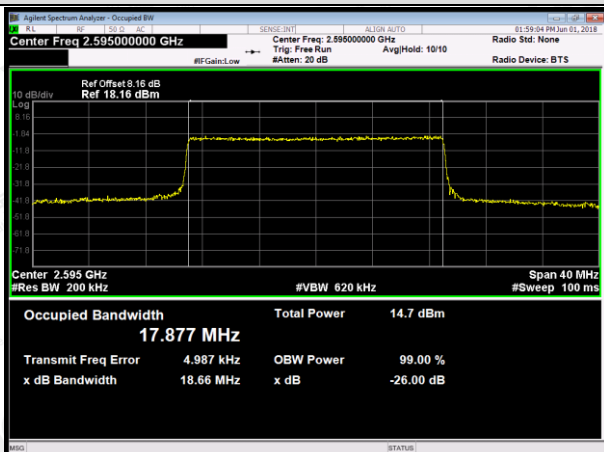
MCH_16QAM_100RB#0
