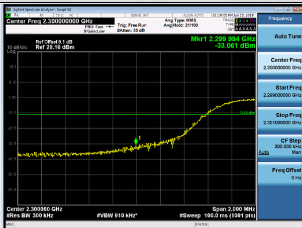
LCH_16QAM_75RB#0
