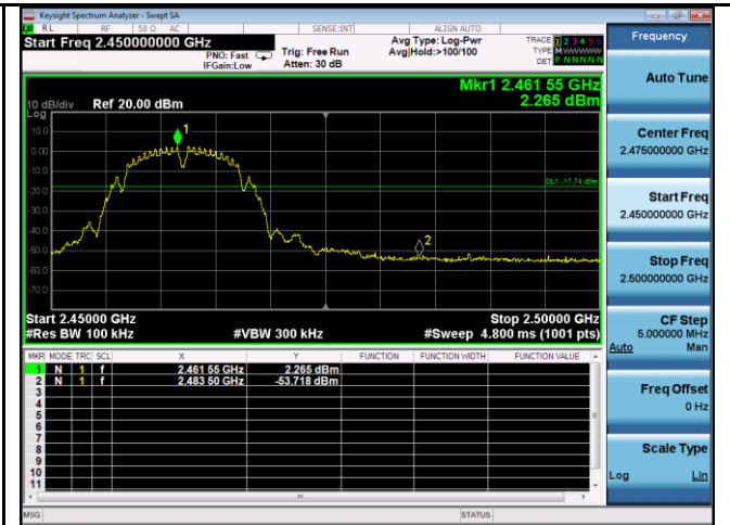
Band Edge, Right Side - 802.11b
