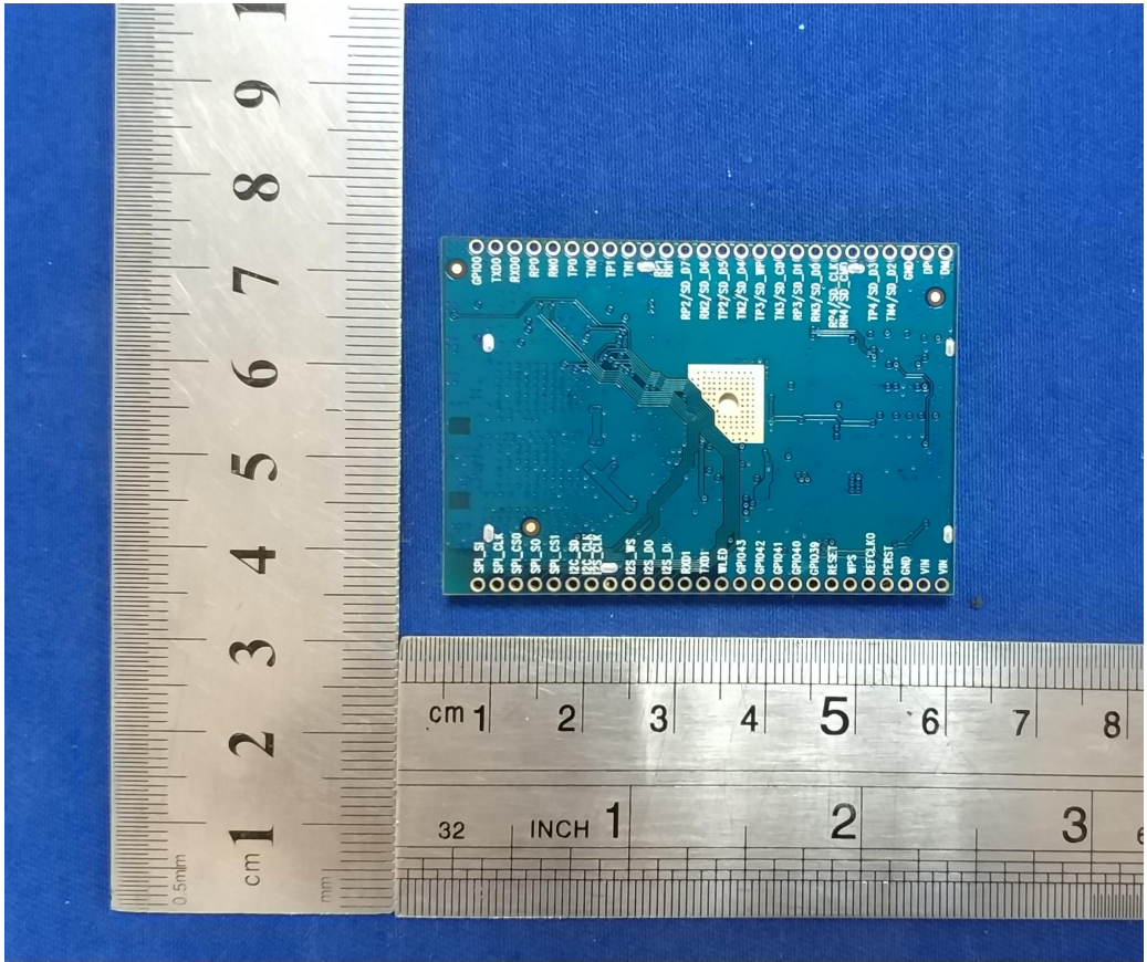
EUT - PCB View
