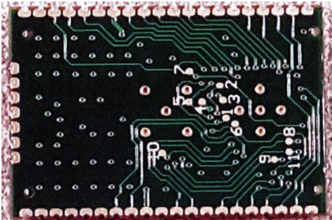
Microchip RN2903A with shield open back side
