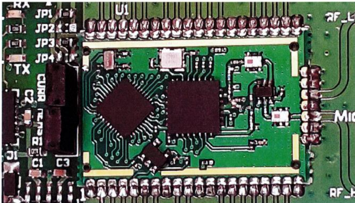
Microchip RN2903A with shield open front side
