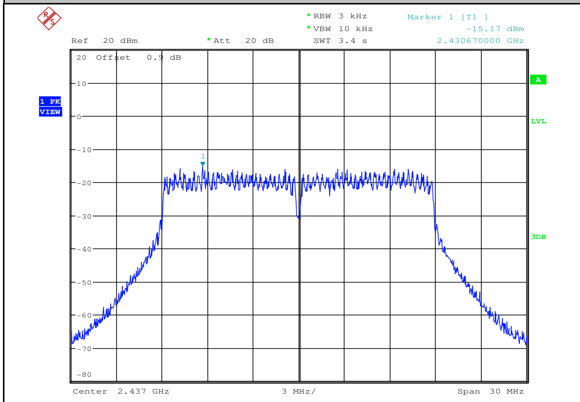
Maximum Peak power spectral density_11N20SISO_2437_Ant2
