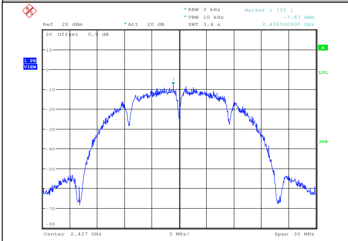
Maximum Peak power spectral density_11B_2437_Ant2
