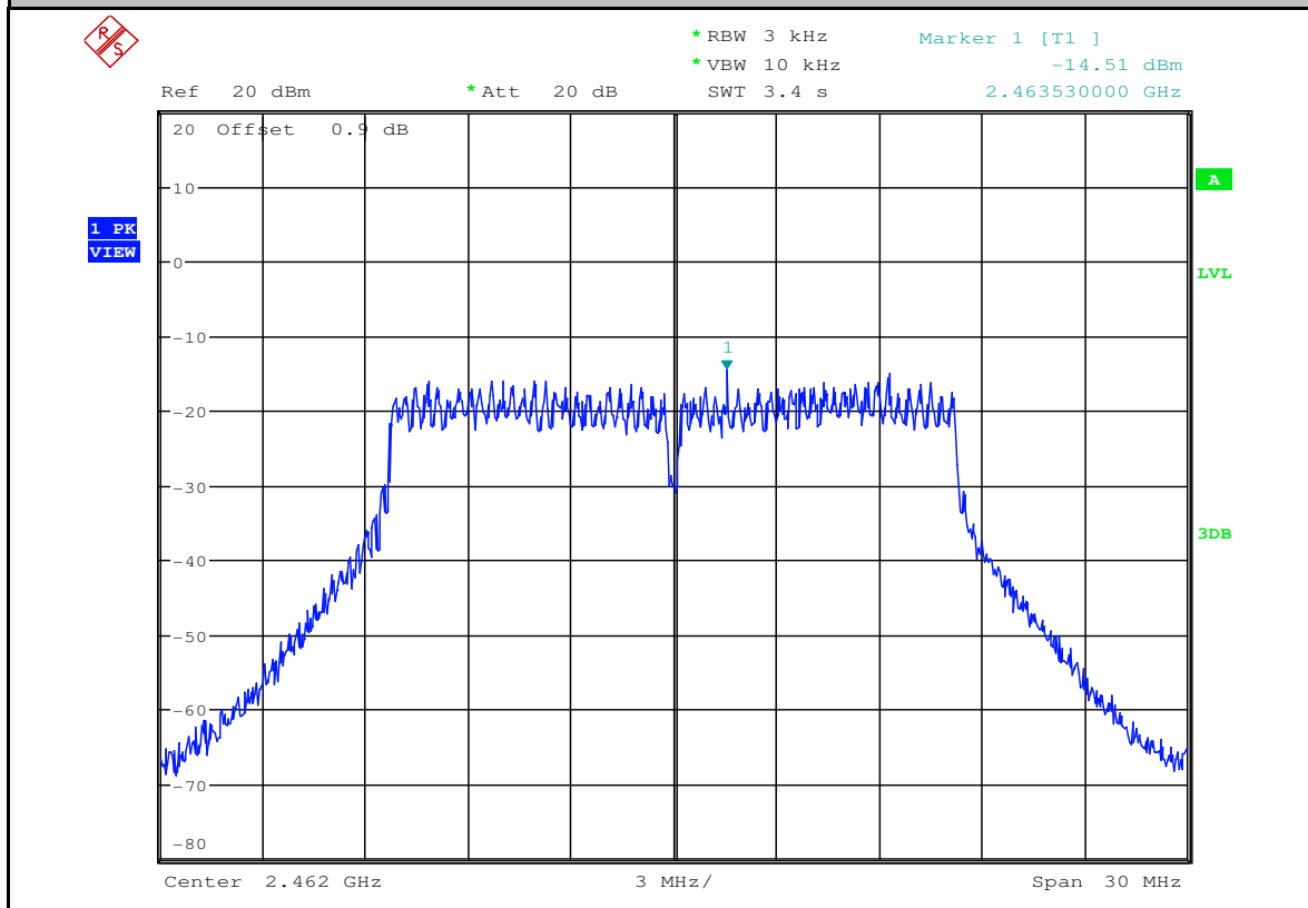
Maximum Peak power spectral density_11G_2462_Ant2
