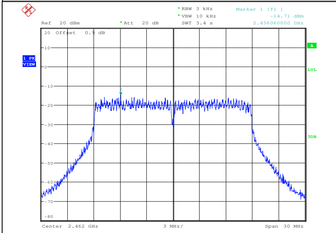
Maximum Peak power spectral density_11N20SISO_2462_Ant2
