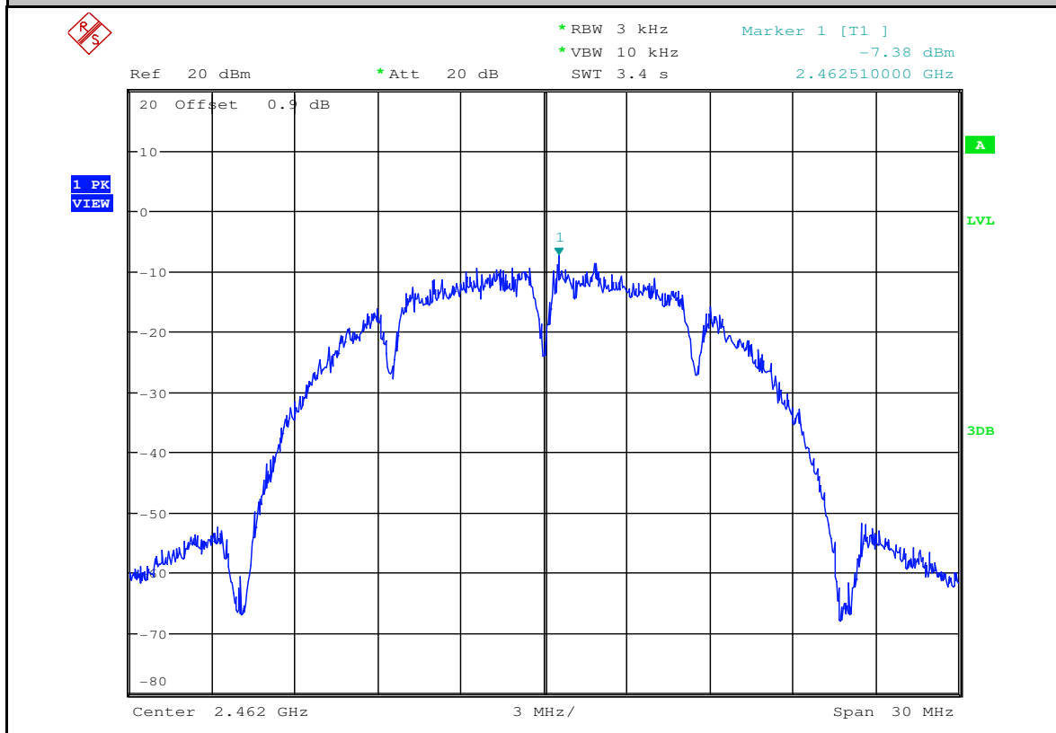
Maximum Peak power spectral density_11B_2462_Ant2
