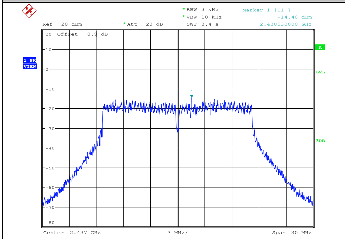
Maximum Peak power spectral density_11G_2437_Ant2
