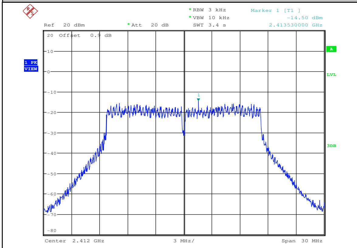
Maximum Peak power spectral density_11G_2412_Ant2
