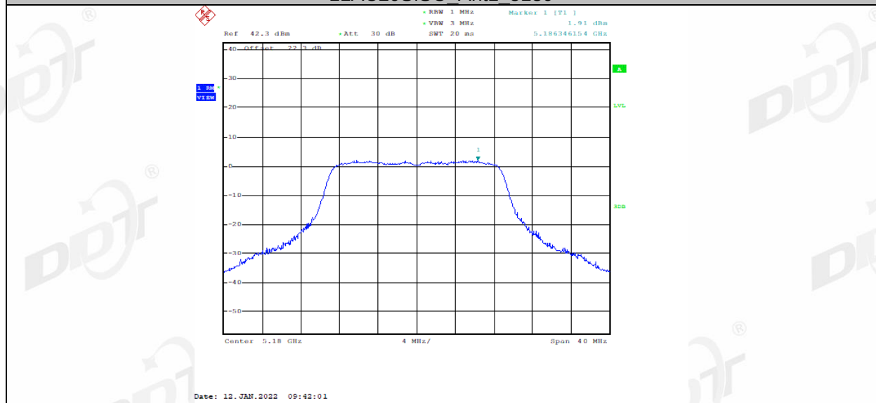
11AC20SISO_Ant1_5200
