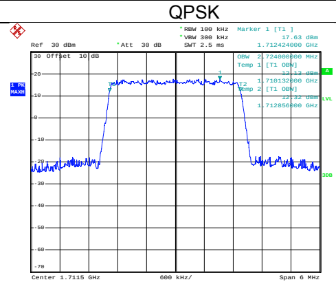
LTE Band 4: 99% Occupy bandwidth BW: 3MHz
