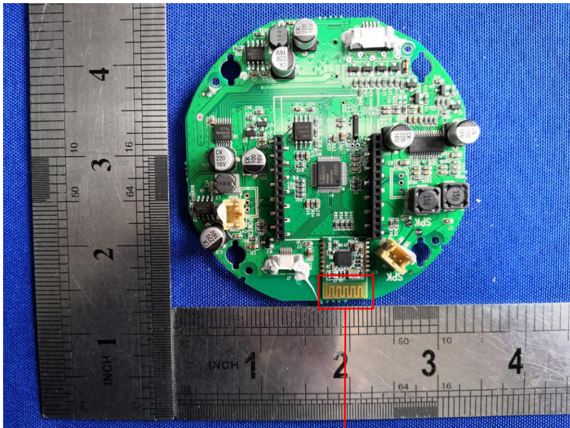
BT PCB ANT
