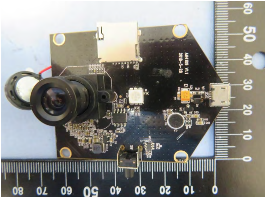
WLAN Antenna
