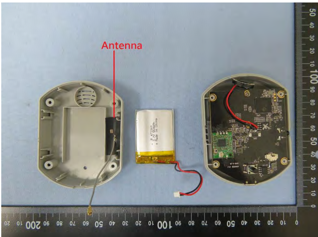
WLAN Antenna
