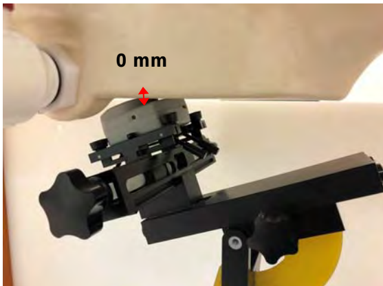
Fig.9 EUT Front 1 to 2 tilt side to flat phantom
