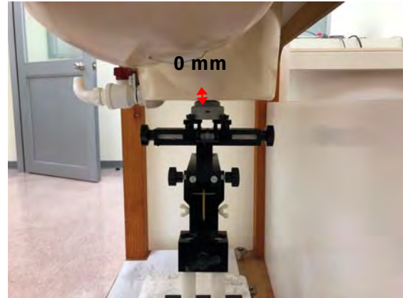
Fig.4 EUT Front 1 side to flat phantom
