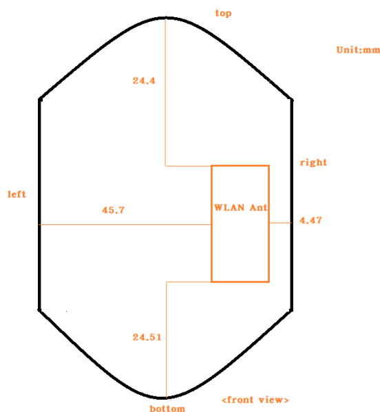
Fig.12 Antenna position of EUT
