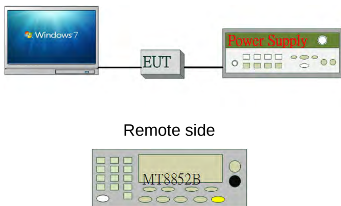
Fig. 2-1 Radiated Emission
