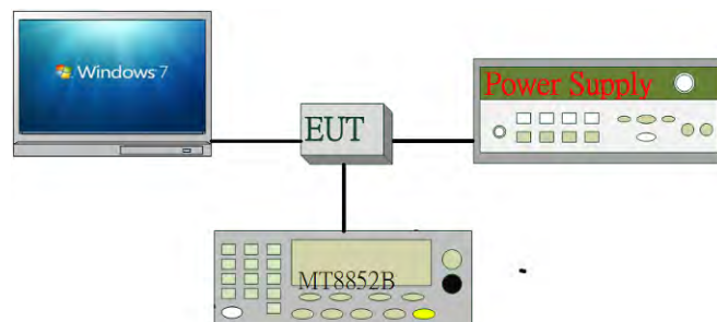
Fig. 2-2 Conducted (Antenna Port) Configuration
