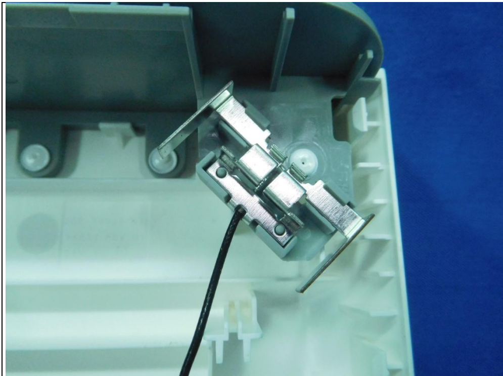
WLAN Antenna 1
