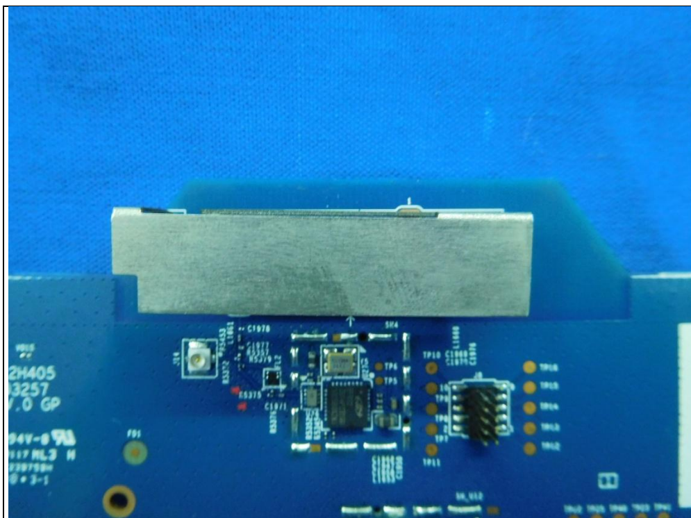
Sub-GHz Antenna
