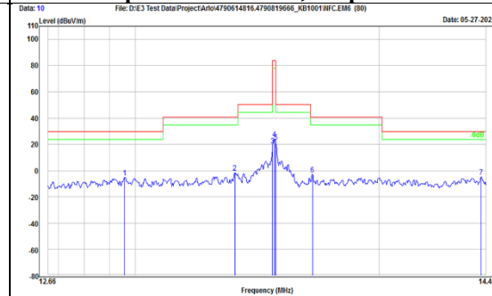
TX, Fundamental NFC-Type A (Ch 1) Radiated Spurious Emission, Perpendicular
