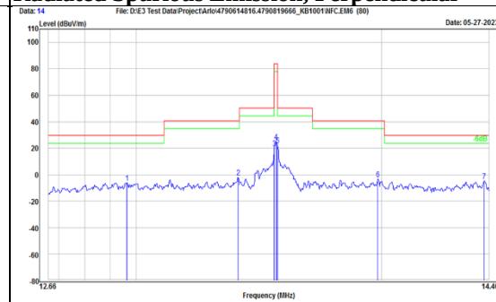
TX, Fundamental NFC-Type V (Ch 1) Radiated Spurious Emission, Perpendicular
