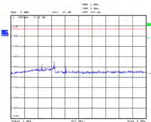
LTE Band 12 1.4MHz CH- Middle 1GHz~9GHz
