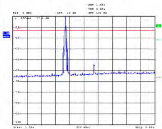
LTE Band 66 20MHz CH-Middle 1GHz~3GHz
