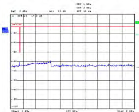
LTE Band 13 5MHz CH-Middle 1GHz~9GHz
