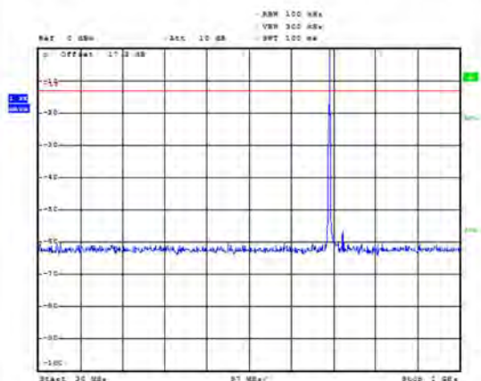
LTE Band 12 1.4MHz CH-Low 30MHz~1GHz
