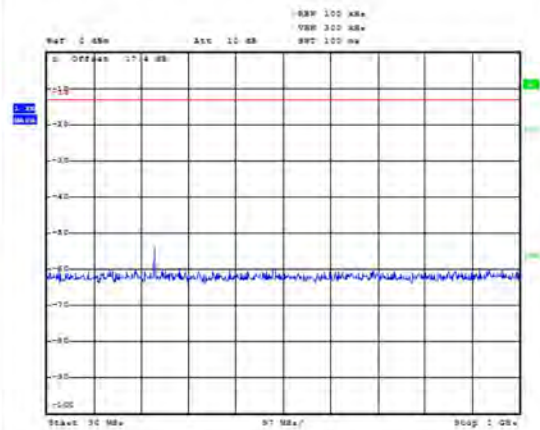
LTE Band 66 10MHz CH-Low 30MHz~1GHz
