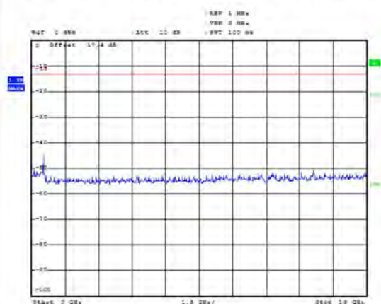
LTE Band 66 20MHz CH-High 3GHz~18GHz
