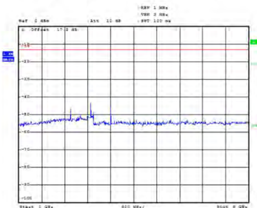
LTE Band 12 1.4MHz CH-Low 1GHz~9GHz
