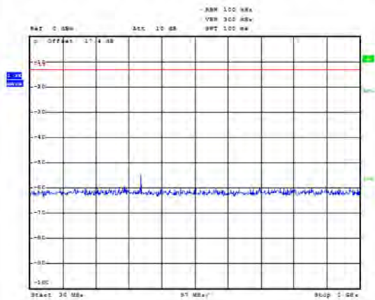
LTE Band 66 5MHz CH-High 30MHz~1GHz
