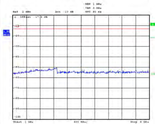
LTE Band 71 10MHz CH-Low 1GHz~9GHz
