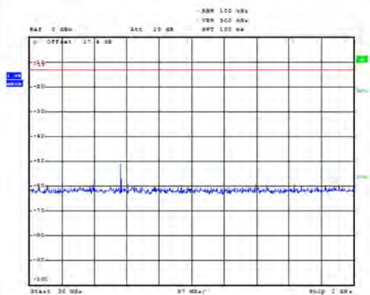
LTE Band 66 20MHz CH-Middle 30MHz~1GHz
