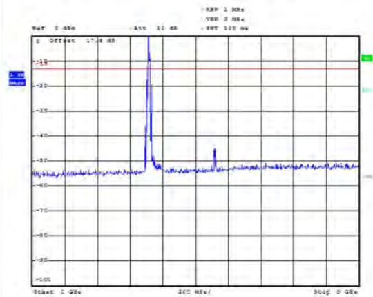
LTE Band 66 10MHz CH-Low 1GHz~3GHz
