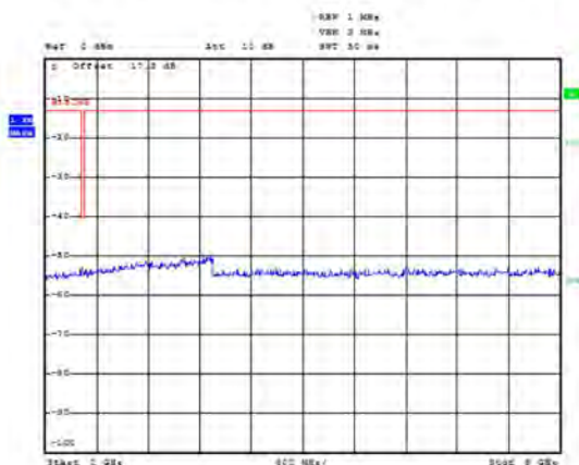
LTE Band 13 5MHz CH-High 1GHz~9GHz
