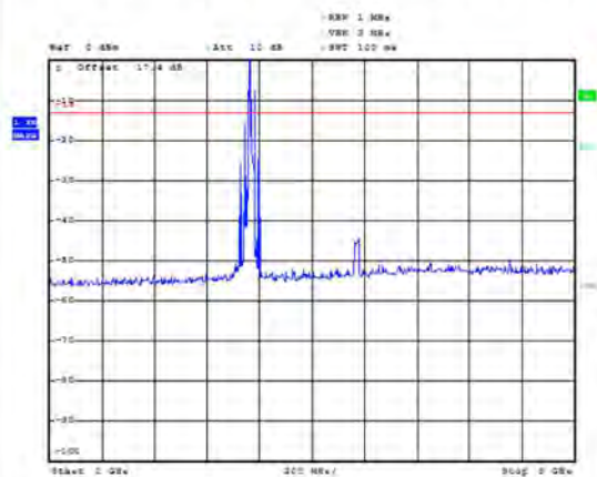
LTE Band 66 20MHz CH-High 1GHz~3GHz
