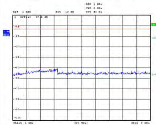
LTE Band 71 10MHz CH-Middle 1GHz~9GHz
