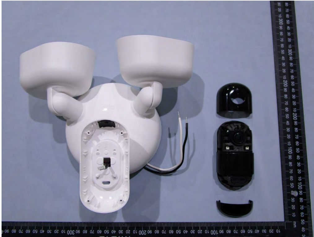
Internal Photos FLW2001 Pic 1
