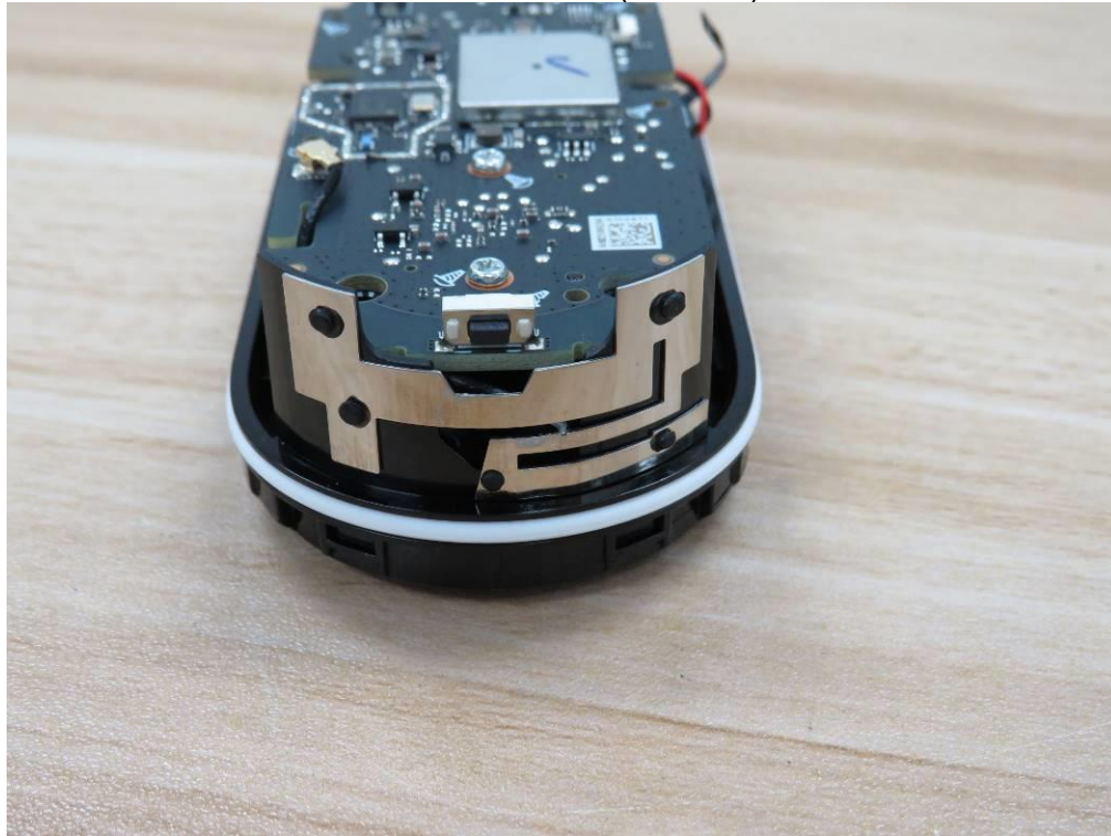
Internal View of EUT(Antenna)-13
