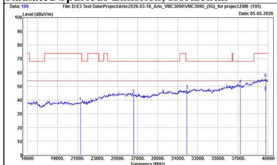
TX, 802.11a - Emission (Ch 64) Radiated Spurious Emission, Horizontal
