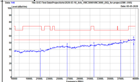
TX, 802.11a - Emission (Ch 60) Radiated Spurious Emission, Vertical
