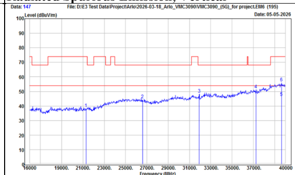
TX, 802.11a - Emission (Ch 64) Radiated Spurious Emission, Vertical
