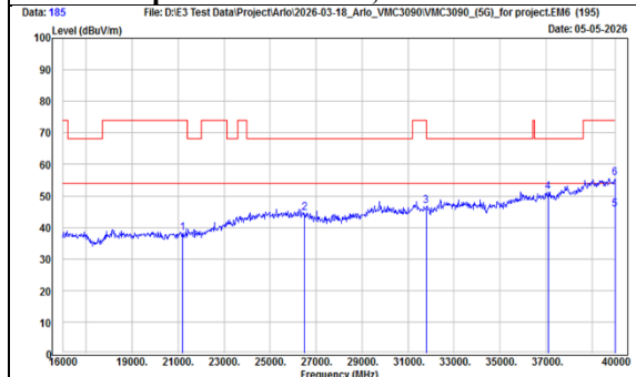
TX, 802.11a - Emission (Ch 60) Radiated Spurious Emission, Horizontal
