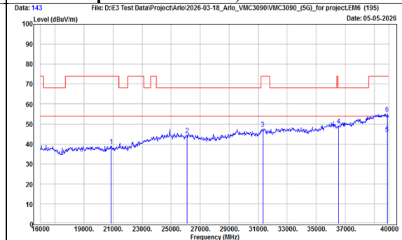
TX, 802.11a - Emission (Ch 44) Radiated Spurious Emission, Vertical
