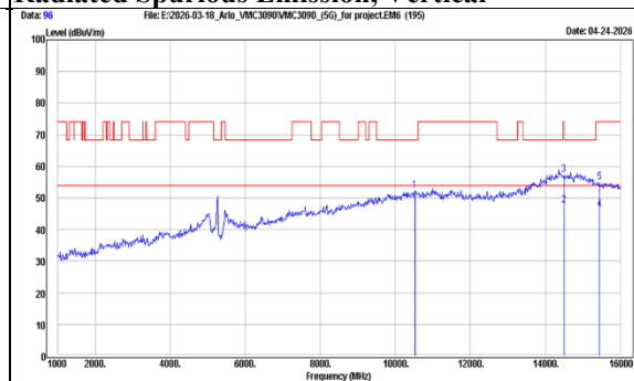
TX, 802.11a - Emission (Ch 52) Radiated Spurious Emission, Vertical
