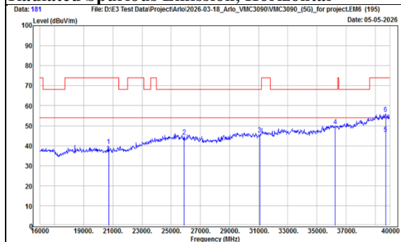
TX, 802.11a - Emission (Ch 36) Radiated Spurious Emission, Horizontal
