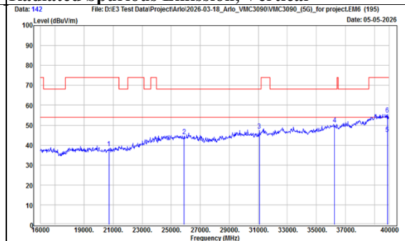
TX, 802.11a - Emission (Ch 36) Radiated Spurious Emission, Vertical
