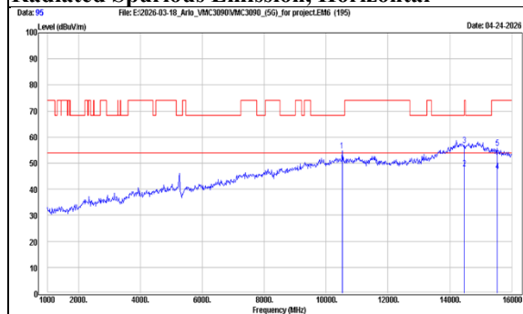
TX, 802.11a - Emission (Ch 52) Radiated Spurious Emission, Horizontal
