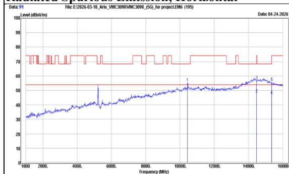
TX, 802.11a - Emission (Ch 44) Radiated Spurious Emission, Horizontal
