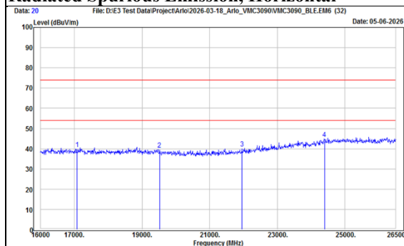
TX, BT-LE-1Mbps - Emission (Ch 19) Radiated Spurious Emission, Horizontal
