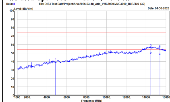
TX, BT-LE-1Mbps - Emission (Ch 19) Radiated Spurious Emission, Vertical
