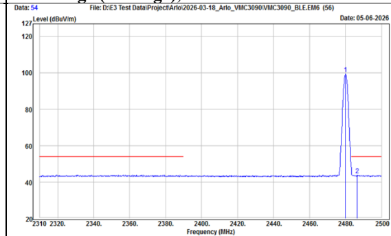
TX, BT-LE-2Mbps (Ch 39) Band Edge (Peak), Vertical
