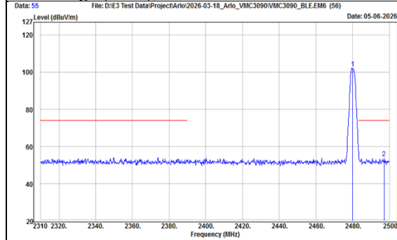
TX, BT-LE-2Mbps (Ch 39) Band Edge (Peak), Horizontal
