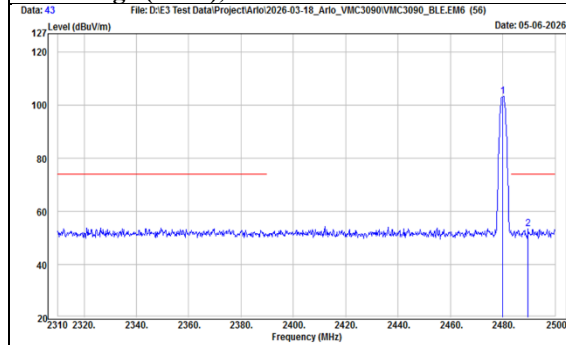
TX, BT-LE-1Mbps (Ch 39) Band Edge (Peak), Horizontal
