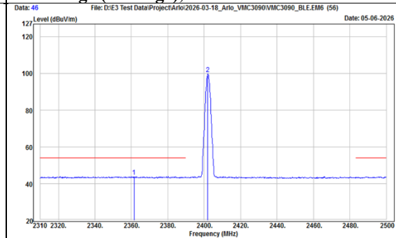
TX, BT-LE-2Mbps (Ch 0) Band Edge (Peak), Vertical
