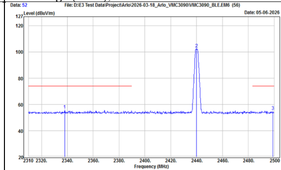
TX, BT-LE-2Mbps (Ch 19) Band Edge (Peak), Vertical
