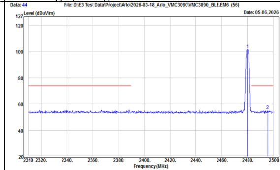
TX, BT-LE-1Mbps (Ch 39) Band Edge (Peak), Vertical
