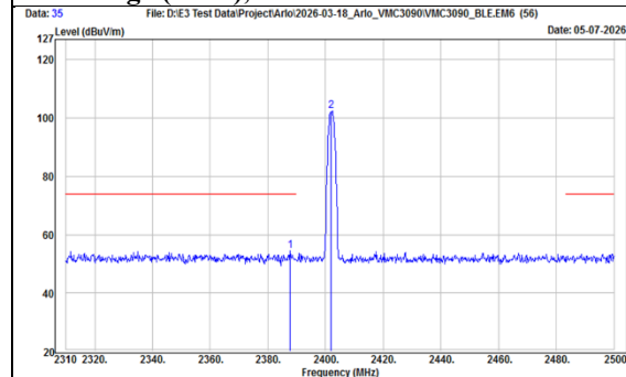
TX, BT-LE-1Mbps (Ch 0) Band Edge (Peak), Horizontal
