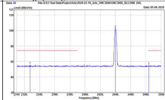
TX, BT-LE-1Mbps (Ch 19) Band Edge (Peak), Vertical
