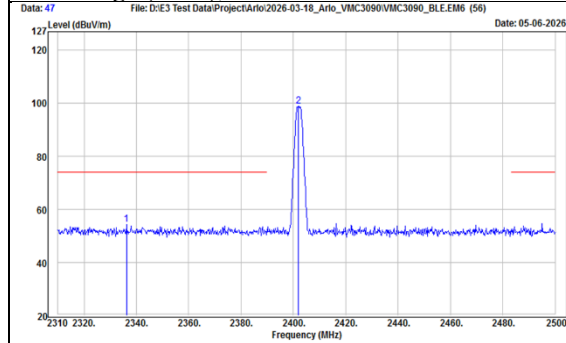
TX, BT-LE-2Mbps (Ch 0) Band Edge (Peak), Horizontal
