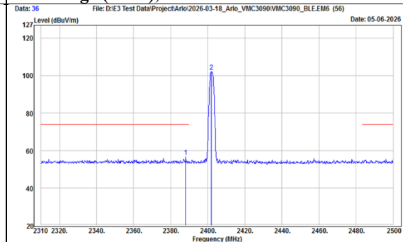
TX, BT-LE-1Mbps (Ch 0) Band Edge (Peak), Vertical
