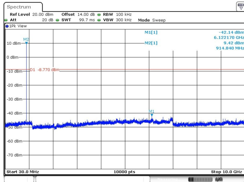
Conducted Spurious Emission Plot
