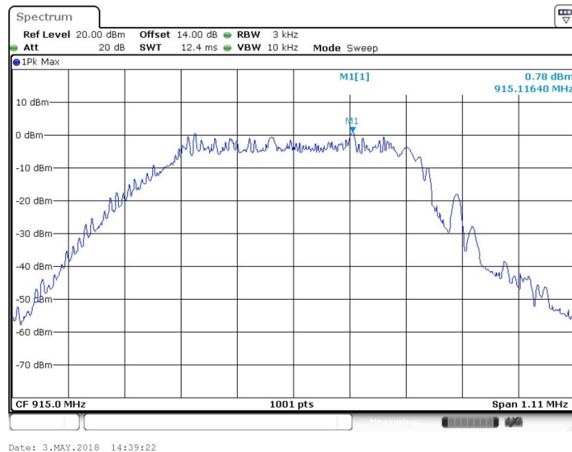
PSD 3kHz Plot
