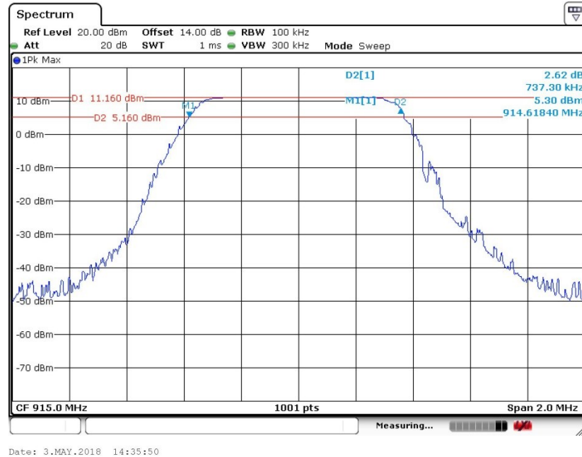
6 dB Bandwidth Plot
