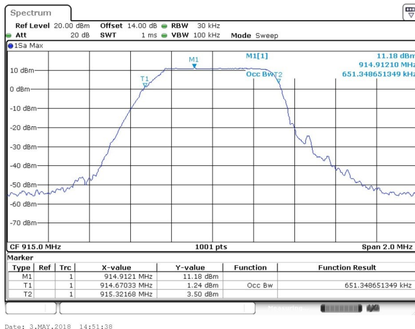
99% Bandwidth Plot
