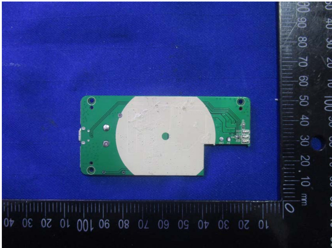
Coil Antenna
