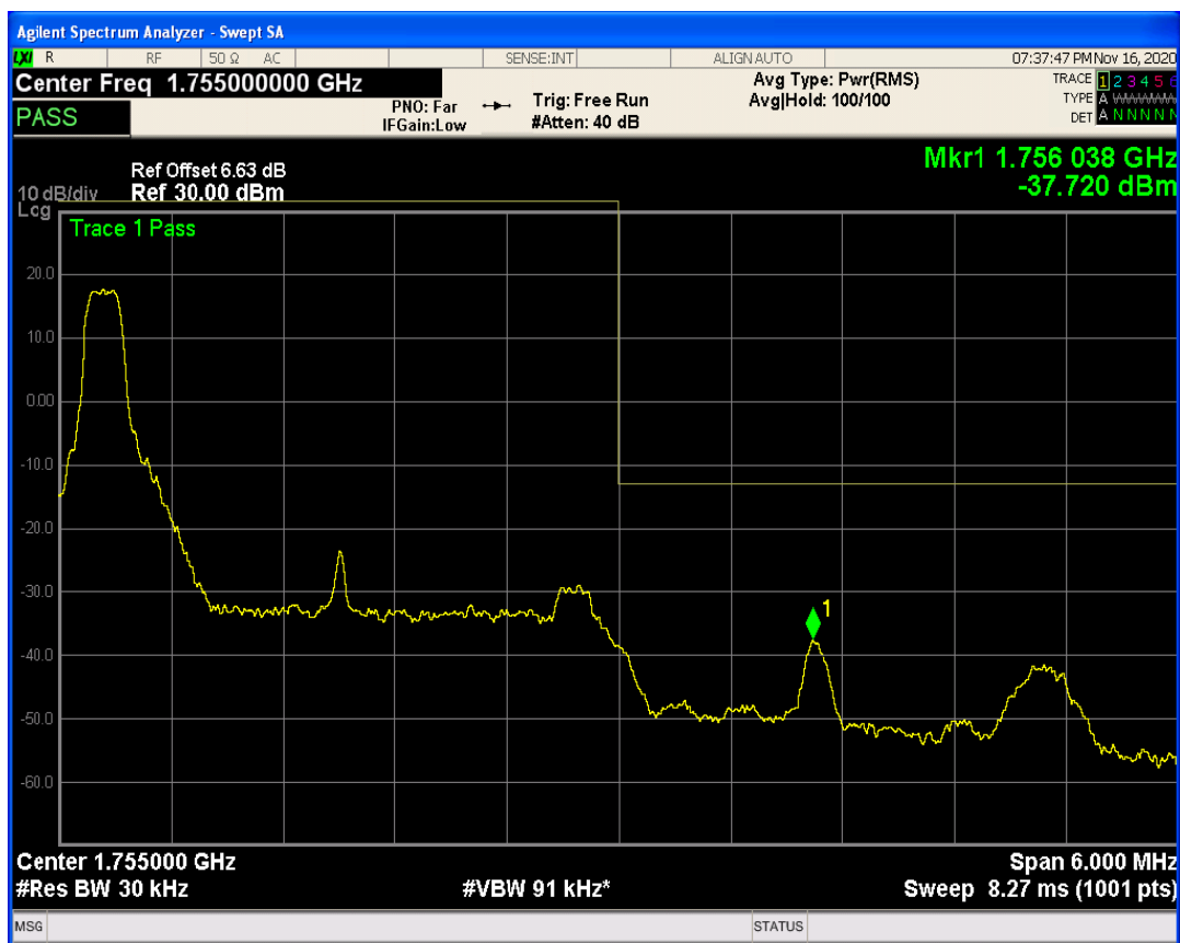
LTE Band4 QPSK BW=3MHz Channel=20385 RB Size=1 Position=#Max
