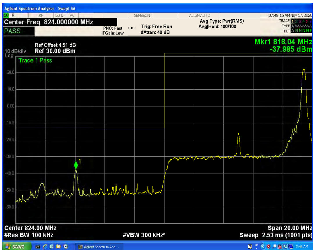
LTE Band5 QPSK BW=10MHz Channel=20450 RB Size=50 Position=#0
