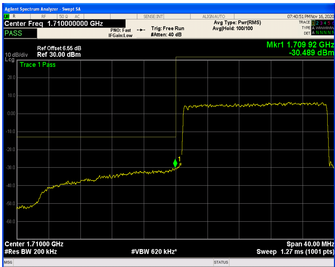
LTE Band4 QAM16 BW=20MHz Channel=20050 RB Size=1 Position=#Max
