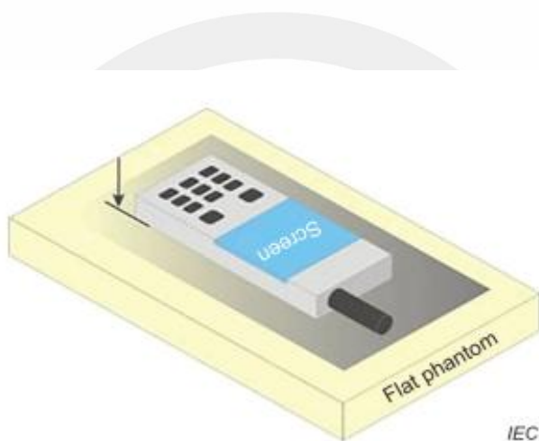
Fig-4.1 Test position for hand-held devices, not used at the head or torso
